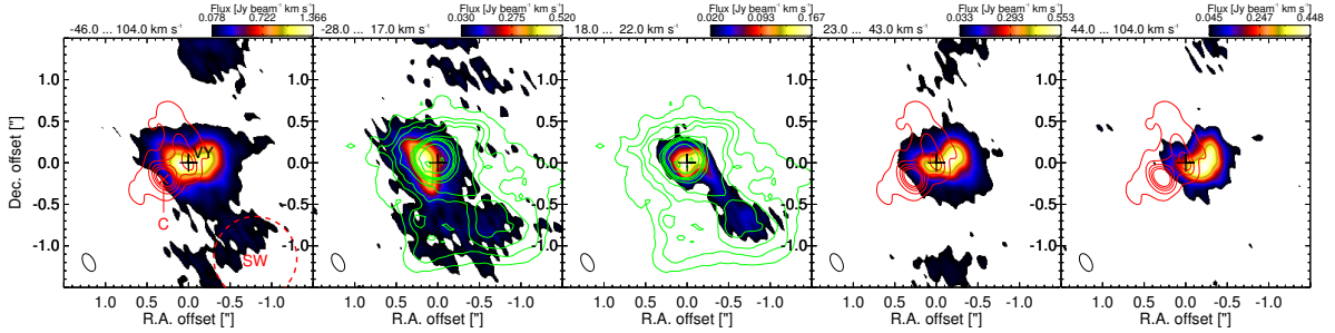
Figure 2. \text{TiO}_2 morphology. Colour maps of emission at 310.78 GHz integrated over the v_{\text{LSR}} -ranges indicated at the top left of each panel, cut off at 3\sigma . Red contours (1st, 4th, and 5th panel) show the 321 GHz continuum at [3, 20, 40, 60, 80]\sigma ; green contours (2nd and 3rd panel) show HST emission at [3, 5, 7, 10, 20, 30, 40, 50, 100, 200]\sigma [12]. In the 1st panel we marked the position of the star (+, VY; black) and of the continuum component (x, C; red) to the south-east [14, 15], and the position and approximate extent of the south-west clump (SW, dashed 1'' diameter circle; red) [11]. The apparent north-south emission is thought to arise from dynamic-range limitations in the peak channels.
