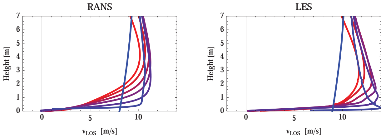
Figure 8. Mean wind profiles calculated by RANS (left) and LES (right). The figures should be comparable to Figure 5 except from a scaling factor on the velocities.
