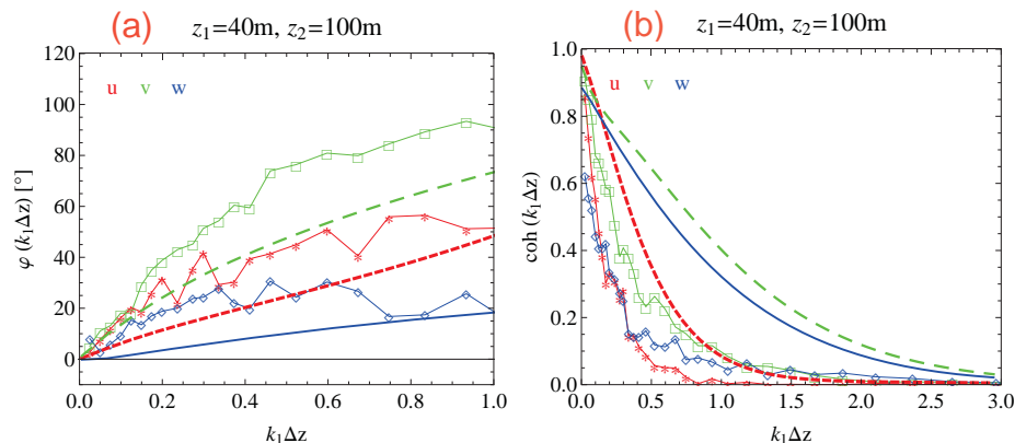
Figure 4. The phases (a) and the coherences (b) between 40 and 100 m at Høvsøre for a neutral ABL fitted with the Mann model [2]. Measurements: \phi_u ; -\ast- , \phi_v ; -\square- , \phi_w ; -\diamond- . Model: \phi_u ; --- , \phi_v ; -.- , \phi_w ; --- . Similar notations are followed for the coherences.
