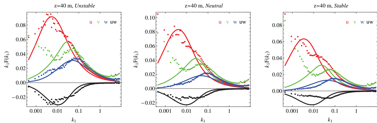
Figure 3. Example of the model fit of single-point spectra to the Høvsøre data at 40 m height to determine the three parameters in the Mann model [2]. Measured (co) spectra are denoted by points and smooth lines show modeled (co) spectra. Number of thirty-minute time series used: Unstable; 165, Neutral; 176 and Stable; 538.
