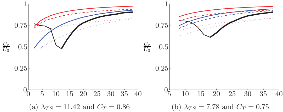
Figure 2. Center wake velocity behind a single wind turbine. — : CFD, U_c . — : Jensen with \alpha_J = 0.05 . - - : Jensen fit to \frac{\delta_1}{R} . ..... : Jensen fit to \frac{\delta_2}{R} . — : Frandsen with \alpha_J = 0.05 . - - : Frandsen fit to \frac{\delta_1}{R} . ..... : Frandsen fit to \frac{\delta_2}{R} .
