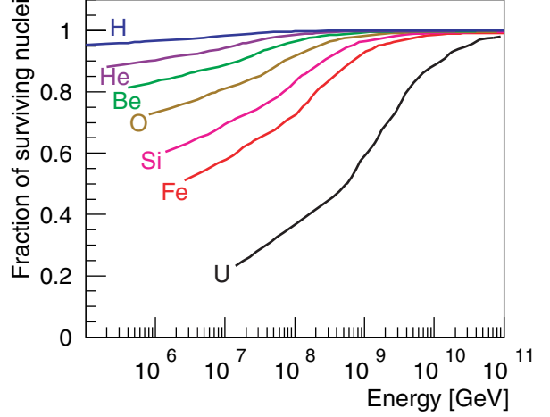
Figure 11. Fraction of nuclei surviving without interaction in the Galaxy for different elements.
