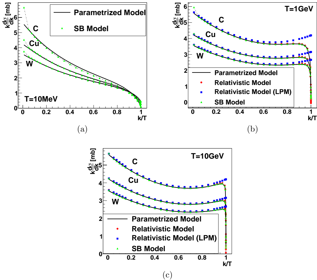
Figure 2. Plots (Relativistic Model, LPM effect activation, Seltzer-Berger Model and Parametrization Model ) for Z = 6, 29, 74 and T=10 MeV, 1 GeV and 10 GeV, respectively.
