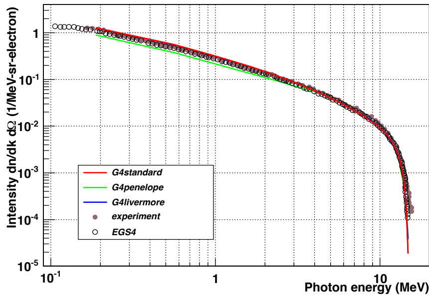
Figure 10. Bremsstrahlung intensity spectrum for a 15 MeV electron beam off 36.1 mm Aluminum target evaluated at the angle of 10^\circ : solid points – data [38], opened points – EGS4 published result, histograms – Geant4 models.
