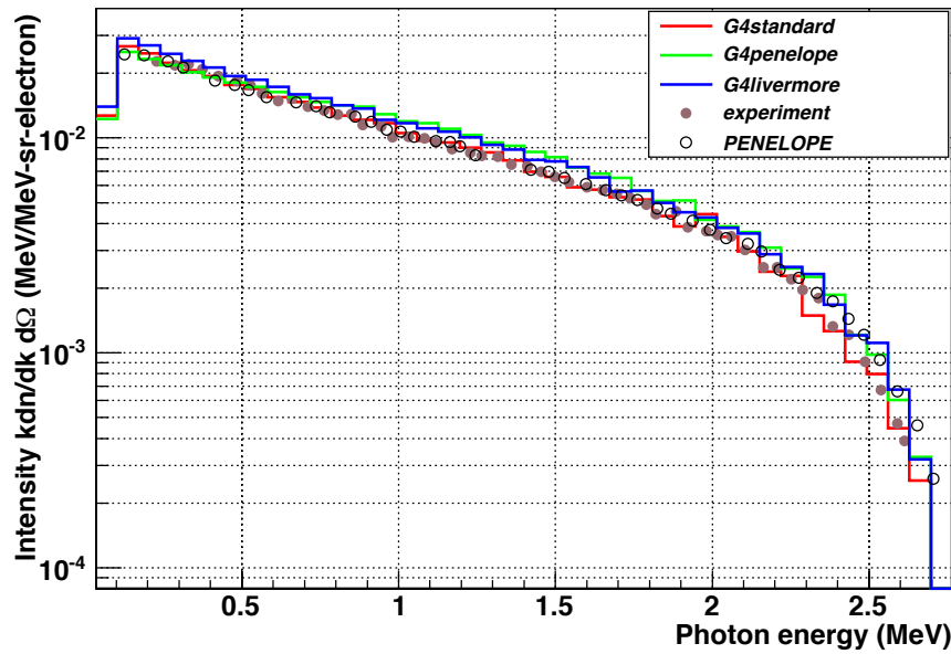
Figure 9. Bremsstrahlung intensity spectrum for a 2.8 MeV electron beam off 6.41 mm Aluminum target evaluated at the angle of 15^\circ : solid points – data [37], opened points – PENELOPE published result, histograms – Geant4 models.
