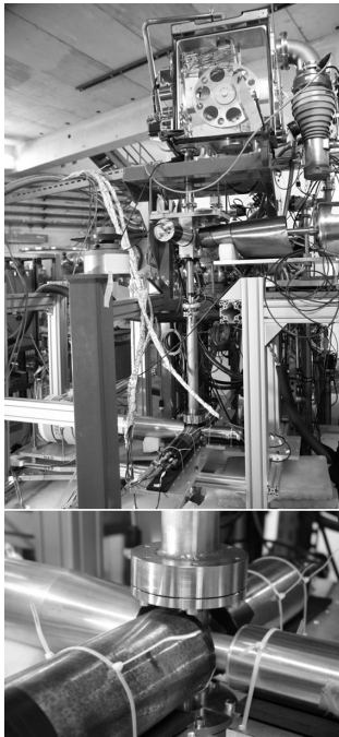
Figure 4. The 4-detector Fast-timing set-up used to measure half-lives at the ALTO beam line.
