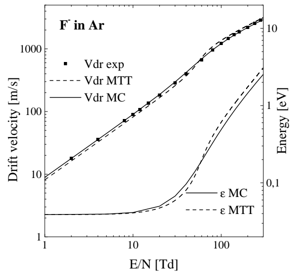
Figure 7. The drift velocity and mean energy for \text{F}^- in Ar at T=300\text{K} . Squares are experimental results taken from Ellis et al. [15].
