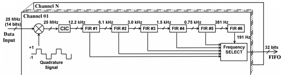
Fig. 5: The Digital Multi-Frequency Demodulator algorithm is shown schematically.
