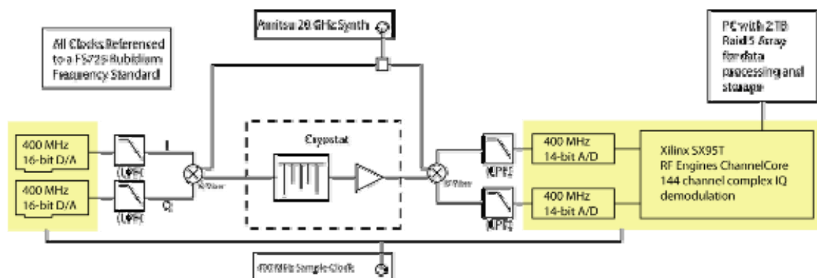
Figure 9. A block diagram of a SDR readout.
