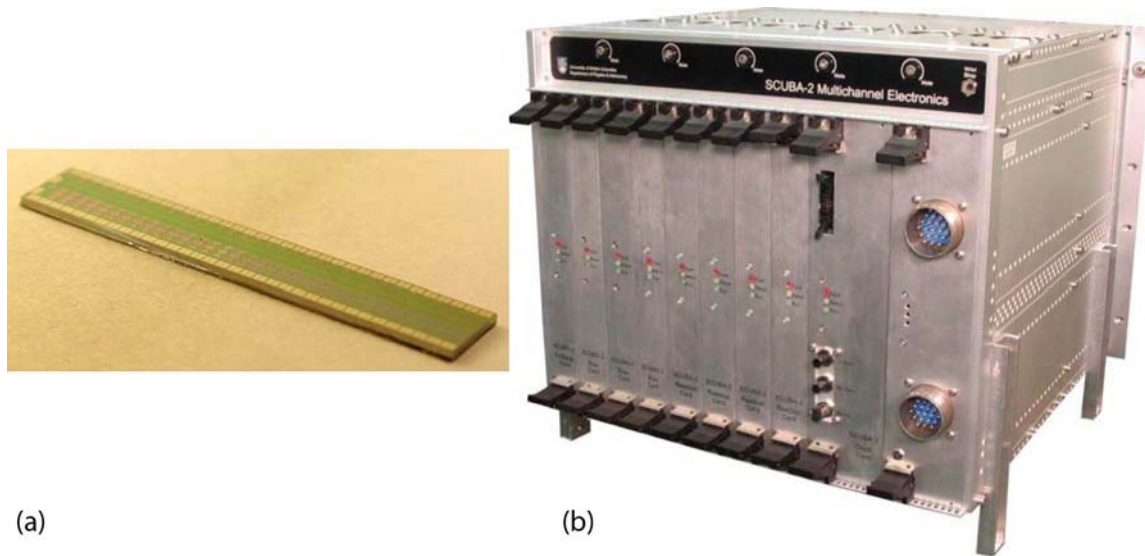
Fig. 1. (a) A 32-channel SQUID multiplexer chip. The chip dimension is 3 \text{ mm} \times 20 \text{ mm} . The 32 SQUIDs are turned on sequentially and read out through one output channel. (b) A Multi-Channel Electronics (MCE) module fabricated by the University of British Columbia. This module can instrument up to 32 output channels, and read out up to 1,280 TES bolometer channels.
