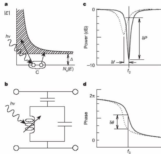
Figure 7. The mechanics of a MKID.
