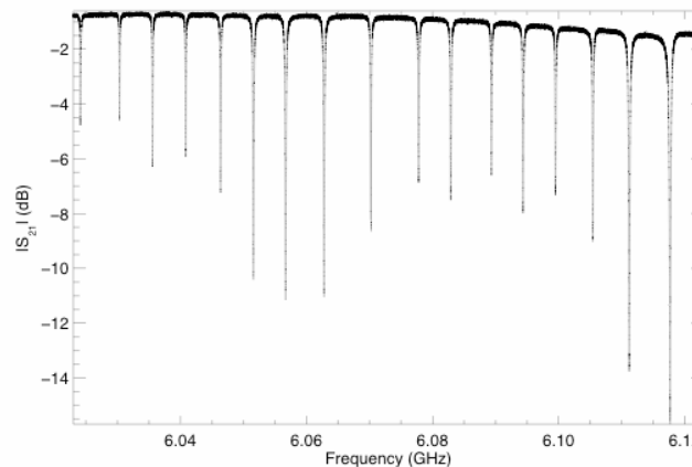
Figure 8. Transmission past a microwave MKID array.
