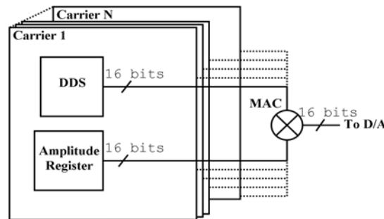
Fig. 4: The Digital Multi-Frequency Synthesizer algorithm is shown schematically.
