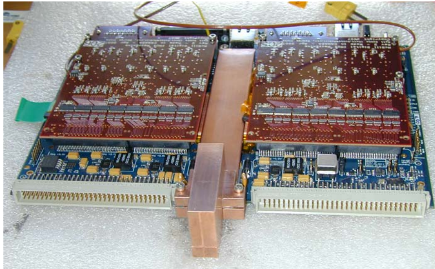
Fig. 6: The digital fMUX backend electronics. An FPGA motherboard is shown (large lower blue board) with two of its analog converter mezzanine boards attached (smaller upper red boards) and the copper convective heat pipe and conductive heat sink.
