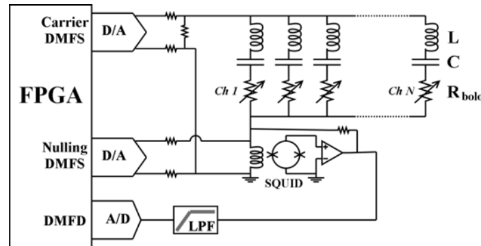
Fig. 3: The digital frequency domain multiplexer system is shown schematically.
