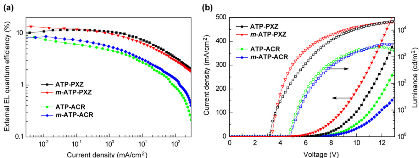
Figure 8. (a) External EL quantum efficiency versus current density curves and (b) current density–voltage–luminance ( J – V – L ) characteristics of TADF-OLEDs with device configurations of ITO/ \alpha -NPD/6 wt%-emitter:host/TPBi/LiF/Al for ATP-PXZ and m -ATP-PXZ, and ITO/ \alpha -NPD/mCP/6 wt%-emitter:host/PPT/TPBi/LiF/Al for ATP-ACR and m -ATP-ACR.
