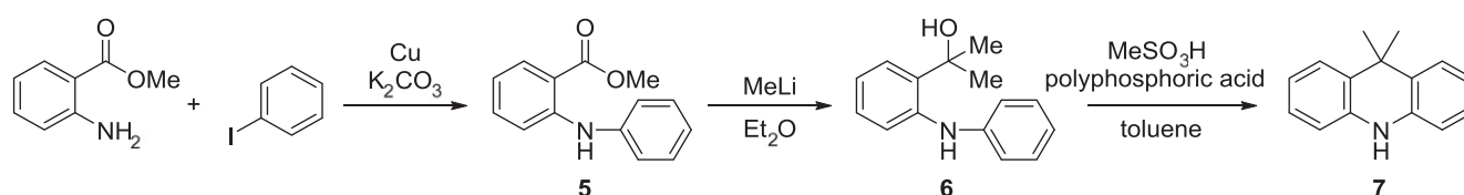
Scheme 1. Synthesis of 9,9-dimethylacridane.
