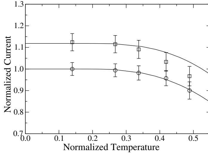
Figure 2. Critical currents (in units of the critical current on the reference chain at T = 1.2 K) as a function of T/T_c for the backbone and the chain. The solid lines are the estimated critical currents for the backbone (top) and the chain (bottom). Circles (squares): experimental values for the chain (backbone).
