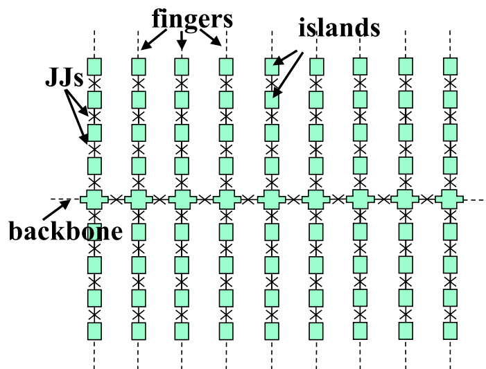
Figure 1. Schematic drawing of a comb array. The superconducting islands (full box) are connected in series to each other through JJs. The finger arrays are connected to each other only through JJs to the central islands forming the backbone array.
