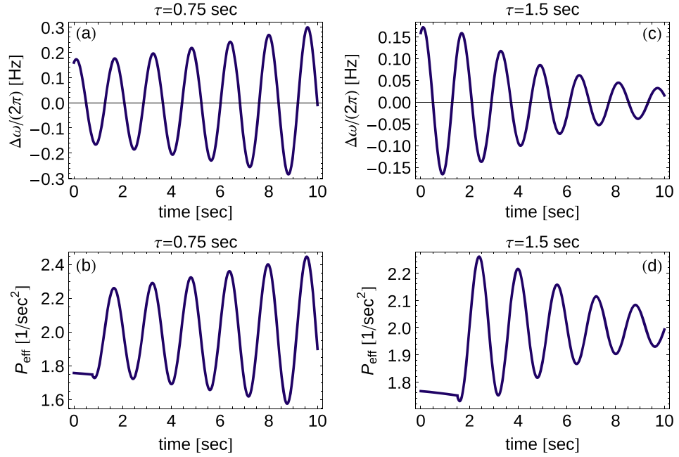
Figure 3. Decentral Smart Grid Control can stabilize or destabilize the grid. Panels (a)–(d) show the frequency difference \Delta\omega/(2\pi) and effective power P_{\text{eff}} = 2P - \gamma\Delta\omega_\tau for an elementary two-node network as a function of time for two different delays, according to (23). For the delay \tau_1 = 0.75 s the effective power becomes large simultaneously to the frequency difference, i.e., the generator produces more energy than needed, when the frequency is already too high, see (a) and (b). Hence, the system gets destabilized completely. On the contrary, the effective power and frequency difference are shifted by half a period for \tau_2 = 1.5 s such that the system is stabilized, see (c) and (d). Initial conditions were \Delta\theta_0 = 0 , \Delta\omega_0 = 1 Hz and the parameters \gamma = 0.25 \text{ s}^{-1} , \alpha = 0.1 \text{ s}^{-1} , P = 1 \text{ s}^{-2} , K = 8 \text{ s}^{-2} were applied.
