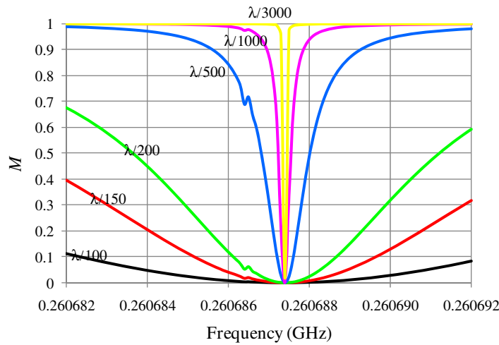
Figure 5. Detail of M as a function of frequency in a narrow band around a notch frequency for different drain port positions. The notch frequency is f = 0.260\,687\,4 GHz ( \nu = 4.996 ). The nearest Schumann frequency is f = 0.260\,866\,09 GHz ( \nu = 5 ), which is outside the range of this figure.
