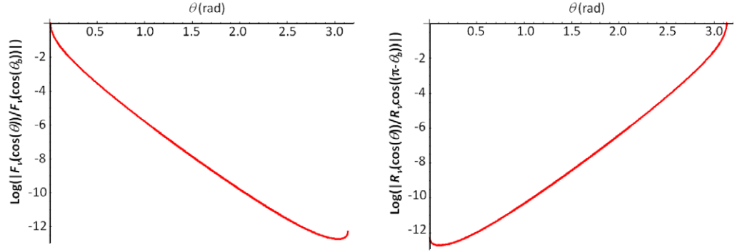
Figure A.2. Graphs for \text{Log}(|F_{v_n}(\cos(\theta))/F_{v_n}(\cos(\theta_b))|) and \text{Log}(|R_{v_n}(\cos(\theta))/R_{v_n}(\cos(\pi - \theta_b))|) as a function of \theta for v_n = -0.5 + 4.0j . F_{v_n}(\cos(\theta)) and R_{v_n}(\cos(\theta)) have a near-exponential attenuation similar to the evanescent waves in conventional waveguides. The modes with complex v_n are not transmitted. The only modes that exist inside the SWG far from the interface are the modes having real v_n . For the band of frequencies and dimensions analyzed here, only v_0 is real and the guide works as single-mode.
