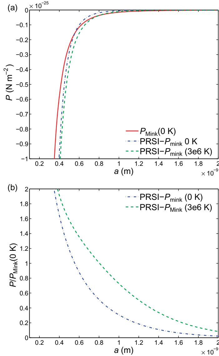
Figure 2. P_{\text{RSI}}^{\text{DD,NN}} - P_{\text{Mink}}^{\text{DD,NN}} for a massless scalar bulk field with k = 10^{19} \text{ GeV} and d = e^{-k\pi r_c} = 10^{-26} . (a) The difference between the Casimir force for RSI and flat (3+1)-spacetime at T = 0 and T = 3 \times 10^6 \text{ K} . The Casimir force for a massless scalar field in flat spacetime at zero temperature is included for comparison. (b) The ratio of the difference between the Casimir force in RSI and flat spacetime at T = 0 and T = 3 \times 10^6 \text{ K} to the force at zero temperature in flat spacetime.
