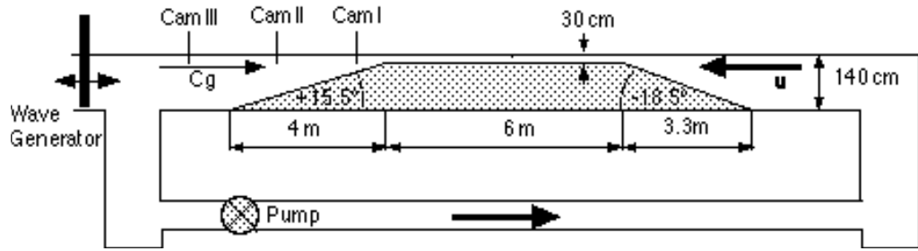
Figure 6. Schematic diagram of the experiment.
