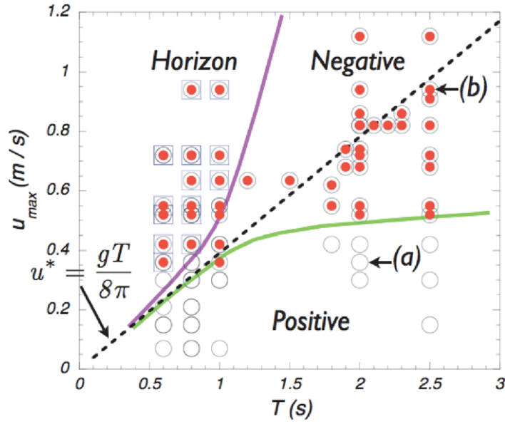
Figure 7. Phase diagram of our experiment. Each circle corresponds to a run with wave period T = 2\pi/\omega and maximal flow speed u_{\max} . The dots indicate runs where we observed negative-frequency waves, the squares run with horizons. In regimes without horizons, we saw a transition to mode conversion into purely positive frequencies below the lower green line in the diagram. The points (a) and (b) indicate the parameters used in figure 8.
