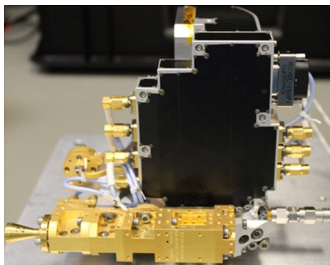
Figure 21. Spaceflight qualified 166 GHz heterodyne radiometer for the MetOp-second generation series of operational meteorology satellites. The volume of 120 \times 120 \times 106 \text{ mm}^3 incorporates a low noise amplifier, sub harmonic Schottky diode mixer and local oscillator system.
