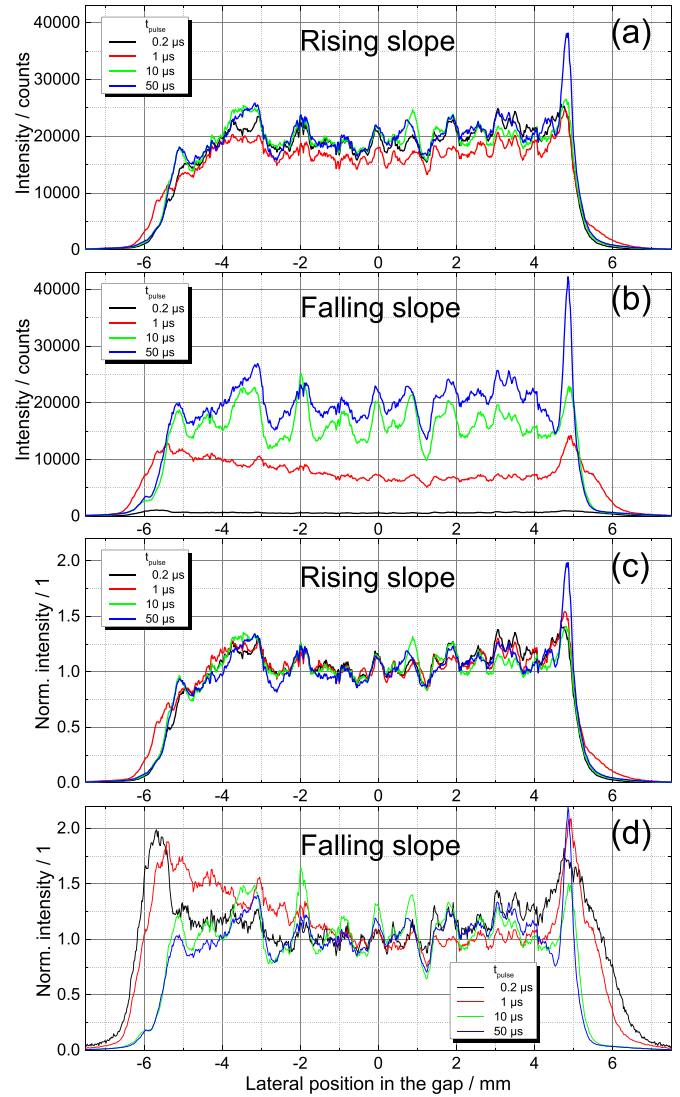
Figure 11. Lateral profiles of discharge emission in the axial centre of the gas gap (axially averaged over 80\ \mu\text{m} ) obtained from the accumulated iCCD images in figure 10. (a) and (b) show the directly comparable intensity while the intensity is normalised with respect to the mean value of the plateau in the gap centre in (c) and (d).
