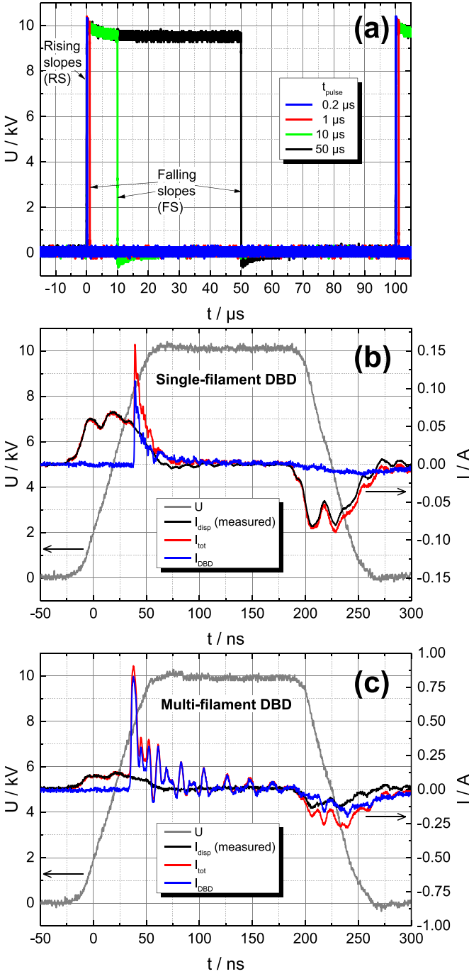
Figure 4. Overview of applied HV pulses (a) under t_{\text{pulse}} variation, and an example for a single- and multi-filament DBD with different current components (displacement ( I_{\text{disp}} ), total ( I_{\text{tot}} ) and discharge ( I_{\text{DBD}} ) current) at both slopes for t_{\text{pulse}} = 0.2 \mu\text{s} (b) and (c).
