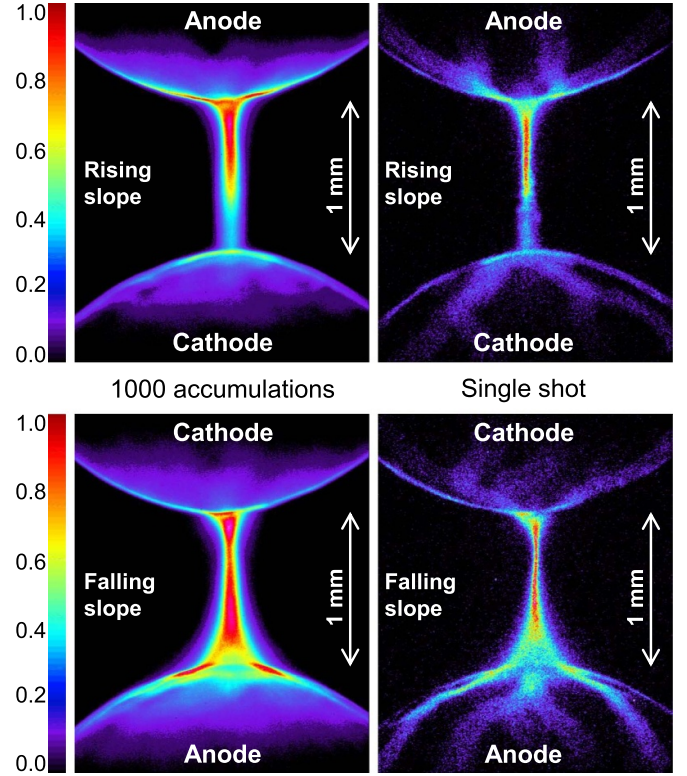
Figure 9. Overall discharge structure at both HV slopes in the single-filament arrangement for 1 \mu s HV pulse width and 250 ns iCCD gate; left column 1000 accumulations (with no MCP (microchannel plate) gain), right column single shot (with 200 MCP gain).
