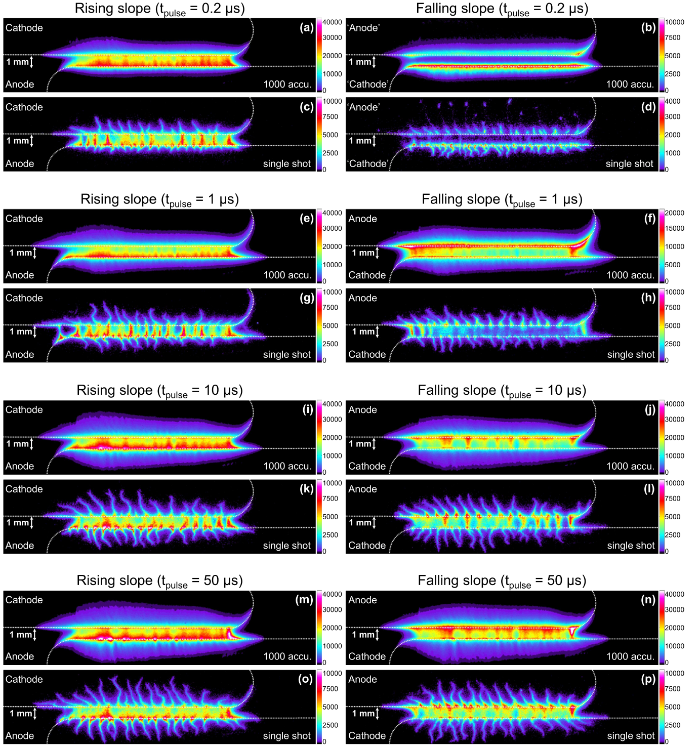
Figure 10. Overview of overall discharge structure at both HV slopes in the multi-filament arrangement for all used HV pulse widths showing accumulation of 1000 subsequent discharge events (no iCCD gain) and a single shot (iCCD gain 200), intensity scaled linearly in pseudocolour (note the different absolute intensity values), iCCD gate width 250 ns for (a)–(d) and 500 ns for (e)–(p).
