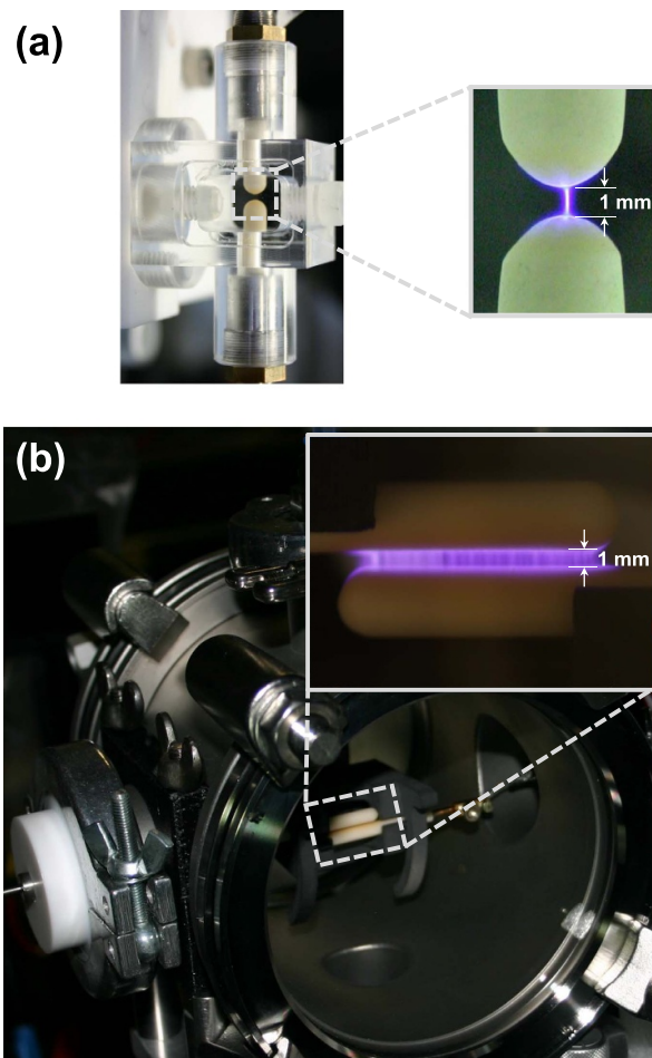
Figure 1. Plexiglas cell with the single-filament arrangement (a), stainless steel discharge chamber containing the multi-filament arrangement (b); photographs of the running DBDs in the 1 mm gap are shown for both arrangements in the respective enlargement.
