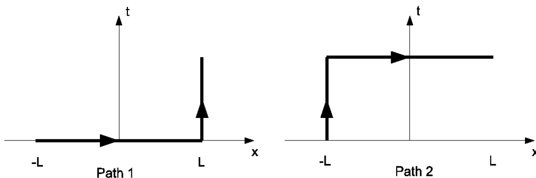
Figure 1: The two paths used to integrate equation (2.2). Since the connection A_\mu is flat the integrations along the two paths give the same result.
