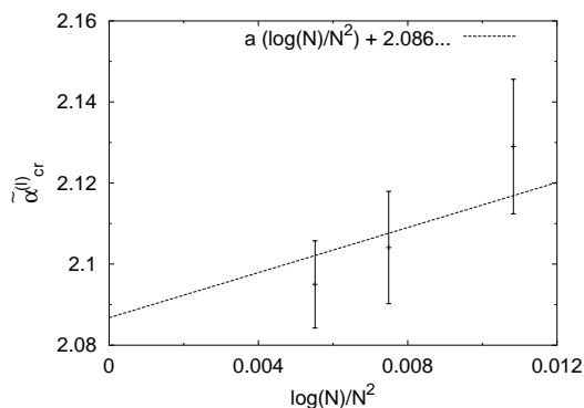
Figure 3: The lower critical point \tilde{\alpha}_{cr}^{(l)} is plotted for N = 16, 20, 24 . The dashed line represents a fit to \tilde{\alpha}_{cr}^{(l)} = (8/3)^{3/4} + a \frac{\log N}{N^2} , where a = 2.781 .
