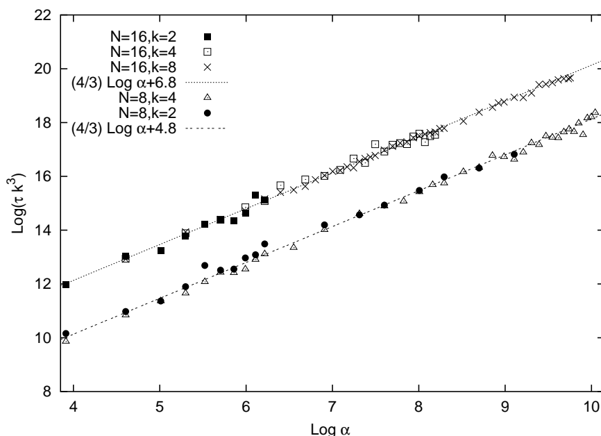
Figure 12: The ‘life time’ ( \tau ) of k coincident fuzzy spheres with k = 2, 4, 8 follows a universal power law. The plot shows \log(\tau k^3) v.s. \log \alpha for N = 8, 16 . The straight lines represent the fits to \log(\tau k^3) = \frac{4}{3} \log \alpha + c .
