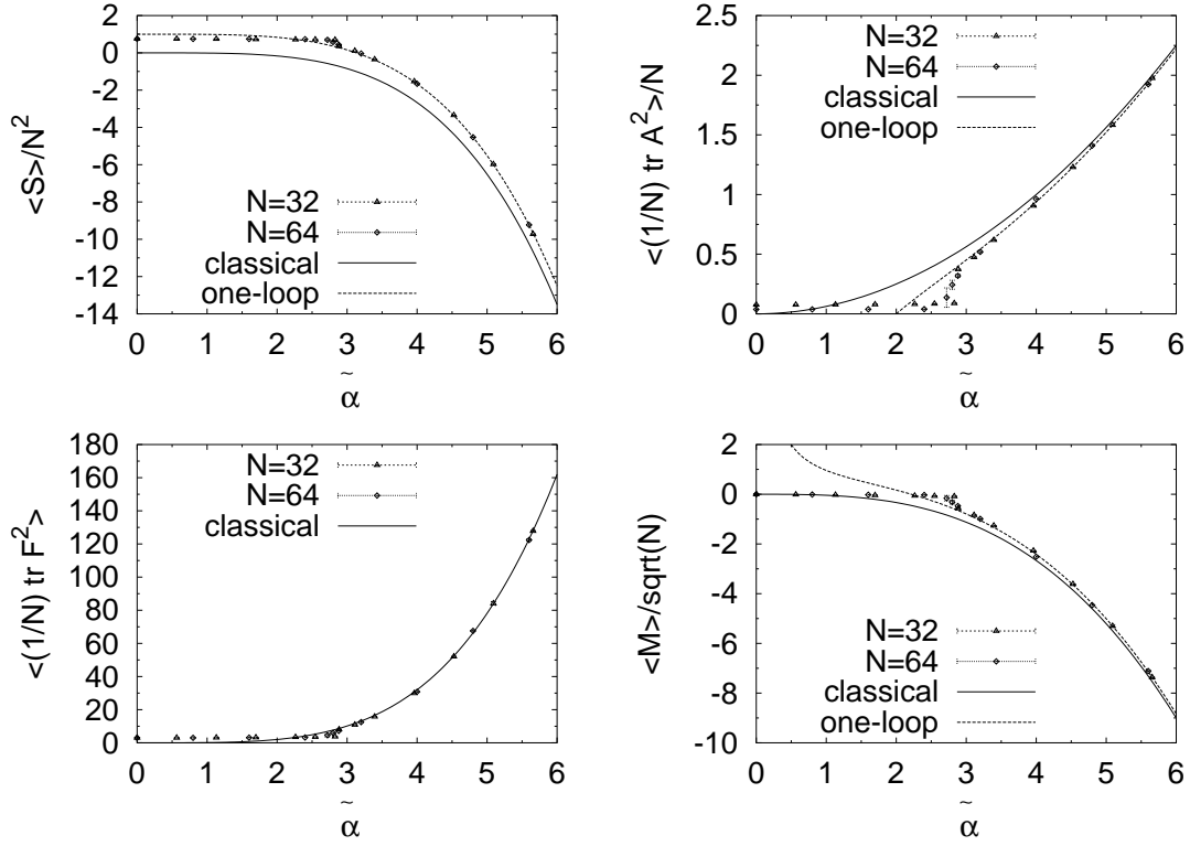
Figure 13: Various observables are plotted against \tilde{\alpha} for N = 32, 64 . The initial configuration is taken to be the k = 2 coincident fuzzy spheres (6.2), and the measurement has been made before they decay into other states.
