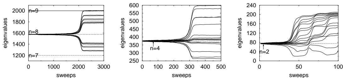
Figure 11: The history of the eigenvalues of the Casimir operator (5.2) is plotted for N = 16 , \alpha = 10.0 . The initial configuration is taken to be the k coincident fuzzy spheres (6.2) with k = 2 (left), k = 4 (middle) and k = 8 (right).
