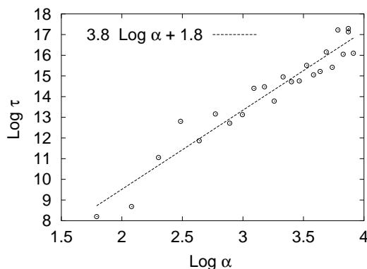
Figure 10: The ‘life time’ ( \tau ) of the multi fuzzy spheres \langle 3, 5 \rangle for N = 8 is shown as a function of \alpha in the log-log plot. The straight line represents a fit to the power law.
