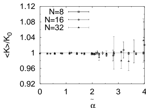
Figure 4: The ratio \langle K \rangle / K_0 is plotted against \tilde{\alpha} for N = 8, 16, 32 with the single fuzzy sphere start. The horizontal line corresponds to the exact result.
