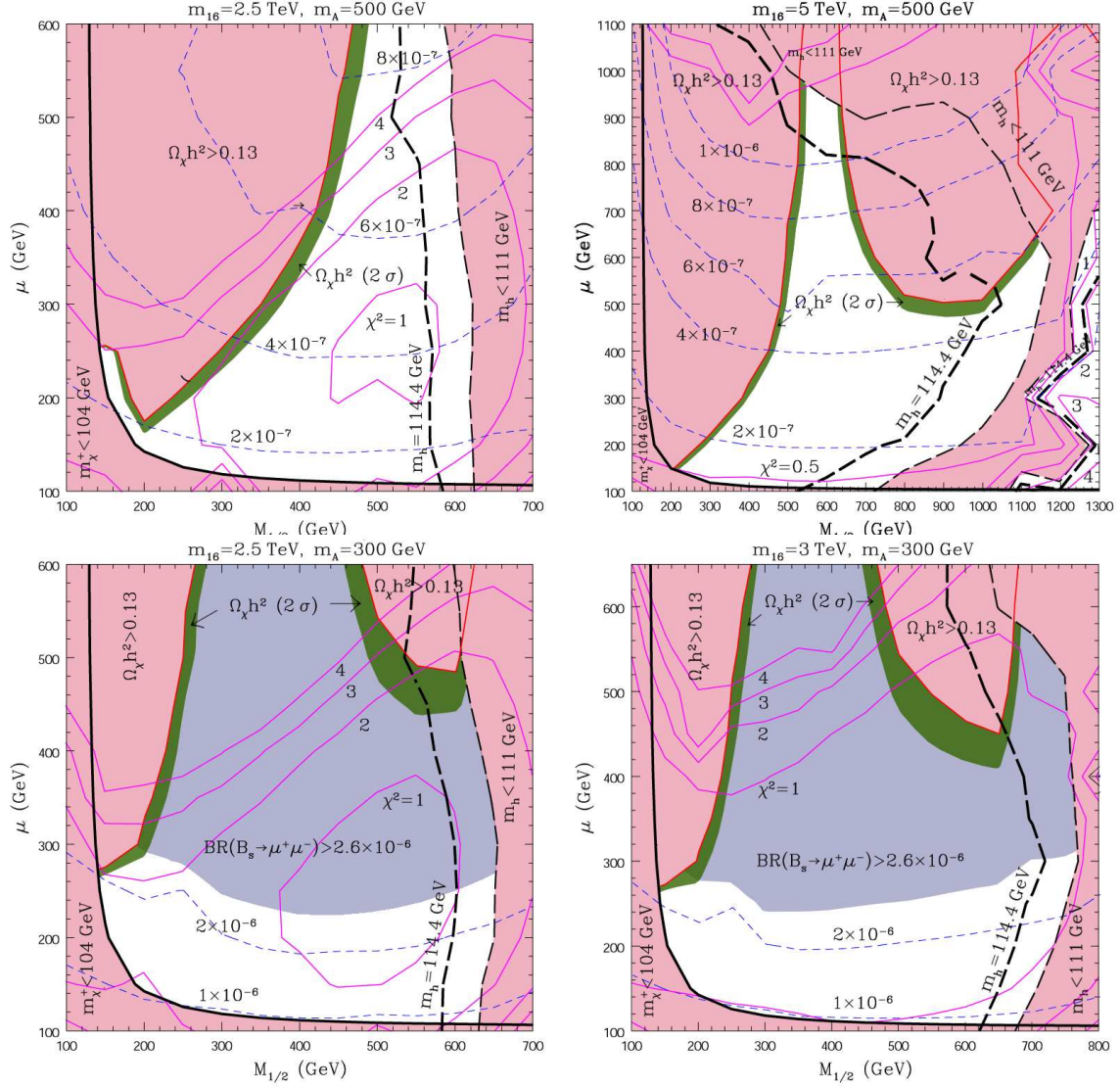
Figure 3: The same as in figure 1 but for m_{16} = 2.5 TeV and m_A = 500 GeV (upper left), m_{16} = 5 TeV and m_A = 500 GeV (upper right), m_{16} = 2.5 TeV and m_A = 300 GeV (lower left) and m_{16} = 3 TeV and m_A = 300 GeV (lower right). Also marked are contours of constant \text{BR}(B_s \rightarrow \mu^+ \mu^-) . The blue regions in the lower two panels are excluded by \text{BR}(B_s \rightarrow \mu^+ \mu^-) > 2.6 \times 10^{-6} . Note the different mass ranges for M_{1/2} and \mu in the different panels.
