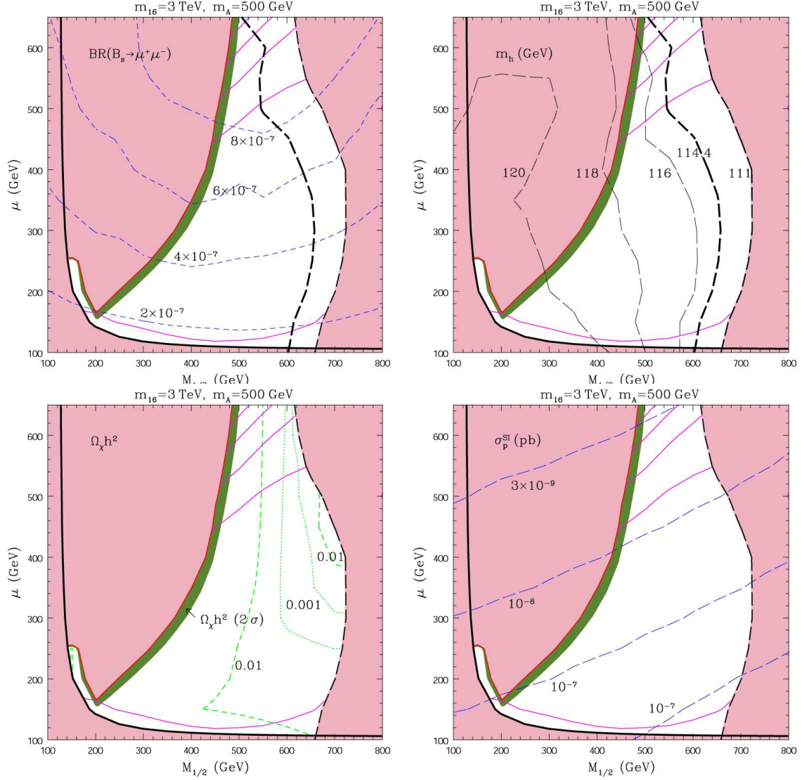
Figure 2: Same as figure 1 with contours of constant \text{BR}(B_s \rightarrow \mu^+ \mu^-) (upper left), m_h (upper right), \Omega_\chi h^2 (lower left) and \sigma_p^{SI} (lower right) for m_{16} = 3 TeV and m_A = 500 GeV.
