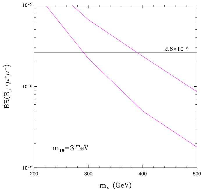
Figure 4: The upper and lower limits on \text{BR}(B_s \rightarrow \mu^+ \mu^-) as a function of m_A in the \mu, M_{1/2} region of parameter space satisfying all the collider constraints, 0.095 < \Omega_\chi h^2 < 0.13 and \chi^2 < 2 for fixed m_{16} = 3 \text{ TeV} .
