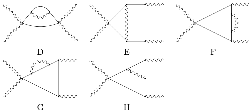
Figure 3: Graphs relevant for the photino and scalar electron contributions \mathcal{M}^{(2),P} and \mathcal{M}^{(2),S} . The solid lines represent the scalar electron while the wavy lines denote either the photon or photino.
