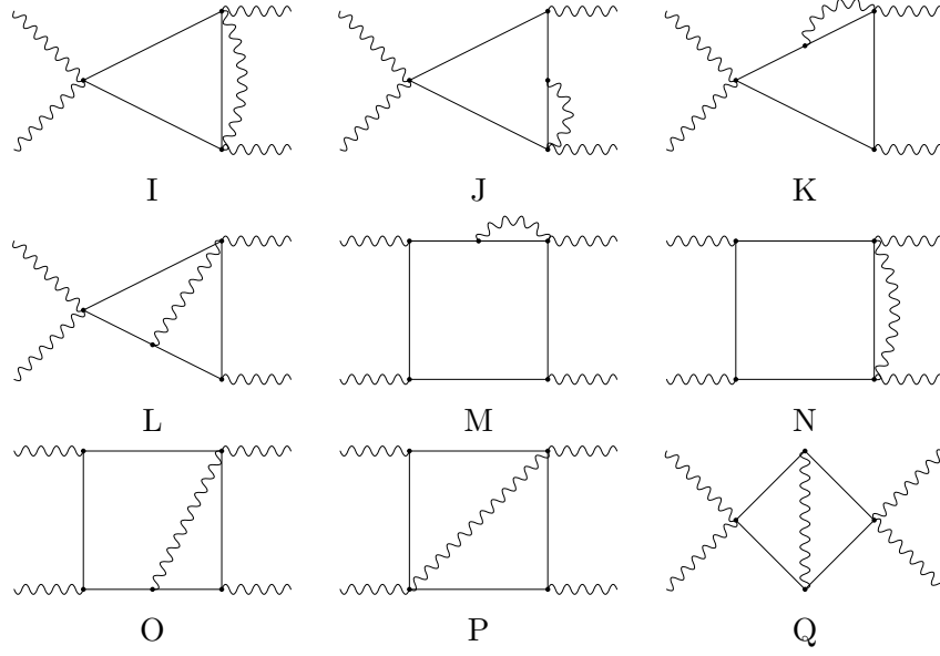
Figure 4: Graphs relevant for the scalar electron contribution \mathcal{M}^{(2),S} . The solid lines represent the scalar electron while the wavy lines denote the photon.
