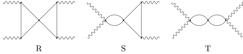
Figure 5: Graphs relevant for the scalar four-point interaction contribution \mathcal{M}^{(2),V} . The solid lines represent the scalar electron while the wavy lines denotes the photon.
