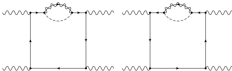
Figure 1: Typical diagrams involving the photino that are related by charge conjugation. The dashed line represents the scalar electron, while the overlaid solid and wavy lines represent the photino. Similar graphs can be drawn where the dashed line represents the scalar photon and the overlaid solid and wavy lines represent the electron.
