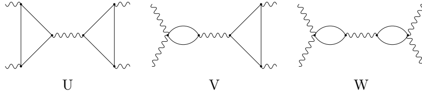
Figure 6: One-particle reducible graphs relevant for the electron, scalar electron and scalar photon contributions \mathcal{M}^{(2),F} , \mathcal{M}^{(2),S} and \mathcal{M}^{(2),X} . The solid lines represent particles from the matter multiplet, i.e. the electron or scalar electron while the wavy lines denote the photon or scalar photon. Graphs V and W are only part of the scalar electron contribution.
