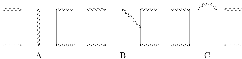
Figure 2: Graphs relevant for the electron, photino, scalar electron and scalar photon contributions \mathcal{M}^{(2),F} , \mathcal{M}^{(2),P} , \mathcal{M}^{(2),S} and \mathcal{M}^{(2),X} . The solid lines represent particles from the matter multiplets, i.e. the electron or scalar electron while the internal wavy lines denote particles from the gauge multiplets, the photon, the photino or the scalar photon.
