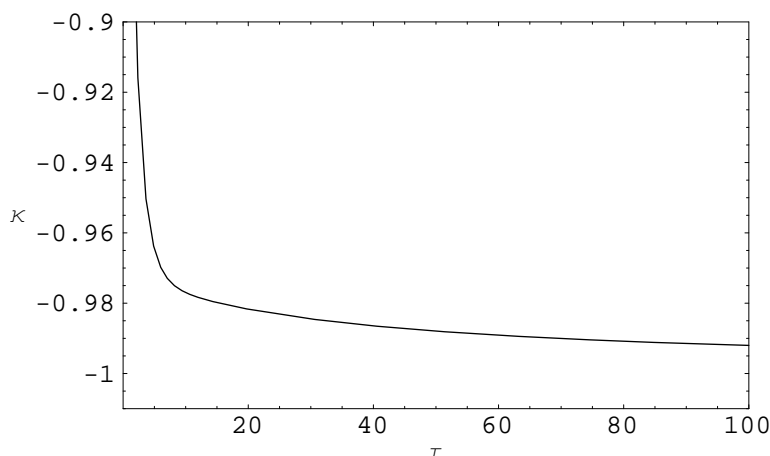
Figure 4: Asymptotic behavior of the equation of state for the potential (3.10). \tau is measured in units of 1/H_0 .
