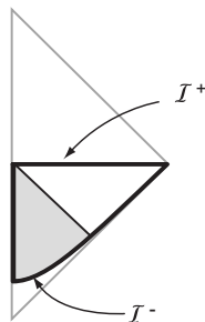
Figure 2: Adding a radiation component renders \mathcal{I}^- spacelike. The shaded triangle is the region accessible to the observer at r = 0 .
