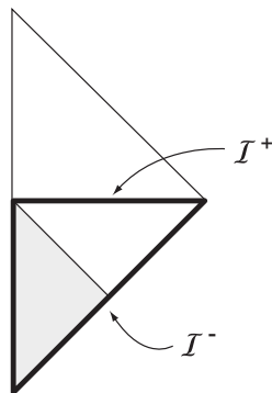
Figure 1: The lower triangle is the Penrose diagram for flat FRW space with \kappa < -1/3 . The shaded triangle is the region accessible to the observer at r = 0 .
