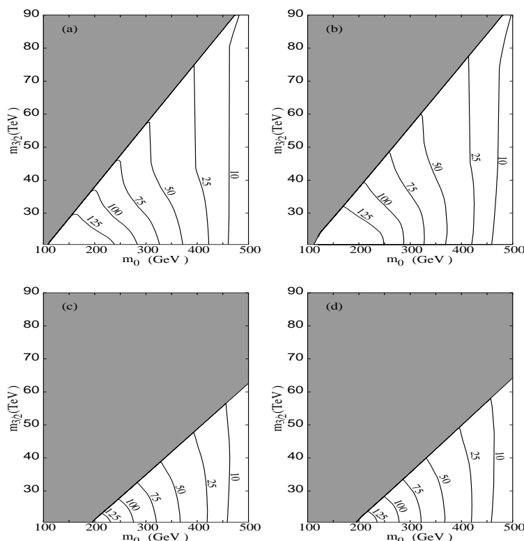
Figure 1: Constant cross section (in fb) contour plots in the m_0 - m_{3/2} plane for (a) \mu < 0 , \tan \beta = 3 , (b) \mu > 0 , \tan \beta = 3 , (c) \mu < 0 , \tan \beta = 30 and (d) \mu > 0 , \tan \beta = 30 .
