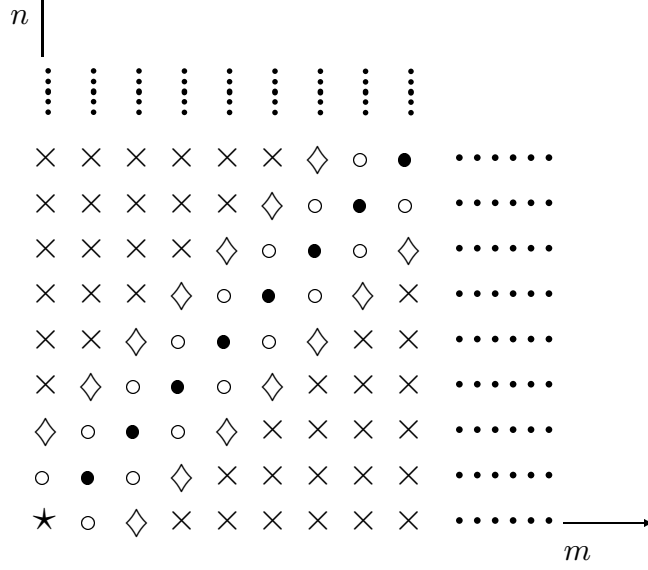
Figure 1: Each entry of the integer grid, m, n = 0, 1, 2, \dots , represents a component \omega(m, n; \theta) of the shs^E(8|4) valued connection one form \omega according to the following rule: the \star denote the spin s = 1 component; a \bullet denotes a generalized vierbein; a \circ denotes a generalized gravitino; a \diamond denotes an auxiliary generalized Lorentz connection and the \times 's denote the remaining auxiliary connections.
