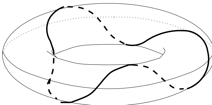
Figure 11: A pictorial representation of a cycle of type (1, 3) , which is wrapped by the NS branes in the 3 \times 1 box model of figure 6.
