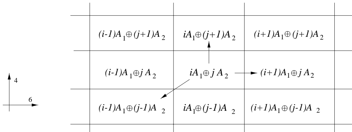
Figure 4: A typical region in a brane box model constructed from a singularity. The arrows denote the chiral multiplets \Phi_{I, I \oplus A_1} , \Phi_{I, I \oplus A_2} , and \Phi_{I, I - A_1 - A_2} , for I = iA_1 \oplus jA_2 , which appear as the horizontal, vertical and diagonal fields.
