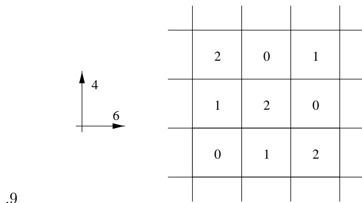
Figure 5: The relation between the n_1 \times n_2 box rectangle and the true unit cell in a general brane box configuration.
