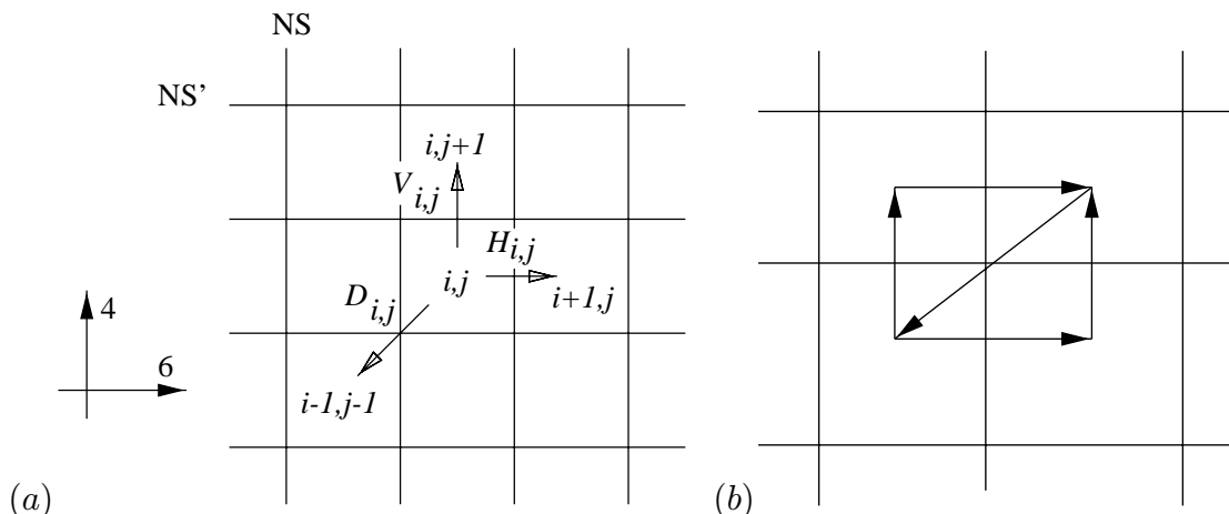
Figure 1: (a) Conventions for denoting the chiral multiplets which are in the fundamental of the group SU(n_{i,j}) and in the antifundamental of an adjacent group. (b) The two superpotential couplings at each corner are represented by an oriented triangle of arrows.
