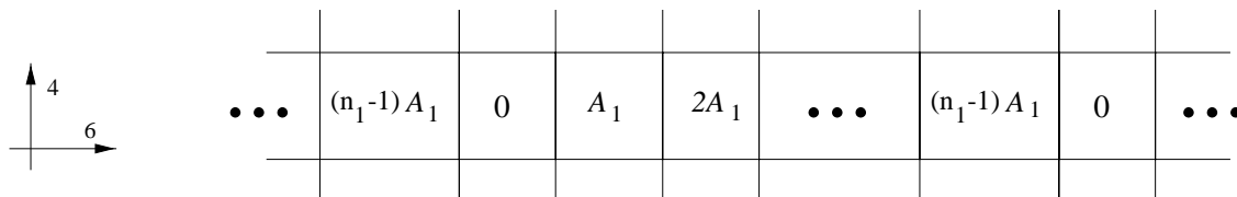
Figure 3: First step in the construction of the brane box model corresponding to a singularity C^3/\Gamma . The labels on each box denote the irreducible representation of \Gamma associated to the gauge factor in that box. The basic period in the infinite array of boxes is bounded by dark lines.
