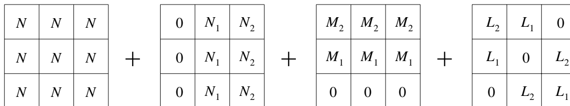
Figure 12: ‘Sewing’ \mathcal{N} = 2 models: A large family of theories can be obtained by adding together models formed by whole rows, columns and diagonal lines of boxes. Here the numbers denote the number of D5 branes in the box.
