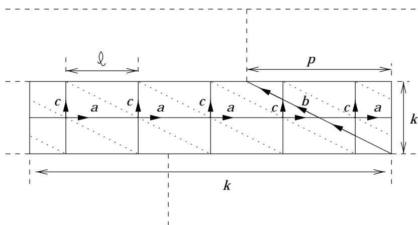
Figure 10: The unit cell in a model with k = 5\ell , p = 2\ell . The cycle of the torus wrapped by the NS' branes is the horizontal line labeled ' a '. The cycle ' c ' corresponding to the NS branes wraps the vertical direction several times due to the shifted identifications (suggested by the dotted lines). The cycle ' b ', corresponding to the slanted line, is the dual to ' a '.
