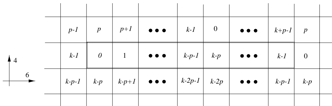
Figure 7: The brane box configuration obtained from the C^3/Z_k singularity described in the text. It corresponds to a k \times 1 box model with trivial identifications of vertical sides and identifications of the horizontal sides up to a shift of p boxes to the left.
