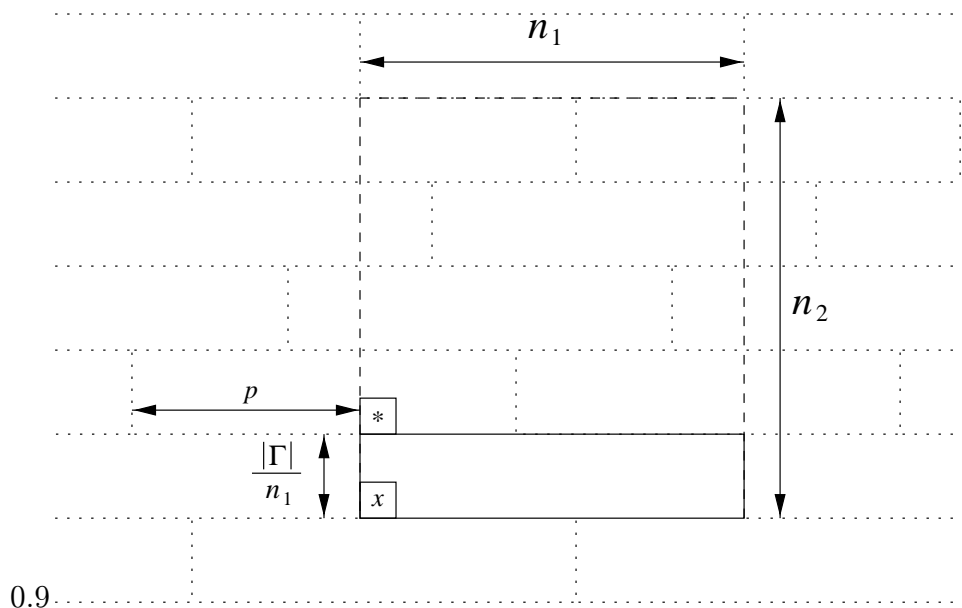
Figure 5: The relation between the n_1 \times n_2 box rectangle and the true unit cell in a general brane box configuration.
