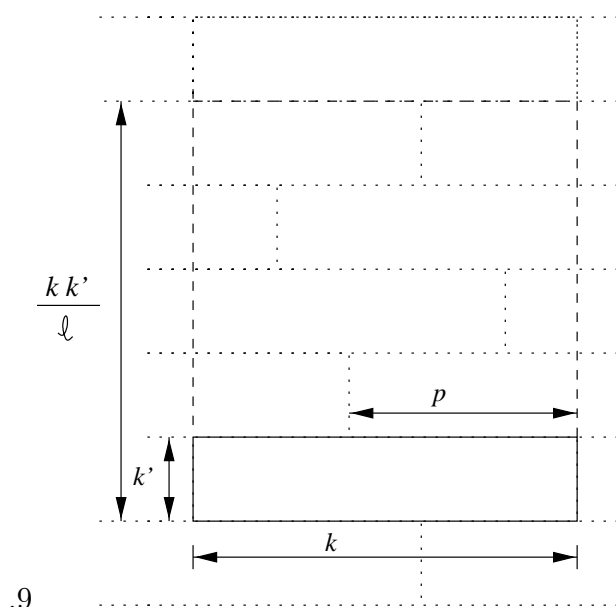
Figure 9: By adjoining several unit cells, we can define a larger rectangle whose sides have trivial identifications.
