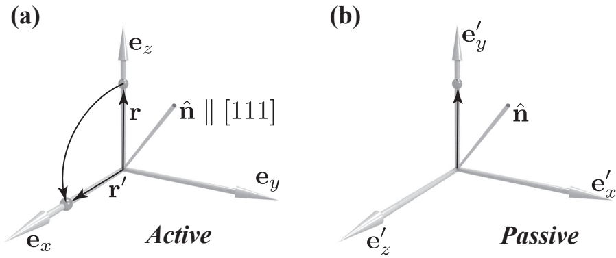
Figure 1. Illustration of active (a) and passive (b) rotations corresponding to 120^\circ around [111] .
