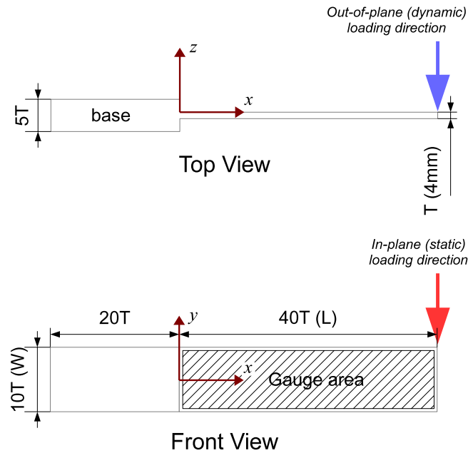
Figure 1. Geometry of the reference material with the gauge area shown shaded.
