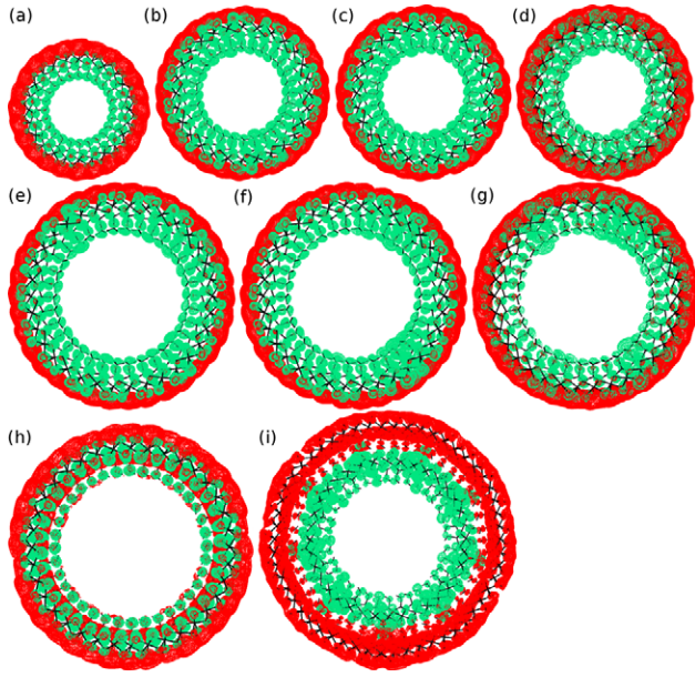
Figure 4. Front view of the VB (green) and CB edge (red) separation for the considered Imo NTs and DFT functionals. (a) AlSi 24 (PBE), (b) AlSi 28 -Me (PBE), (c) AlSi 28 -Me (PBE-D2), (d) AlSi 28 -Me (OPTB88), (e) AlSi 34 -Me (PBE), (f) AlSi 34 -Me (PBE-D2), (g) AlSi 34 -Me (OPTB88), (h) AlGe 36 (PBE), (i) DW-AlGe 36,54 (PBE). The structures in (a)–(h) are displayed according to their relative size (table 1). For more compact representation, the structure in (i) has been scaled down by a factor 1.5. The six lowest-energy occupied and highest-energy empty KS-states have been plotted for the VB and CB edge in (a)–(h), respectively. For DW-AlGe 36,54 , thirty two (sixteen occupied, sixteen empty) frontier KS-states have been used.
