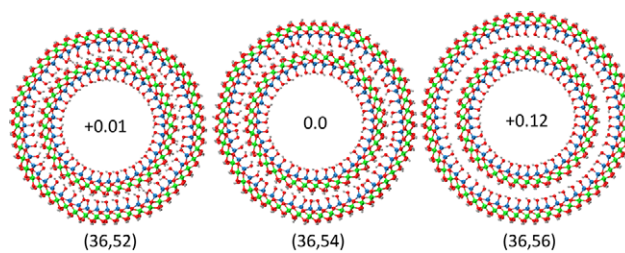
Figure 2. Front view of the optimized DW AlGe ( N_{in} , N_{out} ) NT models screened. The relative energy per (Al 2 GeO 7 H 4 ) unit (eV) is shown inside each NT-model.
