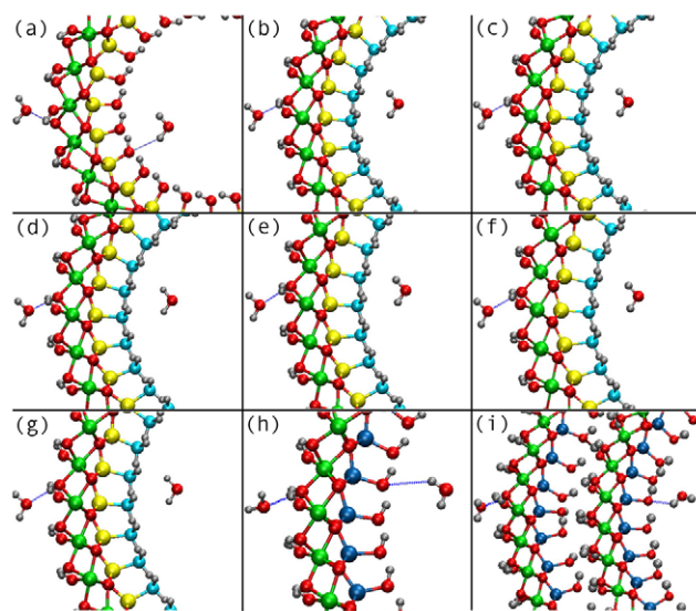
Figure 7. Close up of the optimized geometry of the considered 2\text{H}_2\text{O}@ Imo NTs models for the DFT-functionals used. (a) \text{AlSi}_{24} (PBE), (b) \text{AlSi}_{28}\text{-Me} (PBE), (c) \text{AlSi}_{28}\text{-Me} (PBE-D2), (d) \text{AlSi}_{28}\text{-Me} (OPTB88), (e) \text{AlSi}_{34}\text{-Me} (PBE), (f) \text{AlSi}_{34}\text{-Me} (PBE-D2), (g) \text{AlSi}_{34}\text{-Me} (OPTB88), (h) \text{AlGe}_{36} (PBE), (i) \text{DW-AlGe}_{36,54} (PBE). The shortest \text{H}_2\text{O} -NT H-bonding distances (see also table 4) are highlighted by dotted lines. Same atom-colour labelling as in figure 1.
