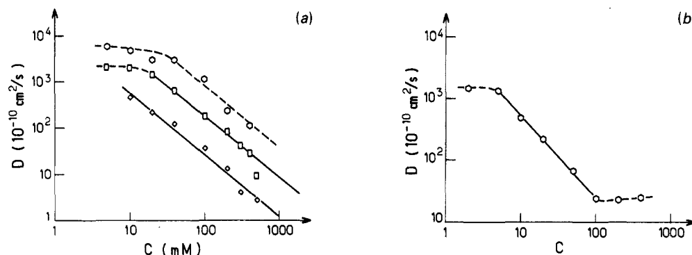
Figure 1. (a) Log-log plot of self-diffusion coefficient D_s versus lecithin concentration in iso-octane solutions at 25 °C: \circ , w_0 = 0 ; \square , w_0 = 1 ; \diamond , w_0 = 2 . The full curves are least-squares fits; the broken curves are guides for the eye. The slopes for the full curves are -1.32 for w_0 = 1 and -1.35 for w_0 = 2 . (b) CTAB + 0.5 M KBr at 35 °C. The full curve is a least-squares fit. Its slope is -1.32 .
