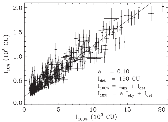
Figure 2. Pixel-by-pixel comparison of the 100% and 10% shutter aperture data. By fitting the data with a linear function, the scale factor for the 10% shutter aperture data and detector background rate are estimated. The comparison is made with the N_{\text{side}} = 64 maps. Here, CU represents the continuum unit (photons \text{cm}^{-2} \text{s}^{-1} \text{\AA}^{-1} \text{sr}^{-1} CU).
