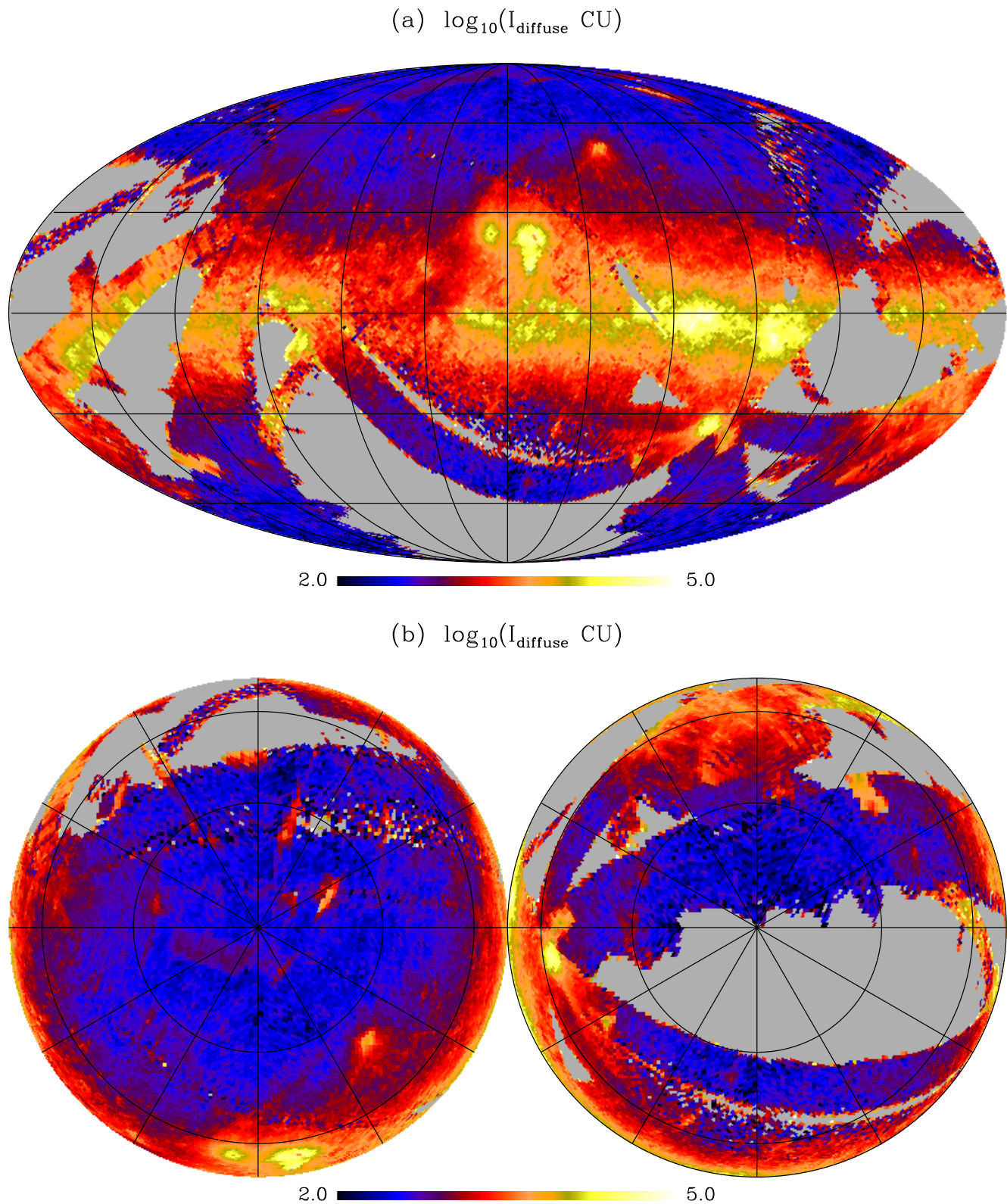
Figure 6. (a) Mollweide and (b) orthographic projections of the diffuse FUV background map observed with SPEAR/FIMS, after removal of locally intense pixels (stars) and the instrumental background. The left and right sides of orthographic projections are centered at the northern and southern Galactic polar caps, respectively, and their longitude increases clockwise and counterclockwise, respectively. In both projections, l = 0^\circ is at the six o'clock position. The intensity scales are logarithmic across the color bars. (c) Mollweide and (d) orthographic projections of signal-to-noise ratio of the diffuse FUV map. The left and right sides of orthographic projections are centered at the northern and southern Galactic polar caps, respectively, and their longitude increases clockwise and counterclockwise, respectively. In both projections, l = 0^\circ is at the six o'clock position. The intensity scales are logarithmic across the color bars.
