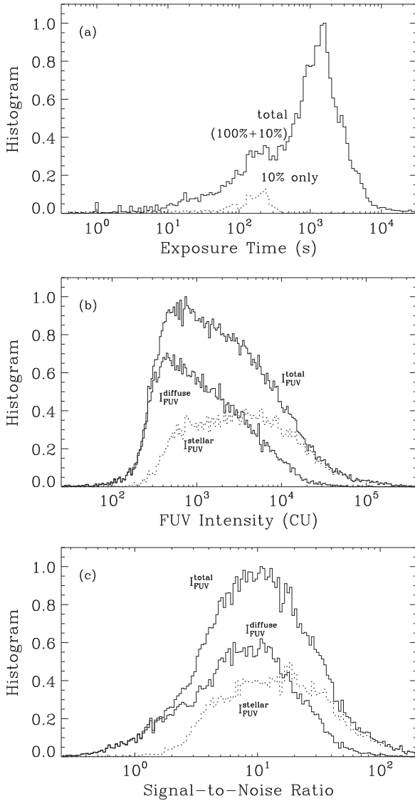
Figure 4. Histograms of (a) exposure time (s), (b) the FUV intensity (photons \text{s}^{-1} \text{cm}^{-1} \text{sr}^{-1} \text{\AA}^{-1} , CU) over the observed sky, and (c) signal-to-noise ratio with bins scaled logarithmically. The histograms are made with about 1^\circ pixels ( N_{\text{side}} = 64 ). A background of 190 CU was removed from the data to take into account the instrumental dark background.
