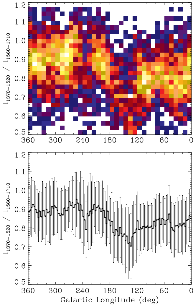
Figure 16. Hardness ratio (1370–1520 Å to 1560–1710 Å) vs. Galactic longitude. The Al II emission line was excluded in estimating the hardness ratio. (A color version of this figure is available in the online journal.)
