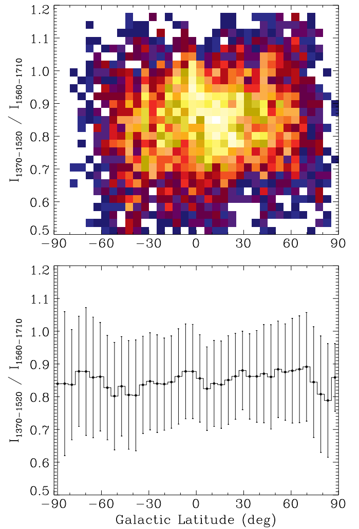
Figure 17. Hardness ratio (1370–1520 Å to 1560–1710 Å) vs. Galactic latitude. The Al II emission line was excluded in estimating the hardness ratio. (A color version of this figure is available in the online journal.)
