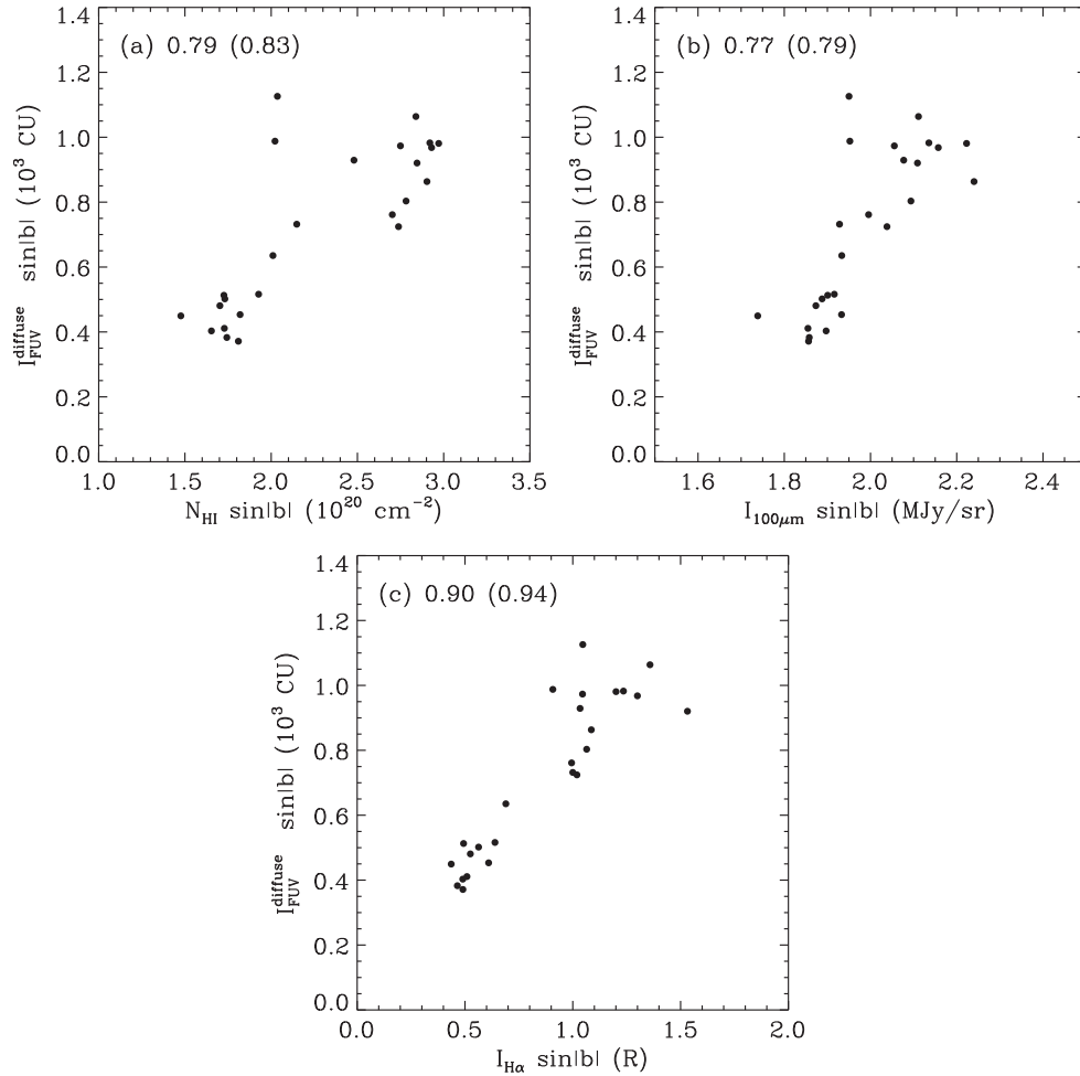
Figure 23. Correlation of the diffuse FUV continuum intensity with (a) neutral hydrogen column density, (b) 100\ \mu\text{m} emission, and (c) the diffuse \text{H}\alpha intensity after the removal of inverse- \sin|b| dependence due to the plane-parallel medium. Data points were obtained from latitude ranges of \sin|b| \geq 0.5 ( |b| \geq 30^\circ ). Numbers outside and inside the parentheses are correlation coefficients estimated in linear and logarithmic scales, respectively.
