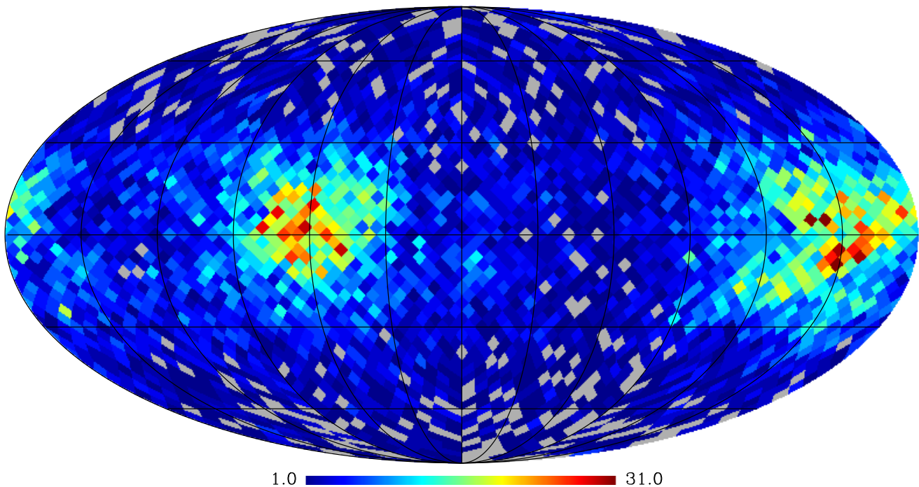
Figure 15. (a) Number of OB-type stars and (b) number of A-type stars from the TD-1 stellar catalog. The maps were made using the resolution parameter N_{\text{side}} = 16 (with \sim 3.7 pixels).
