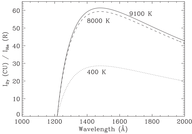
Figure 26. Two-photon continuum intensity that accompany 1 R of H \alpha emission from ionized interstellar hydrogen. The continuum intensity is shown for three temperatures: 9100 K, solid line; 8000 K, dashed line; and 400 K, dotted line.
