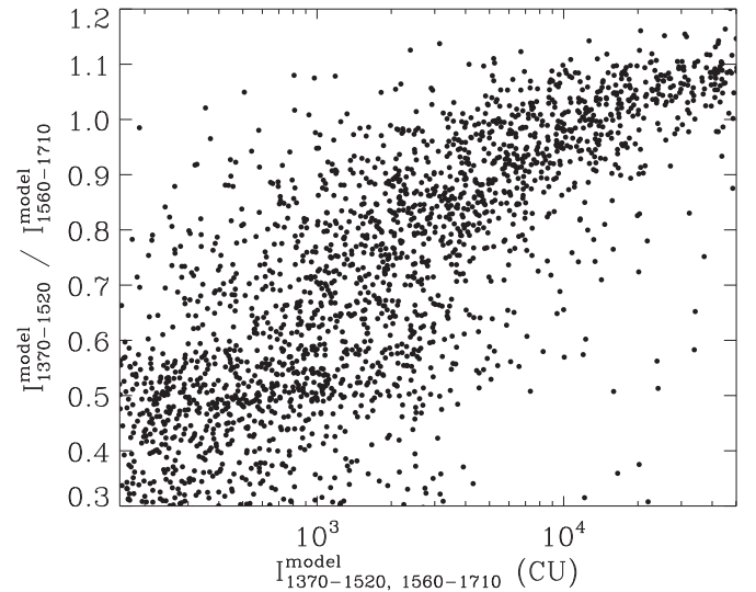
Figure 20. Stellar model prediction of hardness ratio (1370–1520 Å to 1560–1710 Å) vs. intensity (1370–1520, 1560–1660, and 1680–1710 Å). The Al II emission line was excluded in estimating the hardness ratio.
