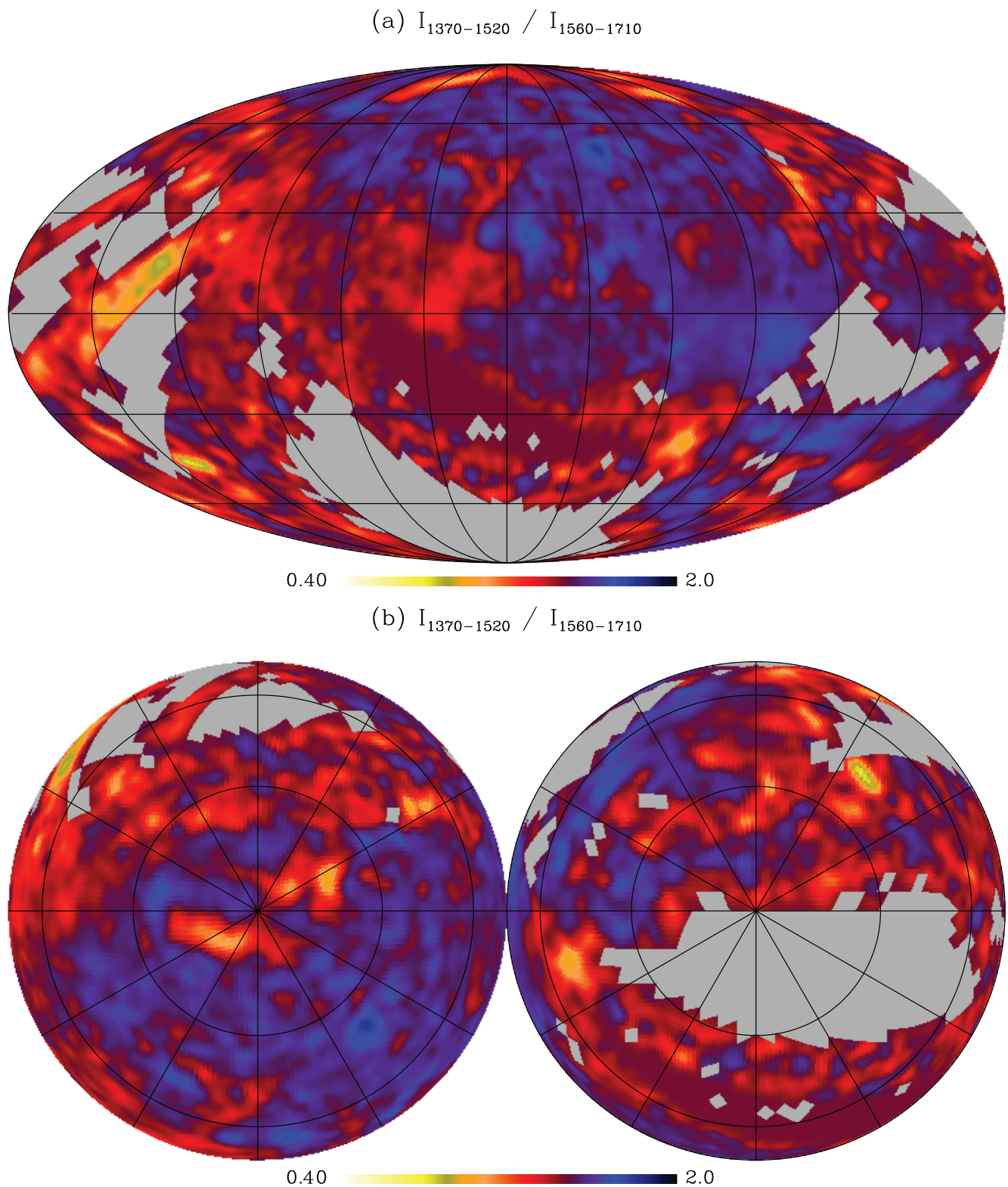
Figure 14. (a) Mollweide and (b) orthographic projections of the hardness ratio (1370–1520 Å to 1560–1710 Å) map. The Al II emission line was excluded in estimating the hardness ratio. The left and right sides of orthographic projections are centered at the northern and southern Galactic polar caps, respectively, and their longitude increases clockwise and counterclockwise, respectively. In both projections, l = 0^\circ is at the six o'clock position. The scales are linear across the color bars.
