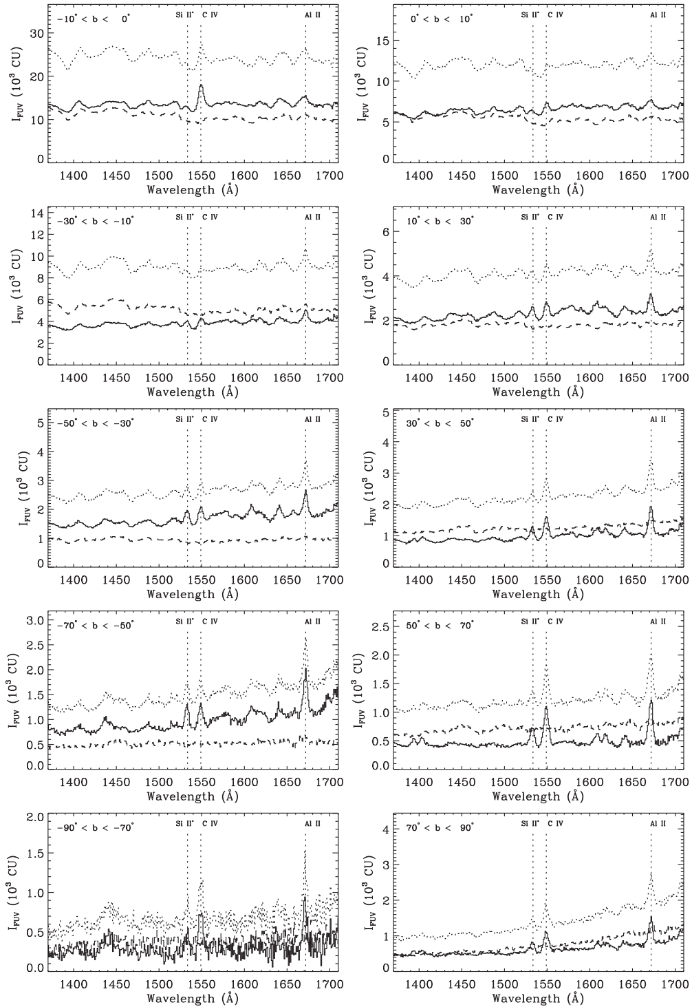
Figure 12. Average FUV spectra in various Galactic latitude ranges. Solid curve shows the diffuse FUV background spectrum. Dotted and dashed curves represent the total (direct stellar + diffuse) and the direct stellar spectra, respectively. Some important ionic lines are also indicated.
