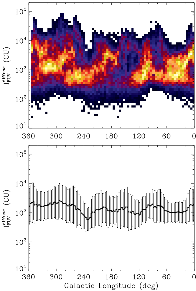
Figure 7. Diffuse FUV intensity vs. Galactic longitude. The top panel plots the two-dimensional histogram of the diffuse FUV intensity as a function of Galactic longitude. The bottom panel plots the median value within each of the 3^\circ longitude strips from the data. The vertical extent of each plotted bar is determined from the average deviation about the median within that bin. (A color version of this figure is available in the online journal.)
