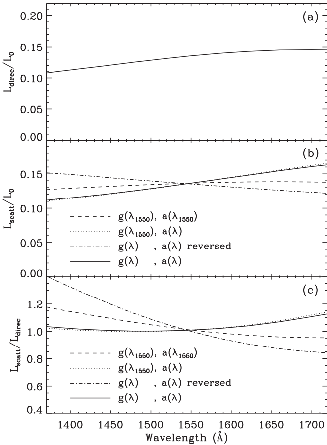
Figure 25. Scattering and absorption in a homogeneous dust medium. (a) The directly escaped and (b) scattered spectra relative to the input luminosity of the point source. (c) The scattered spectrum relative to the attenuated direct stellar spectrum. Here, various combinations of the wavelength dependences of the dust albedo and asymmetry factor are examined.
