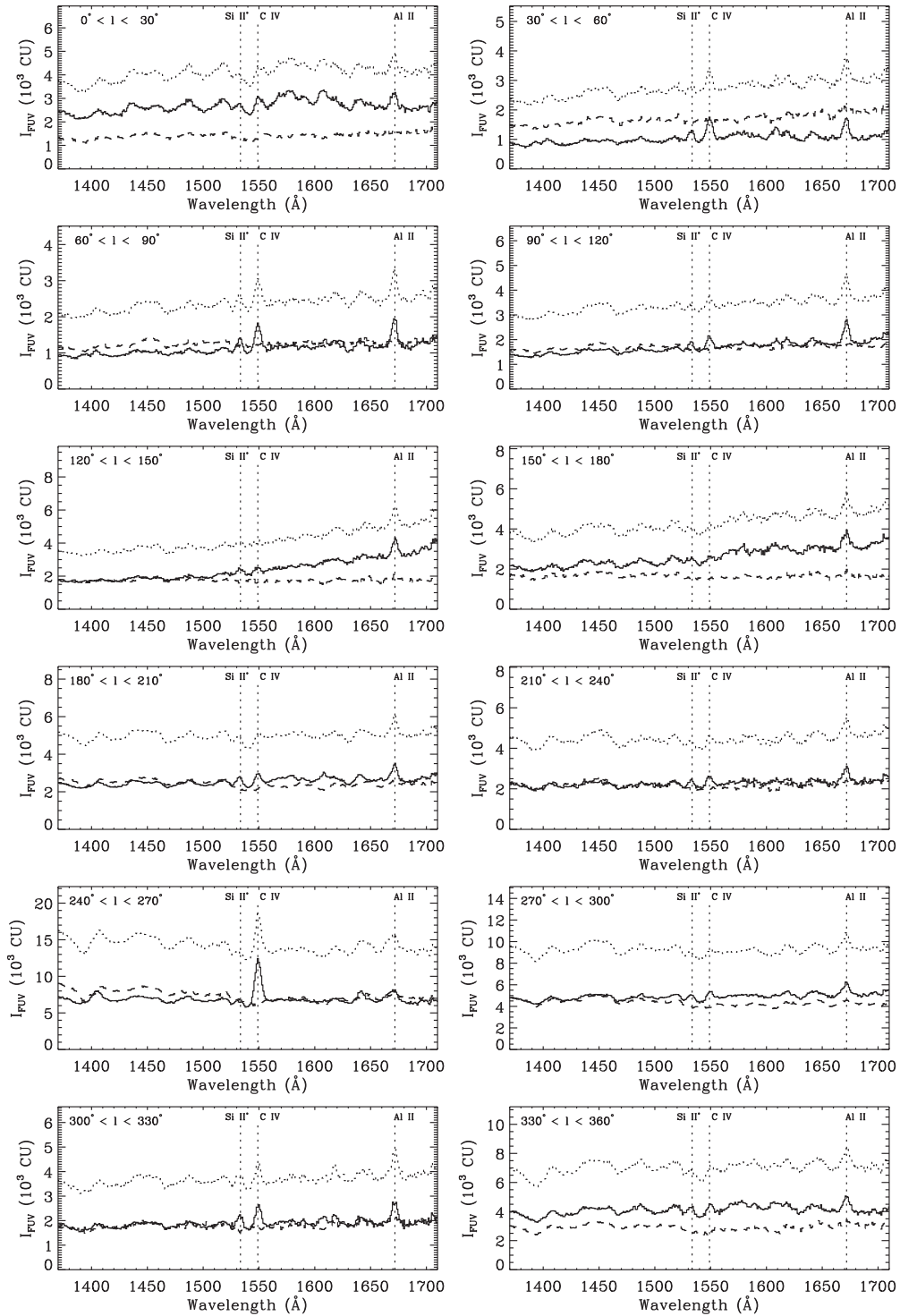
Figure 11. Average FUV spectra in various Galactic longitude ranges. Solid curve shows the diffuse FUV background spectrum. Dotted and dashed curves represent the total (direct stellar + diffuse) and the direct stellar spectra, respectively. Some important ionic lines are also indicated.
