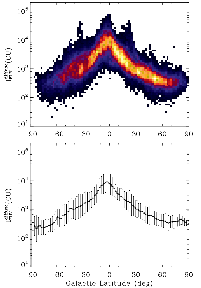
Figure 8. Diffuse FUV intensity vs. Galactic latitude. The top panel plots the two-dimensional histogram of the diffuse FUV intensity as a function of Galactic latitude. The bottom panel plots the median value within each of the 2^\circ latitude strips from the data. The vertical extent of each plotted bar is determined from the average deviation about the median within that bin. (A color version of this figure is available in the online journal.)
