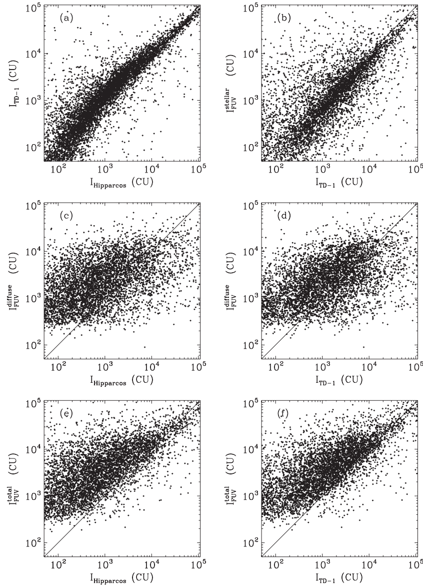
Figure 10. Comparison between the TD-1 stellar equivalent diffuse intensity (SEDI), the Hipparcos SEDI, and the SPEAR/FIMS intensities. (a) The TD-1 SEDI vs. the Hipparcos SEDI, (b) the direct stellar intensity observed with SPEAR/FIMS vs. the TD-1 SEDI, (c) the diffuse FUV background vs. the Hipparcos SEDI, (d) the diffuse FUV background vs. the TD-1 SEDI, (e) the total (direct stellar + diffuse) FUV intensity vs. the Hipparcos SEDI, and (f) the total FUV intensity vs. the TD-1 SEDI. Here, the resolution parameter N_{\text{side}} = 32 corresponding to angular resolution of \sim 1.8 is used. The TD-1 SEDI was estimated using the 1565 Å band, and the others were calculated over the same wavelength bands 1370–1520, 1560–1660, and 1680–1720 Å.
