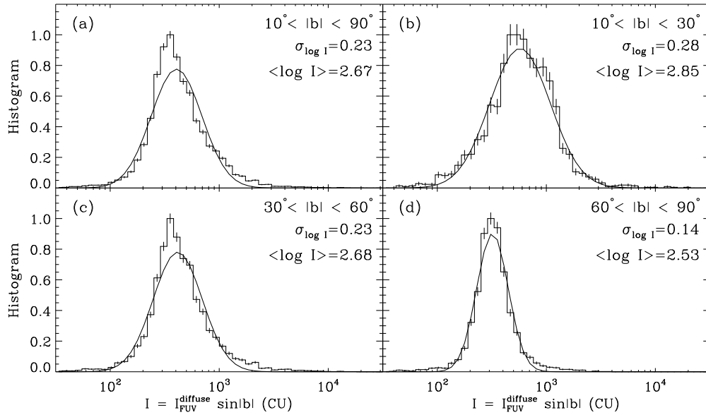
Figure 24. Histograms of I_{\text{FUV}}^{\text{diffuse}} \sin |b| in logarithmic scale. Log-normal fits are also shown. The standard deviations and the mean values of the distribution in logarithmic scale are also shown.
