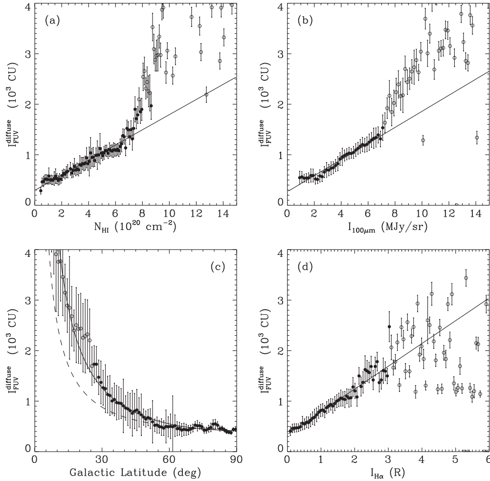
Figure 22. FUV intensity vs. (a) neutral hydrogen column density, (b) 100\,\mu\text{m} emission, (c) Galactic latitude, and (d) the \text{H}\alpha intensity. Best fits in (a), (b), and (d) are lines with (a) slope 1.49\,\text{CU}/(10^{18}\,\text{cm}^{-2}) , offset 271 CU, (b) slope 158\,\text{CU}(\text{MJy sr}^{-1})^{-1} , offset 243 CU, and (d) slope 456\,\text{CU}/\text{R} , offset 309 CU. Best-fit curves in (c) are 847\,\text{csc } |b| - 457\,\text{CU} for solid curve, and 412\,\text{csc } |b| - 457\,\text{CU} for dashed curve. Filled and hollow circles denote the data points, respectively, used and not used for the fit.
