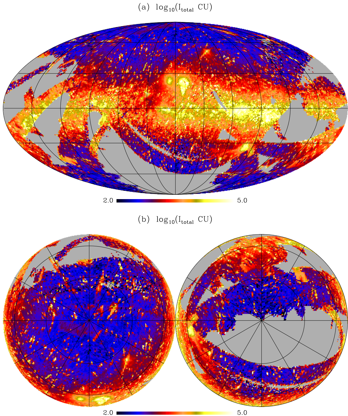
Figure 5. (a) Mollweide and (b) orthographic projections of the combined total (diffuse + direct stellar) FUV map observed with SPEAR/FIMS, after removal of the instrumental background. The left and right sides of orthographic projections are centered at the northern and southern Galactic polar caps, respectively, and their longitude increases clockwise and counterclockwise, respectively. In both projections, l = 0^\circ is at the six o'clock position. The intensity scales are logarithmic across the color bars. (c) Mollweide and (d) orthographic projections of signal-to-noise ratio of the total FUV map. The left and right sides of orthographic projections are centered at the northern and southern Galactic polar caps, respectively, and their longitude increases clockwise and counterclockwise, respectively. In both projections, l = 0^\circ is at the six o'clock position. The intensity scales are logarithmic across the color bars.
