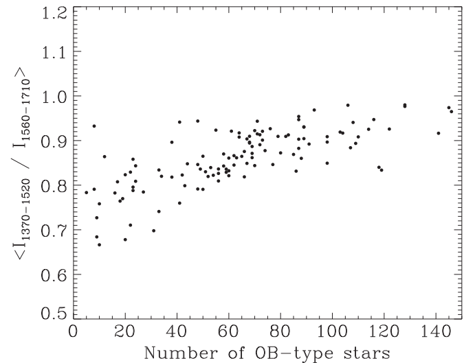
Figure 18. Correlation between the average hardness ratio (1370–1520 Å to 1560–1710 Å) and the number of OB-type stars. The average hardness ratio and the number of OB-type stars were calculated within each of the 3° longitude strips, and then the average hardness ratio vs. the number of OB-type stars was plotted. The Al II emission line was excluded in estimating the hardness ratio.
