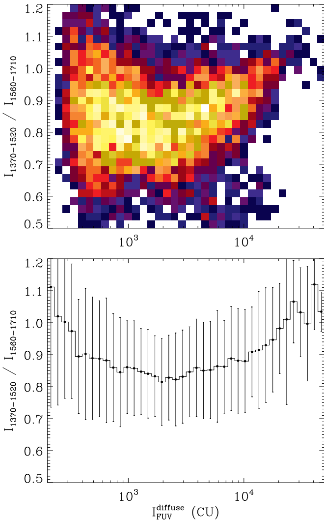
Figure 19. Hardness ratio (1370–1520 Å to 1560–1710 Å) vs. intensity (1370–1520, 1560–1660, and 1680–1710 Å). The Al II emission line was excluded in estimating the hardness ratio.
