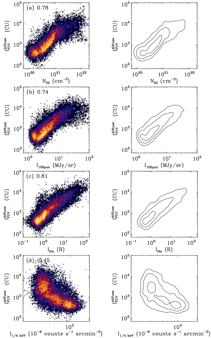
Figure 21. Correlation of the diffuse FUV background with (a) neutral hydrogen column density, (b) 100\,\mu\text{m} emission, (c) the diffuse \text{H}\alpha emission, and (d) soft X-ray ( 1/4\,\text{keV} band) background. The left panels show two-dimensional histogram and the right panels contours of the histograms. Numbers in the left panels are the correlation coefficients estimated in logarithmic scale. The contours correspond to 0.7, 0.3, and 0.1 of the maximum values of the histograms.
