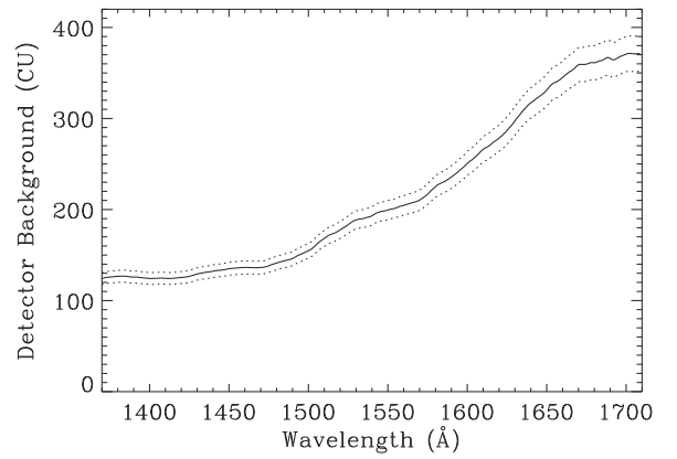
Figure 3. Instrumental background spectrum. The spectrum is essentially the inverse of the effective area curves, as shown in Edelstein et al. (2006a). A 1\sigma error range for the average of detector background value is also shown with dotted lines.
