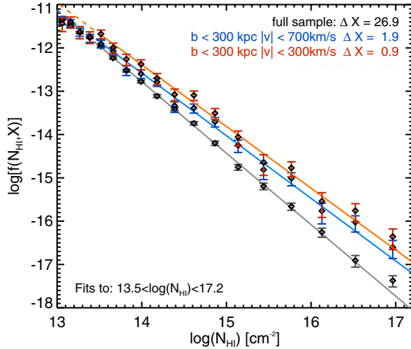
Figure 4. Same as Figure 2 but also considering the distribution of absorbers close to galaxies. The IGM distribution is shown in gray. Red points show the frequency of absorbers of a given N_{\text{H I}} within 300 km s ^{-1} and 300 pkpc of a galaxy in our spectroscopic sample. Blue points show the frequency of those within 700 km s ^{-1} and 300 pkpc. The curves are the maximum likelihood fits to the distributions over the range 13.5 < \log(N_{\text{H I}}/\text{cm}^{-2}) < 17.2 . The parameters of the fit are given in Table 4 along with the opacities calculated from the data and the opacities implied by the fit. Notably this single power law fit to the data does not well reproduce the opacities calculated from the data. Section 5.1 discusses broken power law fits which better reproduce these opacities. (A color version of this figure is available in the online journal.)
