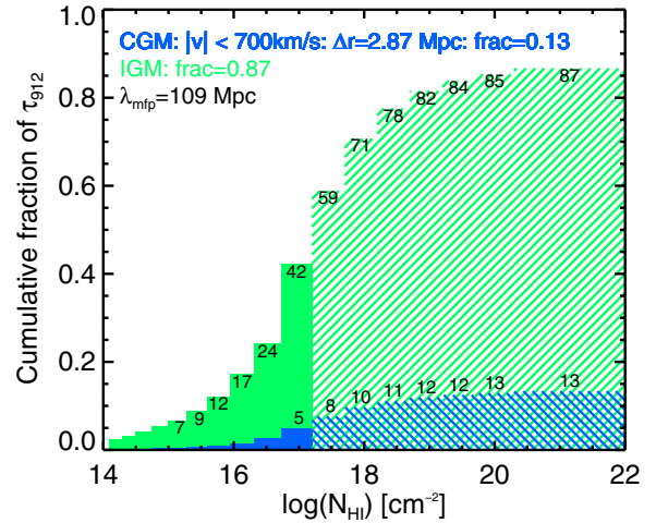
Figure 10. The cumulative fraction of the optical depth within 1 mean free path contributed by absorbers below a given N_{\text{HI}} in the IGM (green) or 700 \text{ km s}^{-1} CGM (blue). The solid histograms represent measurements from the data converted into an optical depth using Equations (12) and (15). The hatched histograms represent values from the fit to the data extrapolated to higher values of N_{\text{HI}} and then converted into an optical depth using Equations (12) and (14). The printed numbers give the percentage of the opacity due to absorbers with N_{\text{HI}} less than or within the N_{\text{HI}} bin.
