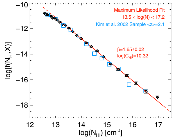
Figure 3. The frequency distribution of absorbers from the KBSS H I sample (black points) and the maximum likelihood fit to the data (red curve). For comparison, overplotted in (blue) squares are the data points from the \langle z \rangle = 2.1 sample from Kim et al. (2002). Because the analysis of the KBSS sample includes higher-order H I transitions, we can measure the frequency of absorbers with \log(N_{\text{H I}}/\text{cm}^{-2}) \gtrsim 14 with much higher fidelity than has been previously possible. Notably, there is no evidence for a strong break in the power law distribution near \log(N_{\text{H I}}/\text{cm}^{-2}) \approx 14 as has been previously suggested.
