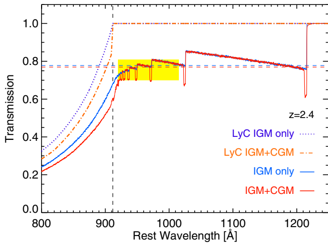
Figure 11. The average transmission spectra from 10,000 runs of the Monte Carlo simulations of IGM only (purple and blue) and IGM+CGM (red and orange) absorption in the foreground of a z = 2.4 emitter shown in the rest frame of the emitter. The solid (blue and red) curves show spectra using MC simulations that include line opacity. The dotted (purple) and dot-dashed (orange) curves show spectra from simulations only including continuum opacity. The highlighted yellow area marks the region between 920–1015 Å in the frame of the emitter which is used to renormalize the line opacity spectra in Figure 12. The dashed horizontal lines mark the average value of the transmission in this region, \langle 1 - D_B \rangle , for the spectra containing line opacity. The vertical dashed line marks the position of the Lyman limit in the frame of the emitter. The line absorption seen in the red spectrum is due to the Lyman series line opacity from high- N_{\text{H I}} CGM absorbers.
