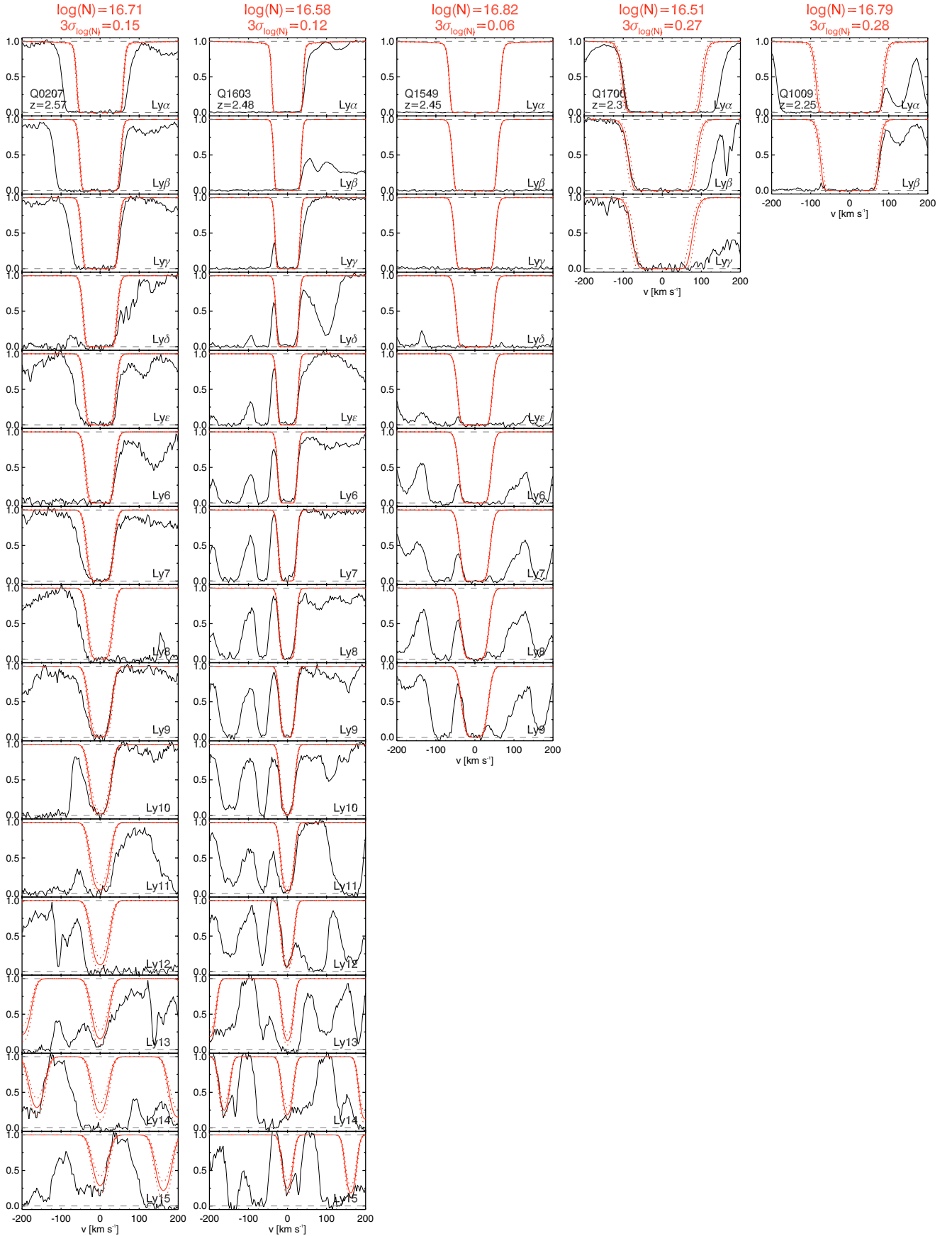
Figure 18. Example fits to absorbers with 16.5 < \log(N_{\text{H I}}/\text{cm}^{-2}) < 17.0 . The black curves show the HIRES data. Gray dashed lines mark the zero point and continuum of the QSO spectra. The solid red curve shows the best fit Voigt profile to each absorber. The dashed red curves show the formal \pm 3\sigma N_{\text{H I}} error. (A color version of this figure is available in the online journal.)
