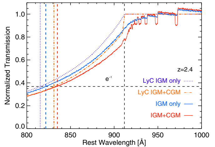
Figure 12. The average normalized transmission below the Lyman limit of a z = 2.4 emitter. The red and orange curves pertain to transmission including the CGM and the blue and purple curves pertain to IGM only transmissions. The dotted (purple) and dot-dashed (orange) lines show the same spectra as in Figure 11 from the continuum opacity only runs of the MC code. The solid (red and blue) curves show the spectra including line opacity normalized by (1 - D_B) . The black vertical dashed line marks the position of the Lyman limit in the frame of the emitter. The dashed horizontal line shows where the normalized transmission is equal to e^{-1} . The colored vertical lines mark the position where each of the spectra crosses the e^{-1} , signifying the position of one \lambda_{\text{mfp}} . These rest wavelengths are converted into physical distances corresponding to the \lambda_{\text{mfp}} as described in the text.
