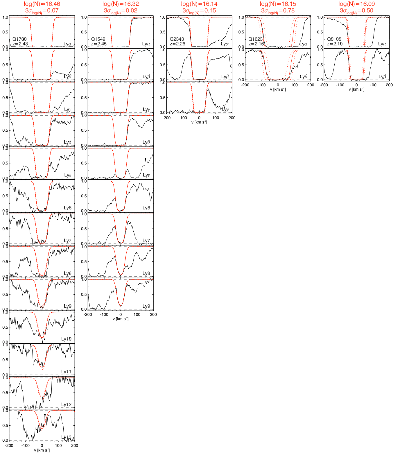
Figure 17. Example fits to absorbers with 16.0 < \log(N_{\text{H I}}/\text{cm}^{-2}) < 16.5 . The black curves show the HIRES data. Gray dashed lines mark the zero point and continuum of the QSO spectra. The solid red curve shows the best fit Voigt profile to each absorber. The dashed red curves show the formal \pm 3\sigma N_{\text{H I}} error. (A color version of this figure is available in the online journal.)
