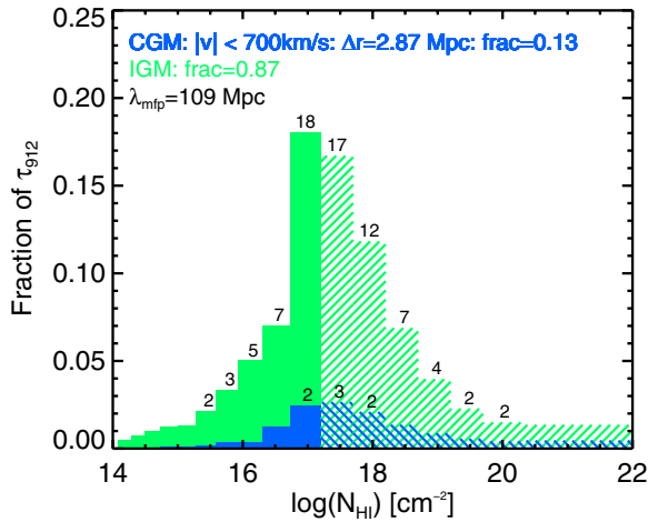
Figure 9. The fraction of the optical depth within 1 mean free path contributed by absorbers within a given bin of N_{\text{HI}} in the IGM (green) or 700 \text{ km s}^{-1} CGM (blue). The solid histograms represent measurements from the data converted into an optical depth using Equations (12) and (15). The hatched histograms represent values from the fit to the data extrapolated to higher values of N_{\text{HI}} and then converted into an optical depth using Equations (12) and (14). The printed numbers give the percentage of the opacity due to that N_{\text{HI}} bin.
