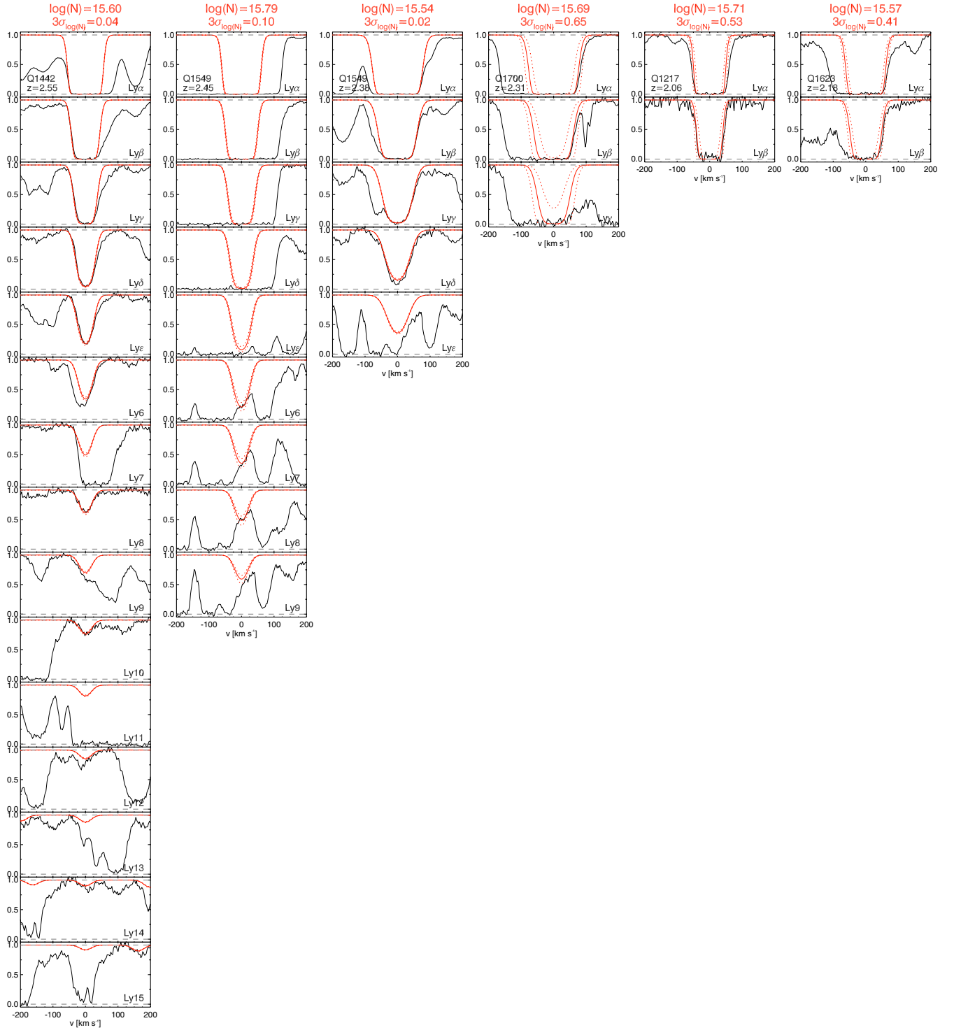
Figure 16. Example fits to absorbers with 15.5 < \log(N_{\text{H I}}/\text{cm}^{-2}) < 16.0 . The black curves show the HIRES data. Gray dashed lines mark the zero point and continuum of the QSO spectra. The solid red curve shows the best fit Voigt profile to each absorber. The dashed red curves show the formal \pm 3\sigma N_{\text{H I}} error. (A color version of this figure is available in the online journal.)
