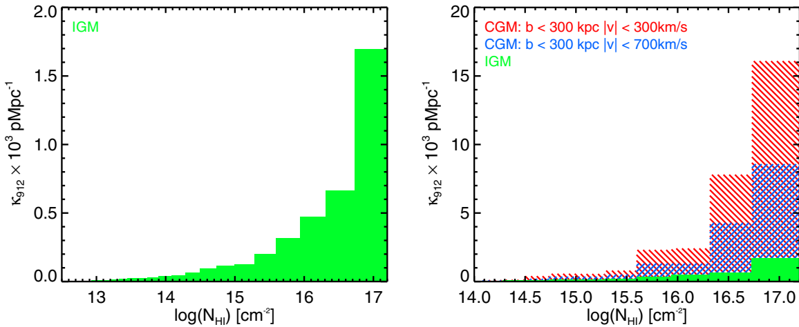
Figure 5. Contributions to the opacity from a given bin in N_{\text{HI}} , measured directly from the data using Equation (15). Left: the IGM opacity per bin in N_{\text{HI}} . Right: the opacity per bin in N_{\text{HI}} within the IGM (green), the 700 \text{ km s}^{-1} CGM (blue) and the 300 \text{ km s}^{-1} CGM (red). Note that the scale of the left-hand panel is 10% of the scale of the right-hand panel. The opacity (optical depth per unit physical distance) of the CGM is an order of magnitude larger than the average opacity in the IGM. (A color version of this figure is available in the online journal.)
