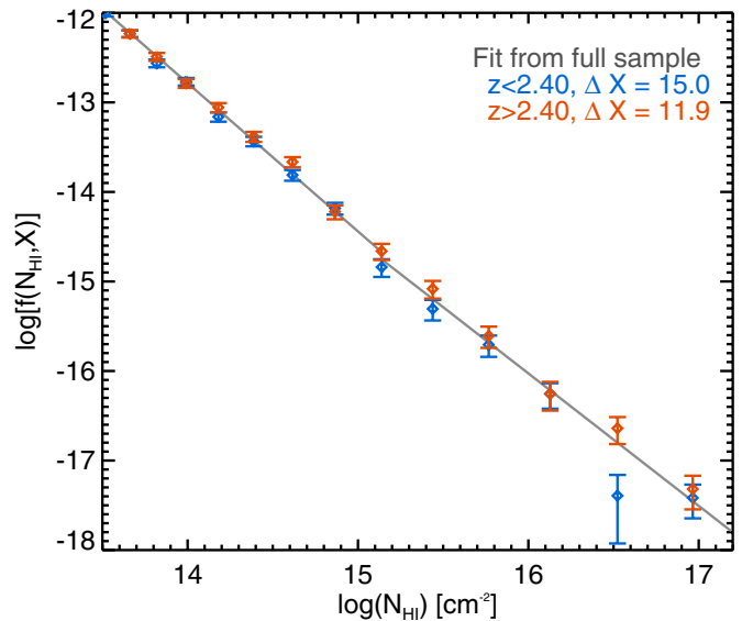
Figure 19. The frequency distribution measured from the higher-redshift (red) and lower-redshift (blue) portions of the absorber sample (many of the points from the two subsamples lie on top of each other). The gray curve shows the broken power law fit to the full absorbers sample from Section 5.1.
