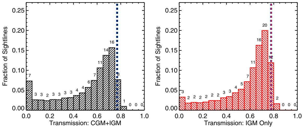
Figure 14. The distribution of transmissions from each sight line averaged over the band pass from 880–910 Å for the IGM+CGM Monte Carlo simulations (left panel) and IGM only Monte Carlo simulations (right panel) that include line opacity. The simulations used for these figures are those with an emission redshift of z = 2.4 . The (blue) dashed vertical line marks the average transmission in the Ly \beta , \gamma , + forest \langle 1 - D_B \rangle . (A color version of this figure is available in the online journal.)
