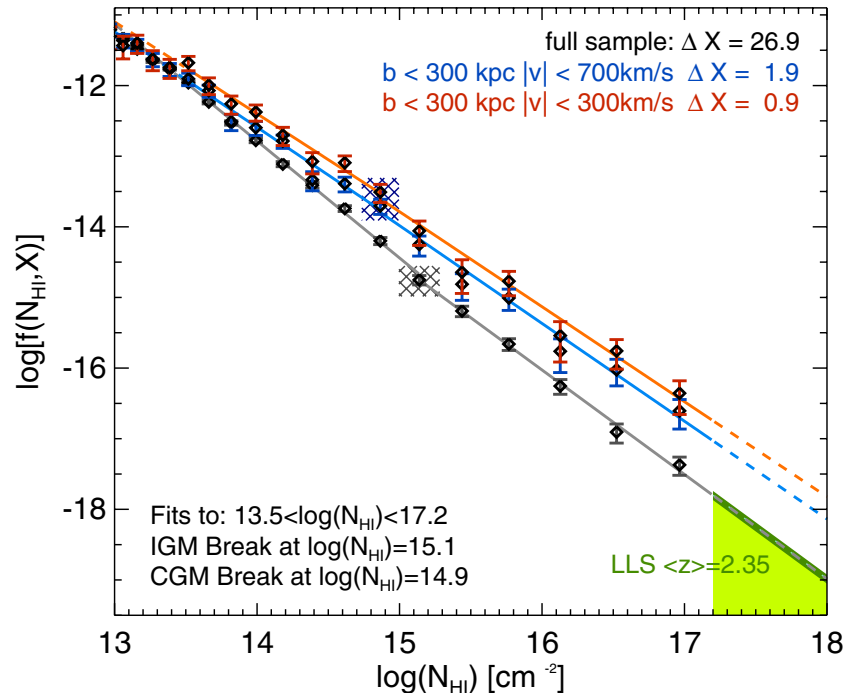
Figure 6. Broken power law least-squares fits to the binned IGM (gray) and CGM (blue and red) data. The slopes and normalizations for each data set (IGM or CGM) are allowed to vary independently; however, both ranges include the data point centered at the break (shaded regions). Note that the broken power law fit is discontinuous at the break location. Including one data point in both ranges minimizes the discontinuity associated with the break and produces a better fit to the data. The hatched box shows the range of N_{\text{HI}} included in that point and thus in both fits. The green triangle represents the measured incidence of LLSs as discussed in Section 3.3. The parameters of the fit are given in Table 5 along with the opacity calculated from the data and the opacity produced by the fit to the distribution. Note that the opacity is reproduced to much higher fidelity using the broken power law fit.
