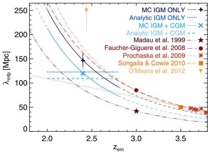
Figure 15. The \lambda_{\text{mfp}} as a function of z_{\text{em}} including previous estimates of the \lambda_{\text{mfp}} from the literature. The blue points and curves refer to values measured in this paper whereas estimates from the literature are plotted in shades of red. The blue cross and X and their corresponding curves show the values of \lambda_{\text{mfp}} calculated from the MC spectra for the IGM ONLY and IGM+CGM runs respectively. The dotted and dashed blue horizontal line show the results of the analytic calculation in Section 5 excluding and including the CGM respectively. The dark red filled star and the dash-dotted curve that intersects it are the suggested values of \lambda_{\text{mfp}} from Madau et al. (1999). The red filled circle and dashed curve are the results of Faucher-Giguère et al. (2008). Prochaska et al. (2009) suggested the values shown with the red/orange asterisks and the dotted line. The measurements of Songaila & Cowie (2010) are shown in the orange filled square and the dash-dotted curve that intersects it. The results of O’Meara et al. (2013) are shown in the orange filled triangle.
