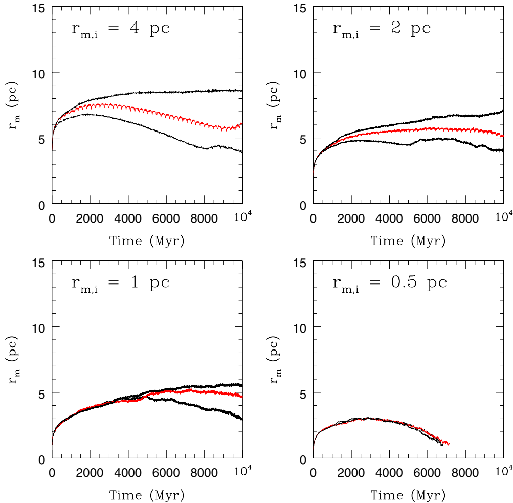
Figure 7. Evolution of half-mass radius over time. The upper left, upper right, lower left, and lower right panels are for simulations with initial half-mass radii of 4 pc, 2 pc, 1 pc, and 0.5 pc, respectively. The red lines correspond to models with orbital eccentricities of 0.5, while the lower black lines correspond to a cluster with a circular orbit at perigalacticon (6 kpc) and the upper black lines correspond to a cluster with a circular orbit at apogalacticon (18 kpc).
