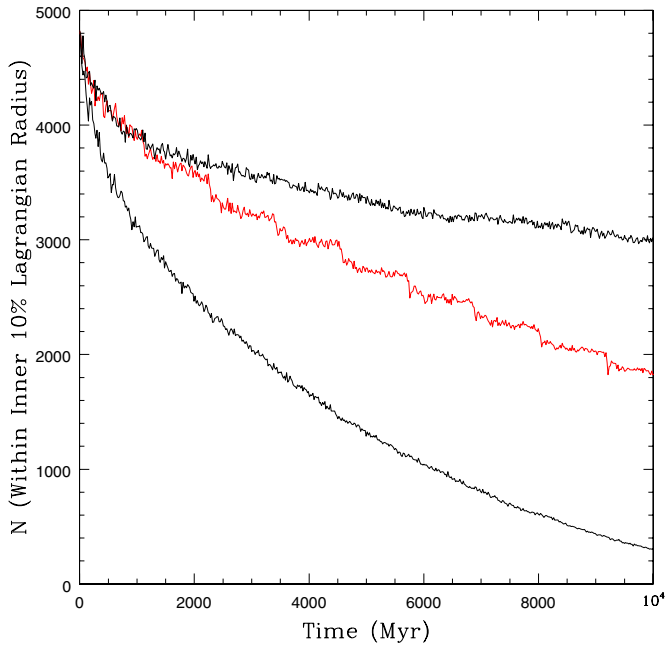
Figure 10. Evolution of the number of stars within the inner 10% Lagrangian radius over time. The red line correspond to the e = 0.9 model (e09r104b). The lower black line corresponds to a cluster with a circular orbit at perigalacticon (6 kpc), while the upper black line corresponds to a cluster with a circular orbit at apogalacticon (104 kpc). The number of stars within the inner 10% Lagrangian radius will naturally decrease over time due to two-body encounters; however, the eccentric case (red line) illustrates that with each perigalactic pass a significant number of stars move beyond the inner 10% Lagrangian radius.
