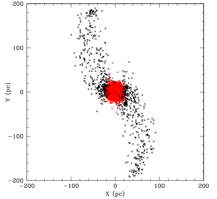
Figure 2. Snapshot of a model cluster on a circular orbit at 6 kpc after 32 orbits (5680 Myr). Bound stars are marked in red.
