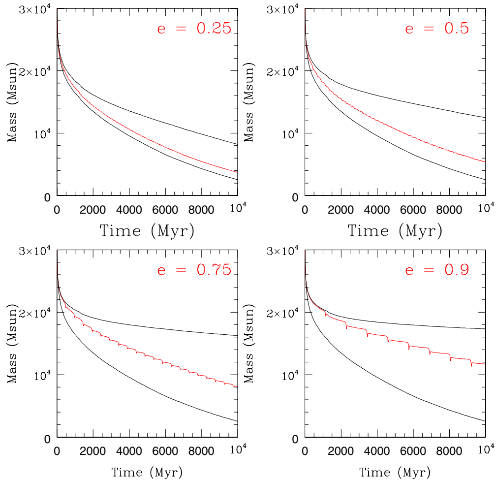
Figure 3. Evolution of total cluster mass over time. The red lines correspond to models with orbital eccentricities as labeled in each panel. In each plot, the lower black line corresponds to a cluster with a circular orbit at perigalacticon (6 kpc), while the upper black line corresponds to a cluster with a circular orbit at apogalacticon. (A color version of this figure is available in the online journal.)
