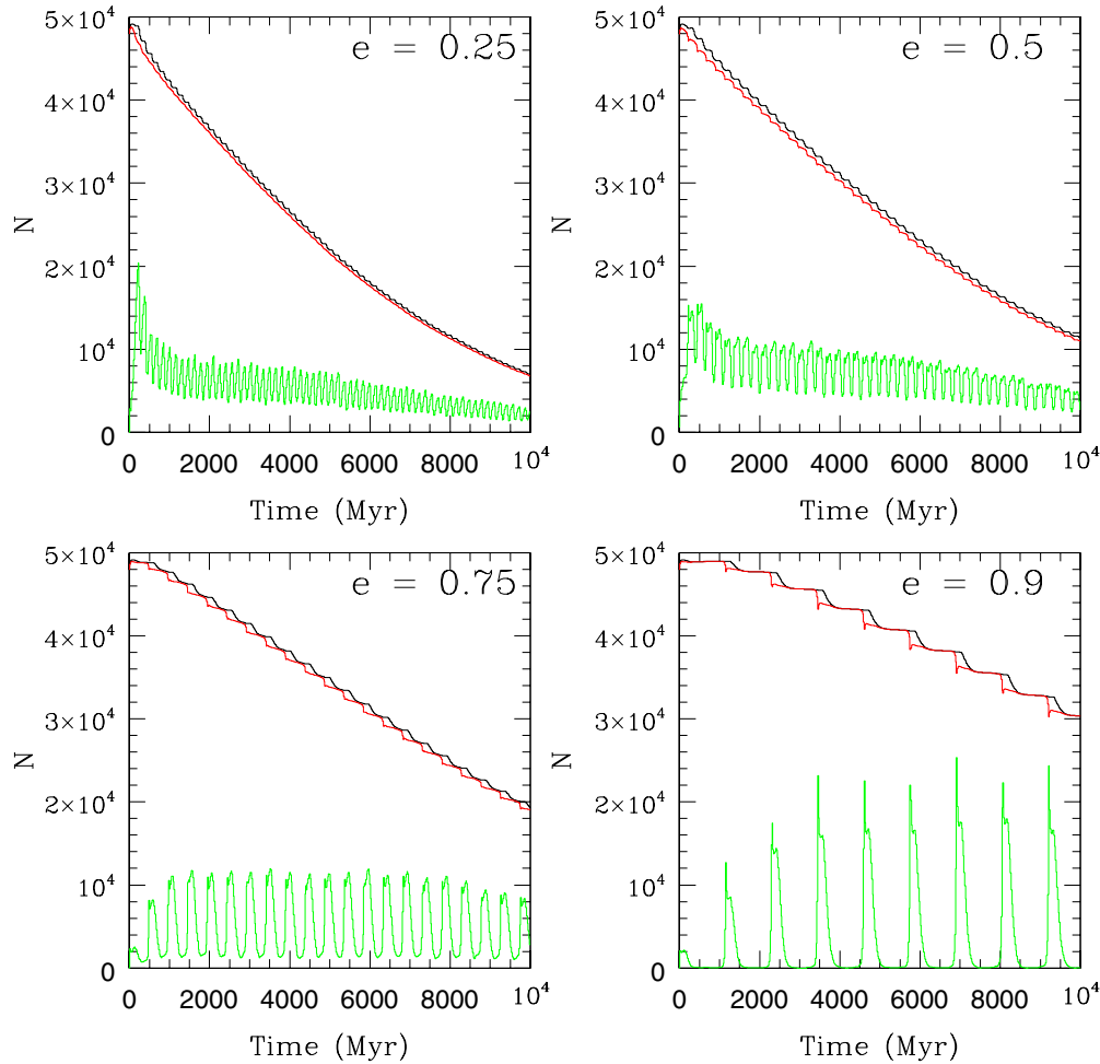
Figure 9. Total number of bound (red) and unbound (green) stars in a cluster as a function of time. The black line corresponds to the total number of stars and the orbital eccentricity of the model is labeled in each panel. For comparison purposes, the number of unbound stars has been increased by a factor of 10.
