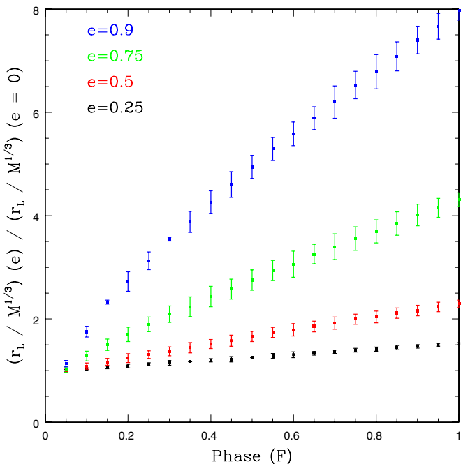
Figure 11. Ratio of the mass normalized limiting radius of model clusters with eccentric orbits to the mass normalized limiting radius of a cluster with a circular orbit at perigalacticon as a function of orbital phase as defined in Equation (7). Error bars represent an uncertainty of 1\sigma .
