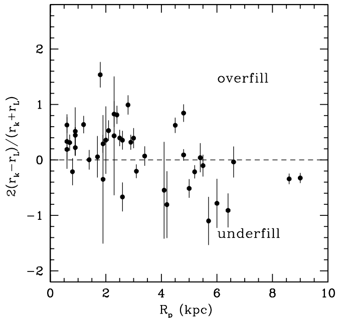
Figure 12. Ratio of difference between fitted King (1962) radius ( r_k ) and limiting radius ( r_L ) to the average of the two radii vs. perigalactic distance for Galactic globular clusters. Limiting radii have been calculated based on the orbital eccentricity and phase of a cluster as given by Equation (8).
