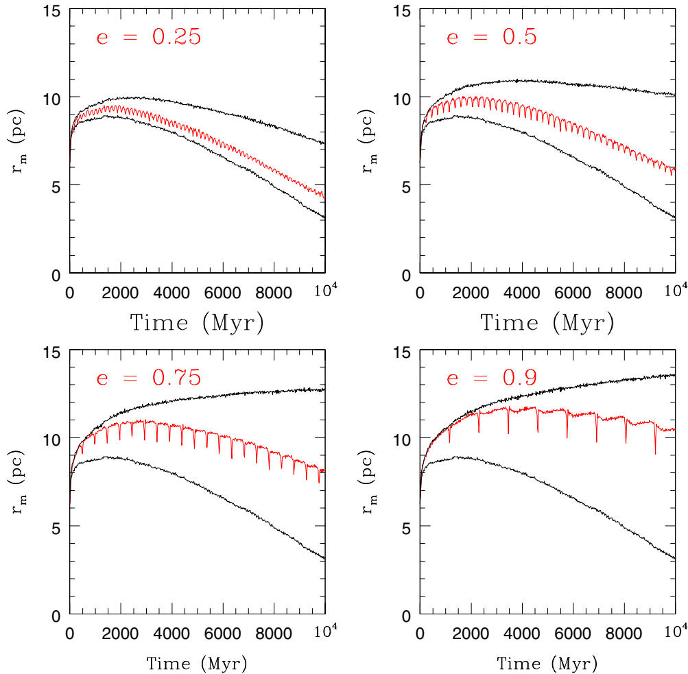
Figure 4. Evolution of half-mass radius over time. The red lines correspond to models with orbital eccentricities as labeled in each panel. In each plot, the lower black line corresponds to a cluster with a circular orbit at perigalacticon (6 kpc), while the upper black line corresponds to a cluster with a circular orbit at apogalacticon. (A color version of this figure is available in the online journal.)
