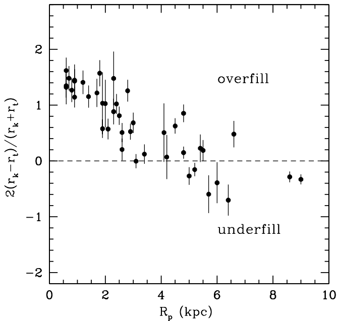
Figure 1. Ratio of difference between observed ( r_k ) and theoretical ( r_t ) tidal radius at perigalacticon to the average ((r_t + r_k)/2) vs. perigalactic distance for Galactic globular clusters.
