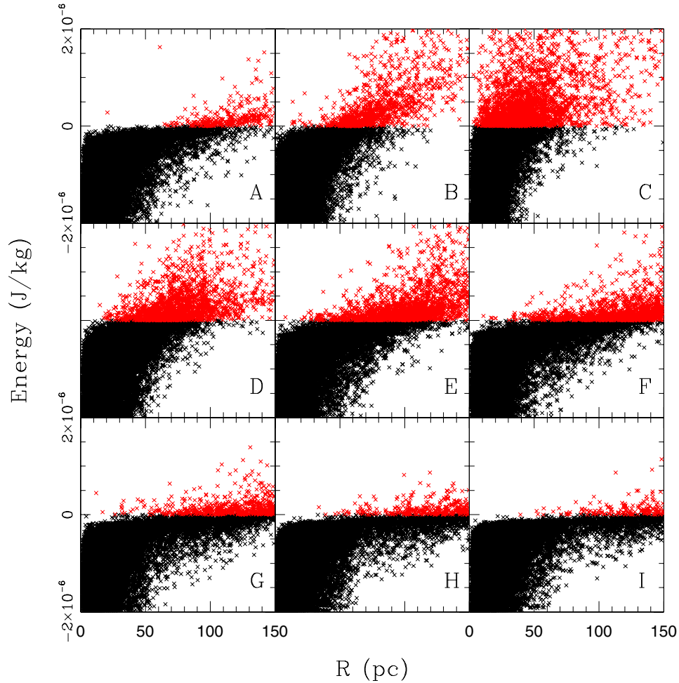
Figure 8. Radial distance and energy of stars within model cluster e09r104rm6 for different time steps. Beginning in Panels (A) and (B) the cluster is travelling toward perigalacticon. In Panel (C) the cluster has just left perigalacticon. In Panels (D)–(I) the cluster is moving away from perigalacticon. Bound stars are marked as black and unbound stars are marked as red.
