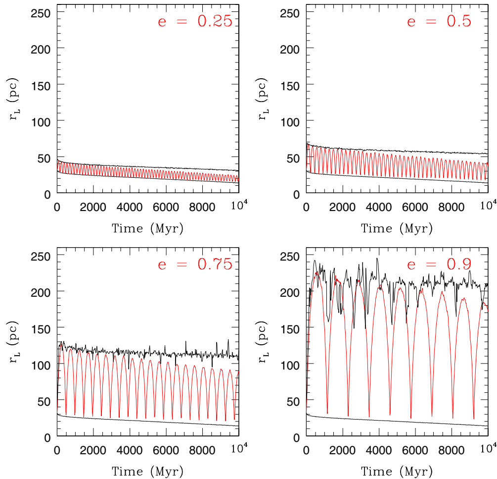
Figure 6. Evolution of the limiting radius over time. The red lines correspond to models with orbital eccentricities as labeled in each panel. In each plot, the lower black line corresponds to a cluster with a circular orbit at perigalacticon (6 kpc), while the upper black line corresponds to a cluster with a circular orbit at apogalacticon. (A color version of this figure is available in the online journal.)
