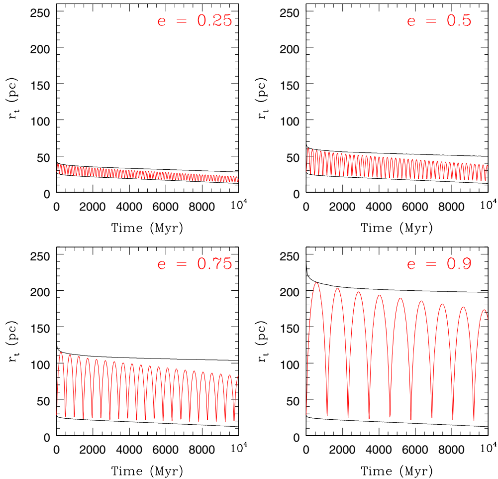
Figure 5. Evolution of the instantaneous tidal radius over time. The red lines correspond to models with orbital eccentricities as labeled in each panel. In each plot, the lower black line corresponds to a cluster with a circular orbit at perigalacticon (6 kpc), while the upper black line corresponds to a cluster with a circular orbit at apogalacticon.
