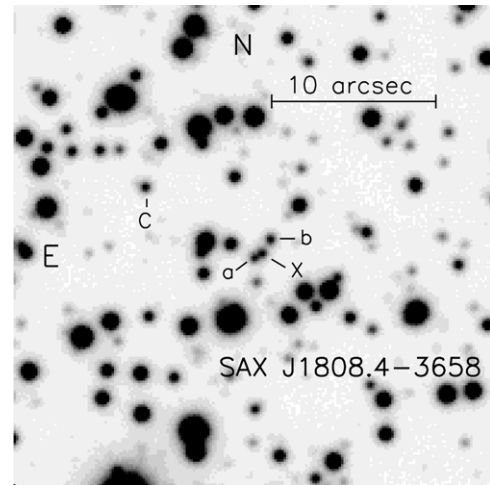
Figure 2. Gemini South r' image of the J1808.4 field. Object X, located between stars a and b , is the optical counterpart to J1808.4. The star labeled as C is used as a check star.
