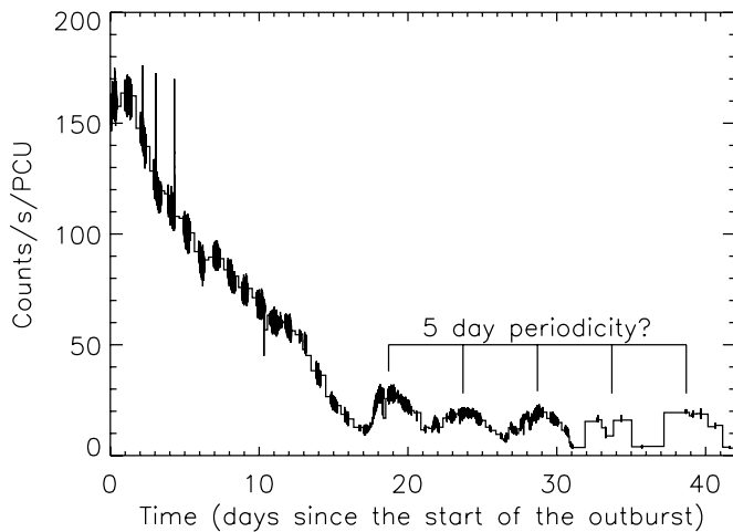
Figure 1. X-ray light curve of J1808.4 during its 2002 outburst, obtained with the proportional counter array (PCA; 2–60 keV energy range) on board the Ross X-ray Timing Explorer satellite. Gaps in the light curve were due to Earth occultations of the source. At the end of the outburst, a \sim 5 day periodicity is tentatively suggested.
