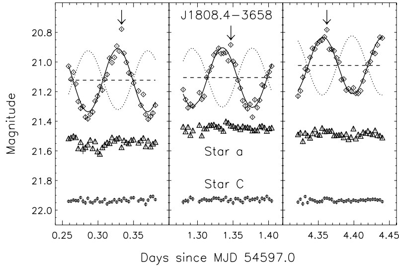
Figure 3. Optical r' light curves of J1808.4 (diamonds), in which sinusoidal modulation is clearly visible. For comparison, the LCs of the nearby star a (triangles) and check star C (circles, downward shifted by 0.8 mag) are also shown. The best-fit sinusoidal function to the LCs of J1808.4 is shown as the solid curves, while the constant magnitude for each LC is indicated by the dashed lines. The optical periodicity well matches the X-ray ephemeris (dotted curves), which gives the mean orbital longitude of the binary (Hartman et al. 2008). The optical brightness peaks correspond to when the pulsar is right in front of the companion star ( 270^\circ mean orbital longitude). The brightest data points in the LCs, indicated by arrows, are at phase 0.05–0.17 after the maxima of the sinusoid.
