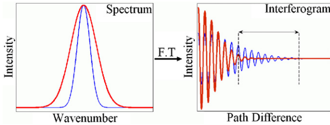
Figure 1. Left: two spectral features with a common central wavenumber and different widths. Right: the interferogram of both spectral features with the chosen part for differentiating the sharper narrow feature.
