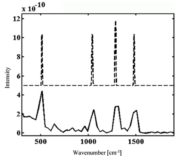
Figure 3. The bio-signature used before the addition of noise (above) and that reconstructed from the selected region of the interferogram with photon noise.
