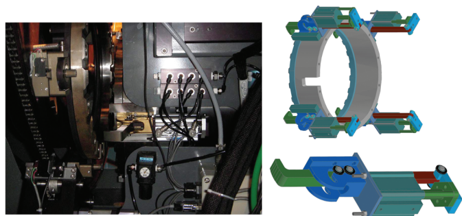
FIG. 29.—The clamping mechanism of the disperser server system. The photo shows, on the far left, the motor and drive train for the DSS wheel. Left of center, in the foreground, is an index ring mounted to the back of a GTM—this unit is one position off in rotation from the receiving ring in the pupil ( background ). One of the clamps is seen in the open receiving position. The solid models on the right show the detail of one clamp and the arrangements of all four clamps that allow IMACS to pull a disperser unit free of the DSS wheel and clamp it to the MOSS structure.
