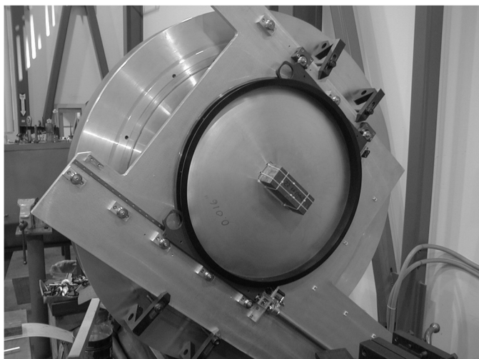
FIG. 25.—Mask server, early in the design development phase. The mask assembly consists of a C-channel hoop that holds the mask and two opposing wings that attach to the hoop. The beveled straight edge on each wing engages with the V-roller wheels to guide the mask assembly between the mask cassette and the in-beam position. In the lower half of the image, the air-cylinder insertion actuator and linear bearing guide are visible. This picture shows the testing of the mechanism under varying gravity orientations, using a gap bed lathe in the Carnegie shop to rotate the unit (this test was done prior to the assembly of the main structure and carriage). The large weight at the center of the mask simulated the estimated mass and center of gravity of the Durham IFU, which was much heavier than a single multislit-mask assembly.
