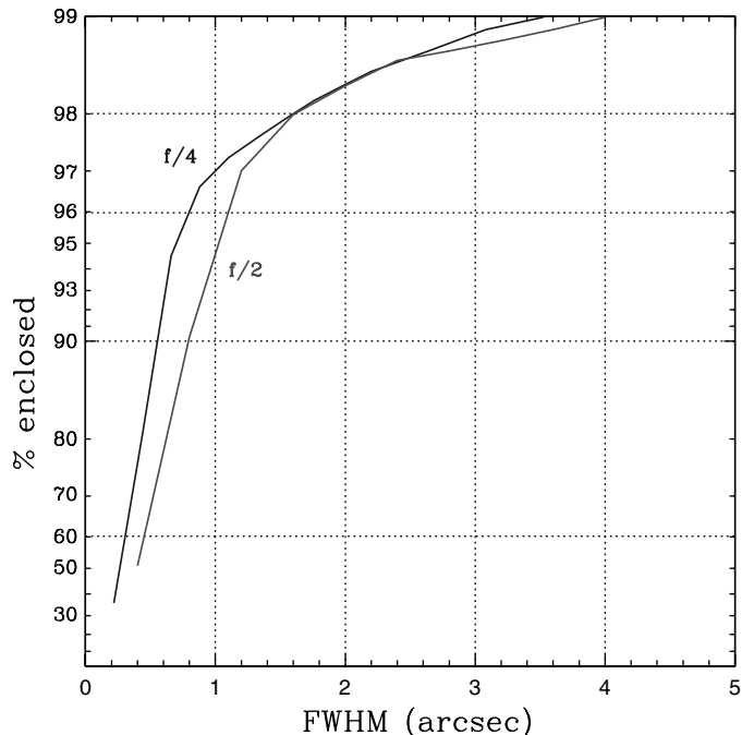
FIG. 19.—The point-spread function for the f/2 and f/4 channels of IMACS. The data show the wings in the light profile of 0.30'' FWHM ( f/4 ) and 0.35'' FWHM ( f/2 ). For both channels, 2% of the light scatters to a diameter greater than 1.5'' , with 1% outside of a 3.5'' diameter.
