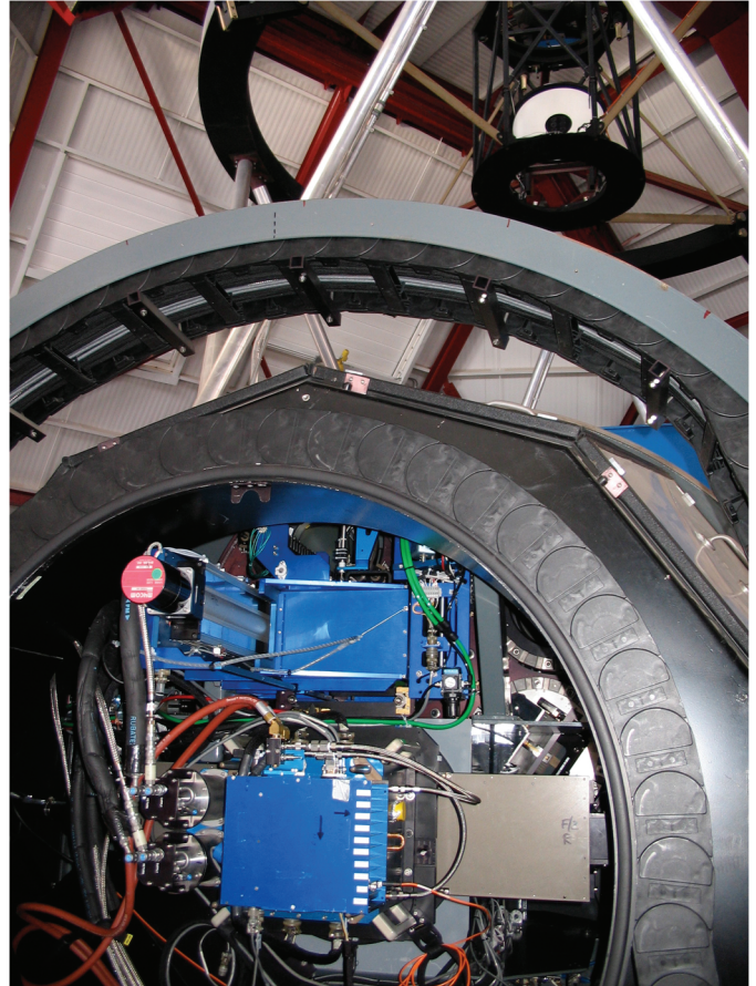
FIG. 23.—Rear view of IMACS, showing some f/2 components. Inside the inner race of the utility wrap is the f/2 filter server ( top )—motor and stage to the left. The Mosaic-2 CCD camera is behind the blue electronics box in the center, with CryoTiger heads on the left and one side of the f/2 shutter to the right. Two index rings at the back of the dispersers are visible above the shutter. A large circular enclosure panel covers this whole area. Above the outer race of the utility wrap the Baade telescope structure and dome can be seen. The small black ring is the bottom of the cage of Gregorian secondary mirror, visible at top. The white doughnut is the pupil screen that is illuminated for flat-field observations, seen in its retracted position.
