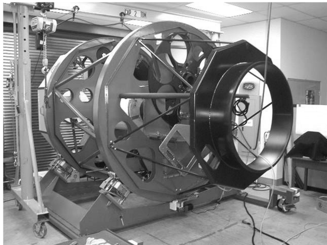
FIG. 21.—An early stage of assembly of IMACS in the Carnegie Observatories shops. This photo shows the carriage, with its self-steering rollers supporting the rotating part of the IMACS structure assembly. The rotating assembly consists of two monocoque disks connected by the main truss, the secondary truss ( black ) supporting the cantilevered rotating portion of the utility wrap, and the MOSS. Also visible in the photo is the primary structure ( wheel ) of the disperser server that carries the spectrograph dispersers and accessories.
