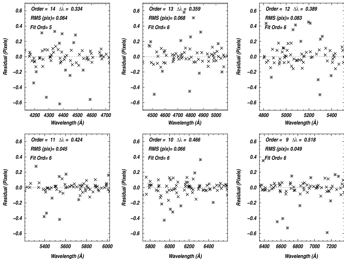
FIG. 6.—Example of the QA plots produced during 1D wavelength calibration. Plotted in each panel are the residuals (in pixels) as a function of wavelength, for each order. The black crosses correspond to ThAr emission lines that were used in the final fit, and asterisks are lines that were rejected. The order number, rms (in pixels), dispersion ( \text{\AA pixel}^{-1} ), and polynomial order is reported for each panel. Note that the typical rms is less than 0.1 pixels and usually is \sim 0.05 pixels. See the electronic edition of the PASP for a color version of this figure.
