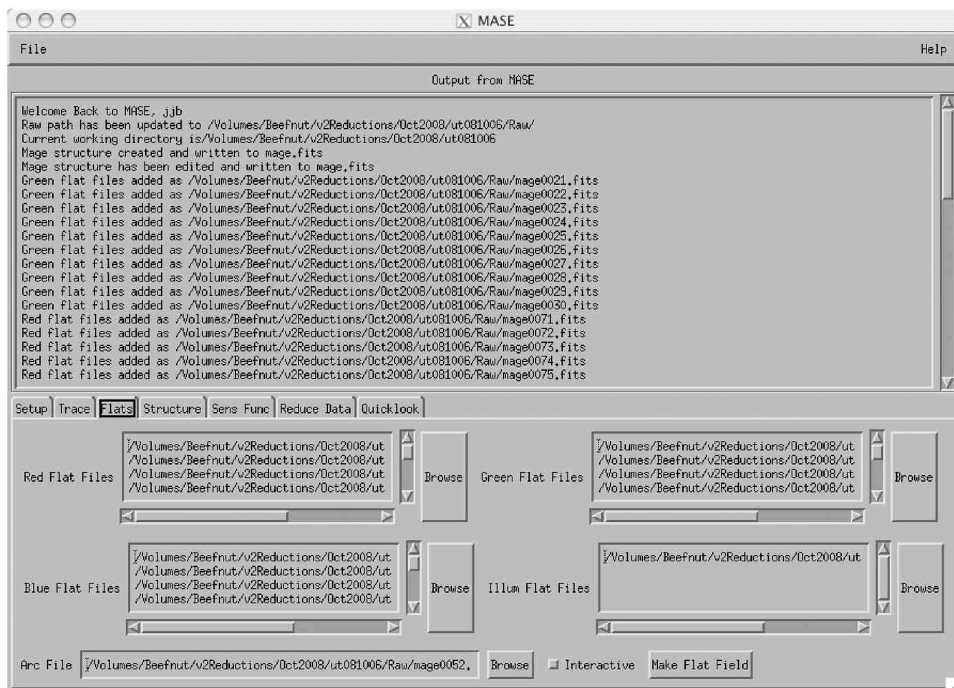
FIG. 2.—MASE GUI. It is composed of the message window and tabs. The message window, located in the upper part of the GUI, provides feedback and confirmation of user actions. Underneath the message window, the tabs separate the major steps in the calibration process and allow the user to select which files are calibrated and reduced. The Flats tab is shown in this example.
