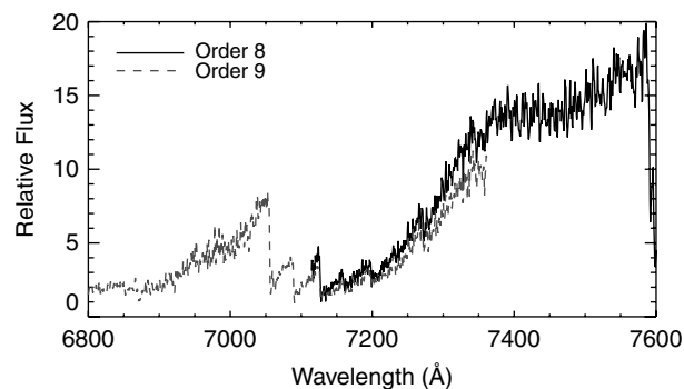
FIG. 10.—Relative flux of an M dwarf observed with MAGE between two adjacent orders (8 and 9, solid line and dashed line, respectively). Note that the agreement between orders is very good, typically to within 5%. See the electronic edition of the PASP for a color version of this figure.
