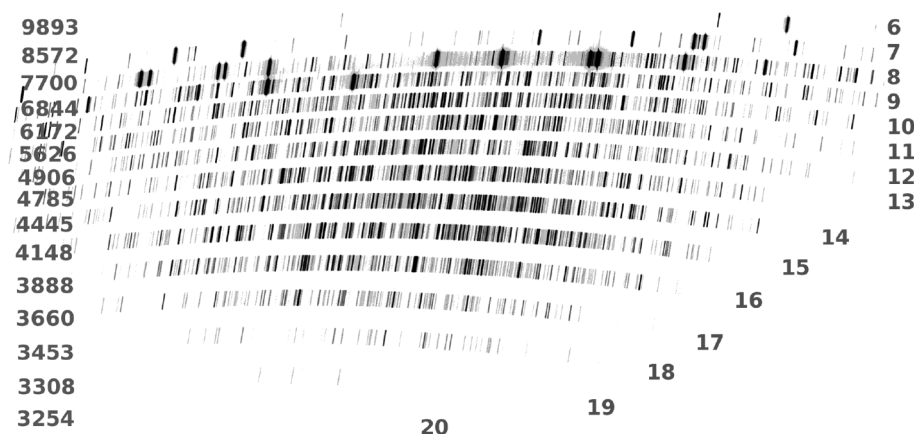
FIG. 5.—Example of a Th-Ar arc spectrum. Note the dearth of emission lines in the reddest and bluest orders. See the electronic edition of the PASP for a color version of this figure.
