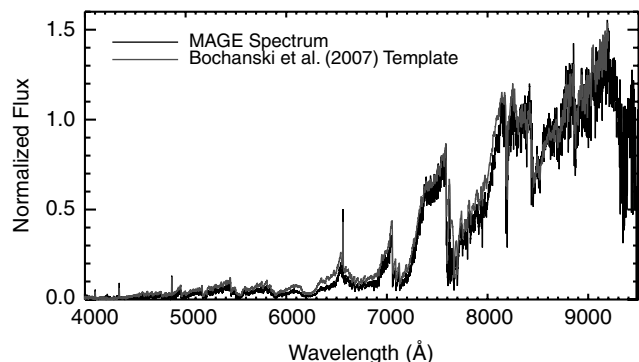
FIG. 9.—Comparison between a reduced MAGE spectrum of an M7 dwarf (black line) and the corresponding SDSS template spectra (gray line; Bochanski et al. 2007). Note the fairly good agreement in the flux calibration between the two objects over the wavelength range shown, despite residual telluric absorption in the MAGE spectrum. Future versions of MASE will include a telluric correction. See the electronic edition of the PASP for a color version of this figure.
