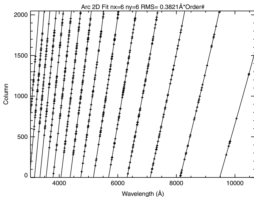
FIG. 7.—Example of the QA plots produced during 2D wavelength calibration. The line is the 2D Chebyshev polynomial fit, and the crosses are the individual line centers, shown as a function of column ( x pixel position) and wavelength. This step improves the accuracy in orders with few Th-Ar lines, such as order 6 (the rightmost order). See the electronic edition of the PASP for a color version of this figure.
