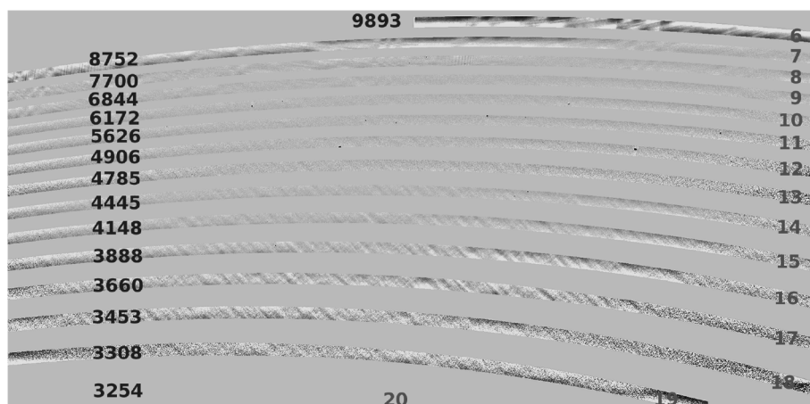
FIG. 4.—Example of a “superflat” combining separate red, green and blue flats. The image has been stretched to enhance the contrast. There is significant fringing in the reddest orders, and note that order 20 has all pixels set to unity. See the electronic edition of the PASP for a color version of this figure.
