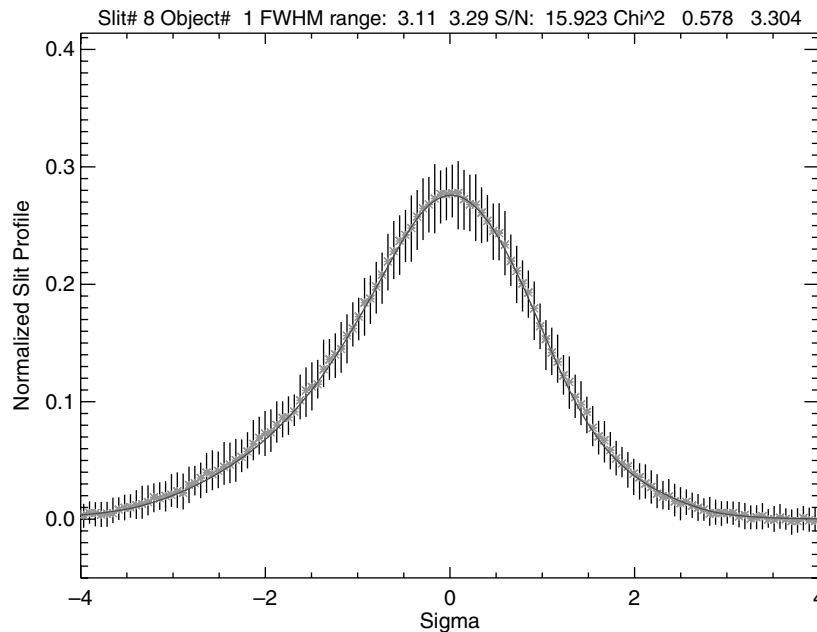
FIG. 8.—Illustrative slit profile produced during extraction. The normalized median counts are plotted as crosses . The error bars represent the 20th and 80th percentiles. The profile is shown as a function of sigma standard deviations where sigma is defined in terms of the mean full width at half-maximum ( \sigma = \text{FWHM}/2.35 ). Note that the FWHM can vary along the trace. See the electronic edition of the PASP for a color version of this figure.
