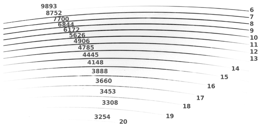
FIG. 1.—Example of MAGE spectrum of a flux standard. The central wavelengths and order numbers are listed near each order. The position of the wavelength labels do not correspond to their actual location on the chip. Note that the sensitivity of MAGE falls off sharply in orders 6 and 20. See the electronic edition of the PASP for a color version of this figure.
