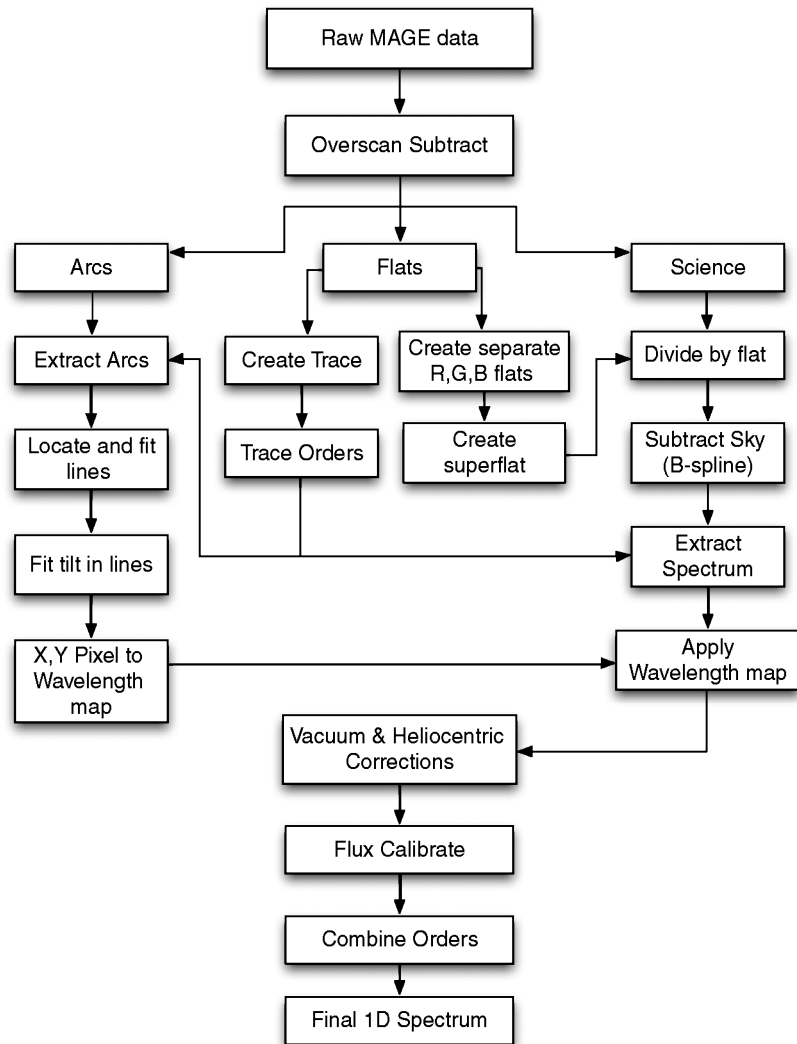
FIG. 3.—Illustrative flowchart of the MASE reduction pipeline. Each major step in the pipeline discussed in the text is shown.
