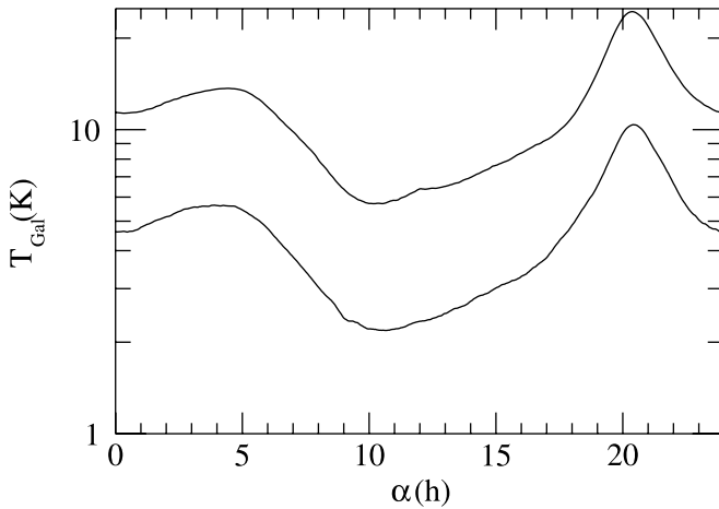
FIG. 2.—Brightness temperature of the Galaxy at 600 ( upper line ) and 820 MHz ( lower line ) after the separation of the celestial signal into primordial (CMB), extragalactic, and Galactic contributions. The correction for polarization based on Brouw & Spoelstra (1976) and Spoelstra (1984) is also taken into account. Some of the data plotted here are reported in Table 2 with the corresponding uncertainties.
