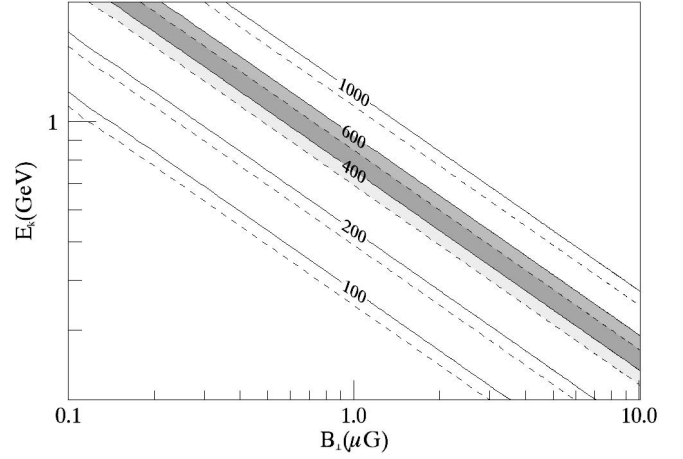
FIG. 8.— Contour levels of \nu_{\text{ex}}(\text{MHz}) in the (E_k, B_i) -plane. The two families of lines are referred to a_2 = 3.0 (dashed lines) and a_2 = 2.6 (solid lines) with a_1 = 1.7 (see § 4.3 for explanation). The regions with 400 \leq \nu_{\text{ex}}(\text{MHz}) \leq 600 are shown as distinct (and partially superposed) gray bands for the two cases.
