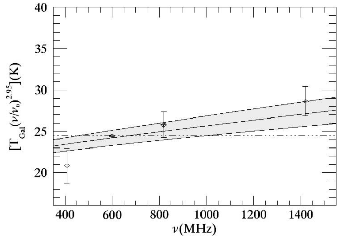
FIG. 9.— Temperature of the Galaxy toward the Cygnus region ( \alpha = 20^{\text{h}}24^{\text{m}}, \delta = +42^\circ ). The plot represents T_{\text{Gal}}(\text{K})(\nu/\nu_0)^{2.95} vs. \nu (MHz), with \nu_0 = 600.5 MHz. Diamonds : Experimental points at 408, 600.5, 817.85, 820, and 1420 MHz. The dot-dashed line is the temperature at 600 MHz scaled at the different frequencies with a synchrotron spectral index \beta_{\text{syn}} = 2.95 . The light gray band represents the result of the two-component (thermal+nonthermal) fit. The error bar at 600.5 MHz is smaller than the plotting symbol. See text for more details.
