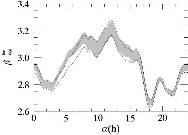
FIG. 5.—Local spectral index \beta_{\text{Gal}}^{\text{loc}} between 600 and 820 MHz (TRIS data) at \delta = +42^\circ . Gray band: Data not corrected for polarization effects. Region enclosed by solid lines: Data corrected for polarization. The width of the two bands represents the \pm\sigma uncertainty. The two bands, which have a similar width, are almost everywhere superposed, except in the region 04^{\text{h}} \lesssim \alpha \lesssim 08^{\text{h}} .
