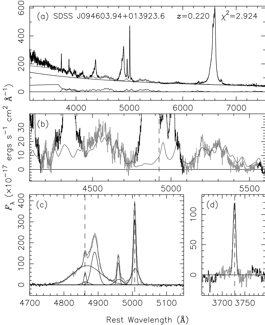
FIG. 14.—Spectrum of SDSS J094603.94+013923.6, an example of a OQ 208–like source. (a) Continuum decomposition. (b) Fe model and the observed spectrum after subtracting the power law and Balmer continuum. The spectra and the marks plotted in (a) and (b) are as the same as those in the top and bottom panels of Fig. 1. (c) Fitting of H \beta and [O III] emission lines. The multiple Gaussian components are in blue, and the sum of them is in red. The two blue dashed lines mark the rest-frame wavelength of H \beta and [O III] \lambda 5007 . (d) Fitting of [O II] emission line. The blue dashed line marks the rest-frame wavelength of [O II] \lambda 3727 . Note that the redshifts and widths of [O II], [O III], and H \beta_{NC} are almost the same. Note also that we added an additional redshifted Gaussian line to fit H \beta . The width and velocity shift of this redshifted H \beta component are consistent with those of Fe II emission. See text and Table 3 for more details. [See the electronic edition of the Journal for a color version of this figure.]
