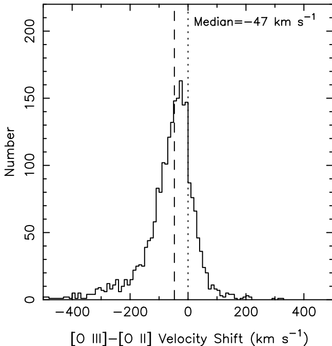
FIG. 5.—Distribution of [\text{O III}] velocity shifts with respect to [\text{O II}] . Positive velocity indicates a redshift. The dotted line marks the position of zero velocity shift, while the dashed line marks the median of the distribution.
