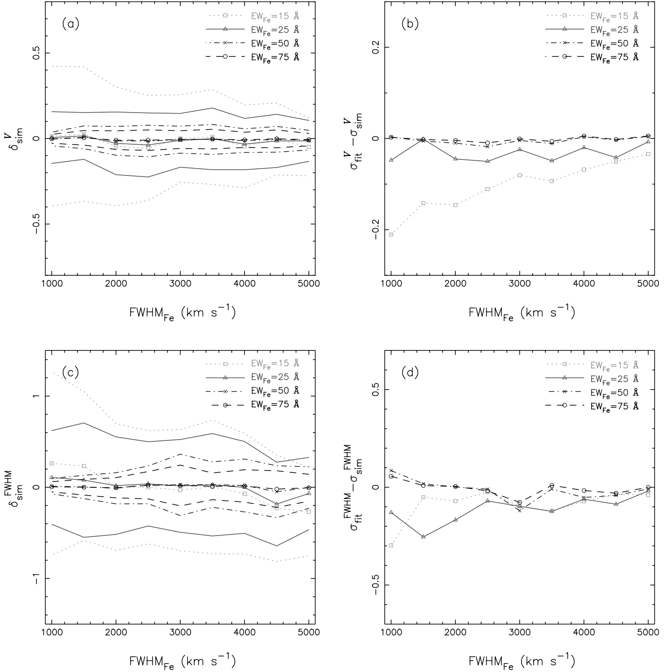
FIG. 4.—(a) Input-output simulations of v_{\text{Fe}} measurements. We define \delta_{\text{sim}}^V = (V_{\text{in}} - V_{\text{out}})/\text{FWHM}_{\text{in}} . For each \text{EW}_{\text{Fe}} , the middle line represents the mean \delta_{\text{sim}}^V , and the other two lines above and below are one standard deviation above and below the mean. The S/N in the simulation is 10, which is the lower limit of our sample, so the uncertainties shown here should be considered upper limits. (b) Test of the error bars given by the code; \sigma_{\text{fit}}^V is the average value of the errors given by the code in 100 trials, divided by \text{FWHM}_{\text{in}} , and \sigma_{\text{sim}}^V is the standard deviation of \delta_{\text{sim}}^V . (c) Input-output simulations of \text{FWHM}_{\text{Fe}} measurements. We define \delta_{\text{sim}}^{\text{FWHM}} = (\text{FWHM}_{\text{out}} - \text{FWHM}_{\text{in}})/\text{FWHM}_{\text{in}} . (d) Test of the error bars by the code. \sigma_{\text{fit}}^{\text{FWHM}} is the average value of the relative errors of \text{FWHM}_{\text{Fe}} given by the code in 100 trials, and \sigma_{\text{sim}}^{\text{FWHM}} is the standard deviation of \delta_{\text{sim}}^{\text{FWHM}} . See text for details of the simulation. [See the electronic edition of the Journal for a color version of this figure.]
