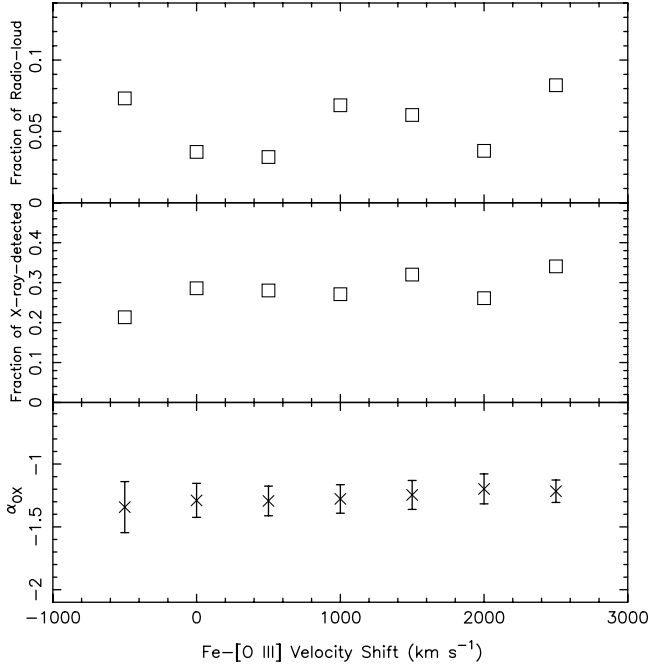
FIG. 11.— Top : Fraction of radio-loud quasars in bins of different v_{\text{Fe}} . Middle : Fraction of X-ray-detected quasars. Bottom : \alpha_{\text{ox}} in bins of different v_{\text{Fe}} .
