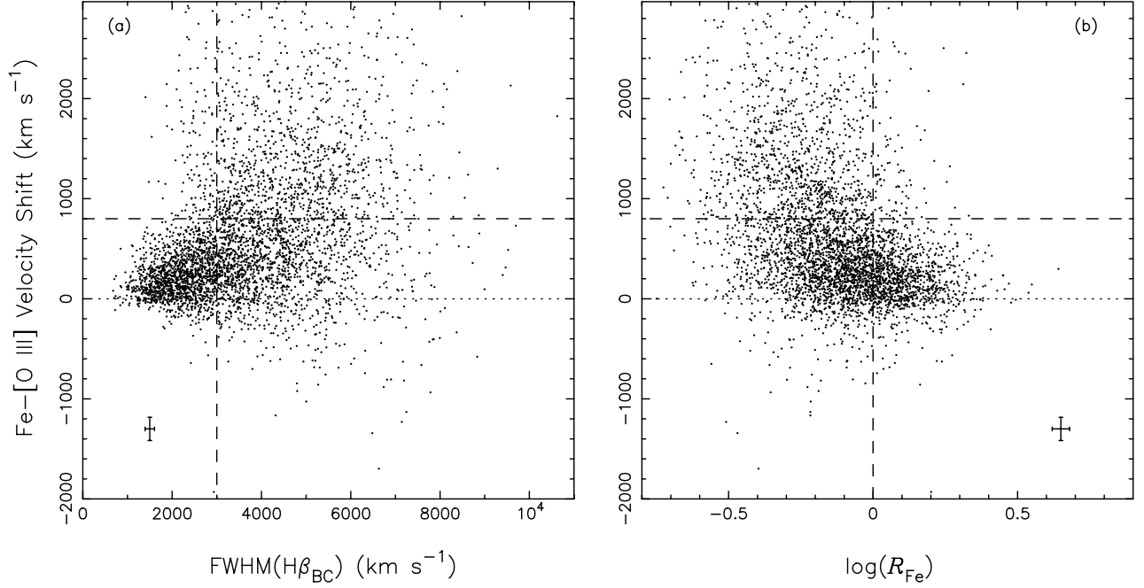
FIG. 9.—Correlation diagram for v_{\text{Fe}} vs. \text{FWHM}(\text{H}\beta_{\text{BC}}) (left) and for v_{\text{Fe}} vs. R_{\text{Fe}} (right). The crosses in the figure present the median values of the errors in both coordinates. See text for description of the vertical and horizontal lines.
