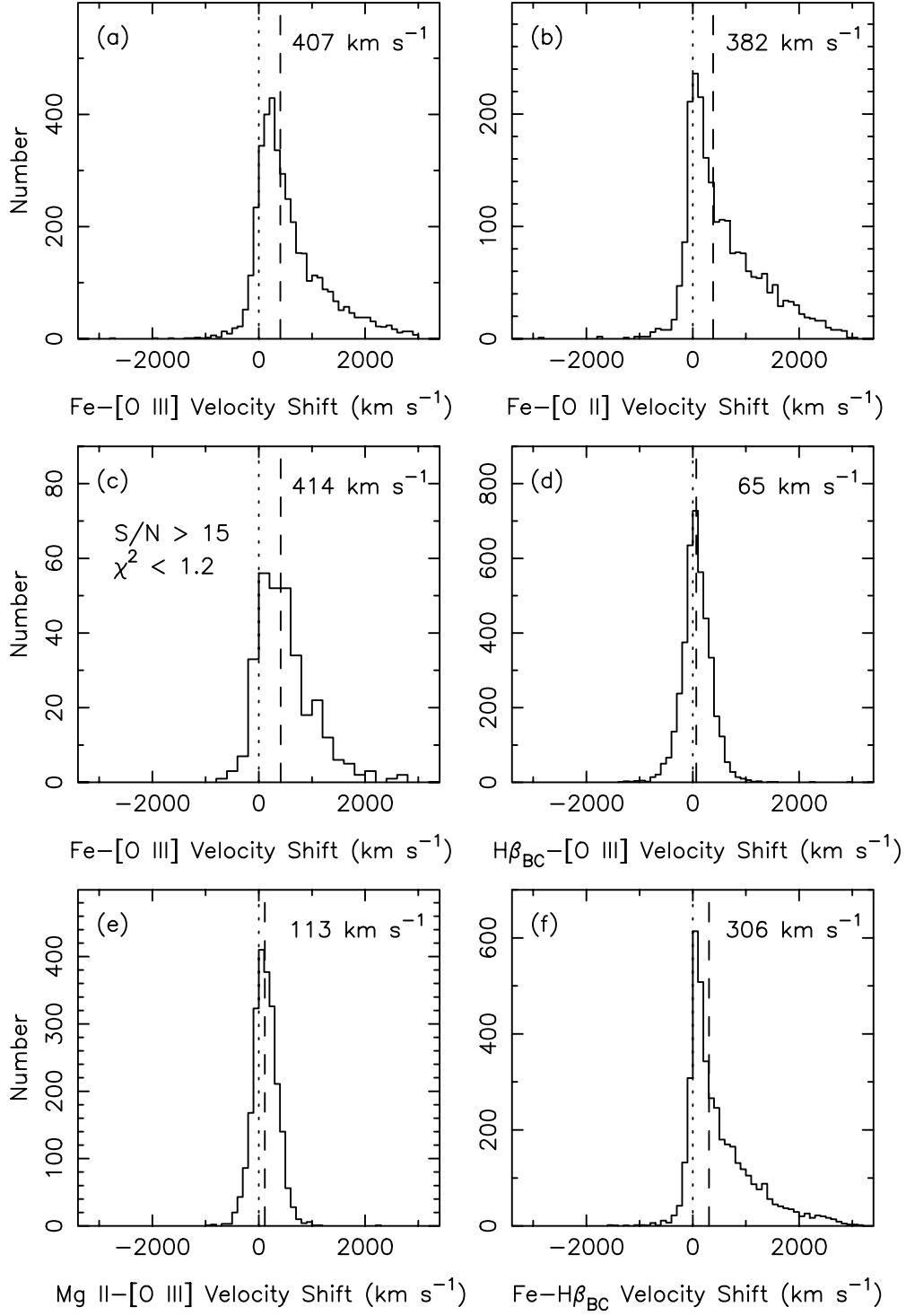
FIG. 7.—(a) Distribution of Fe II velocity shifts with respect to [O III]. (b) Fe II velocity shifts with respect to [O II]. (c) The distributions of v_{\text{Fe}} in the subsample that has the stricter criteria S/N > 15 and \chi^2 < 1.2 . (d) H\beta_{\text{BC}} velocity shifts with respect to [O III]. (e) Mg II velocity shifts with respect to [O III]. (f) Distribution of Fe II velocity shifts with respect to H\beta_{\text{BC}} . Positive velocity indicates a redshift. The number in each panel is the median value of the respective distribution, which is also marked by the dashed line. The dotted line marks the position of zero velocity shift.
