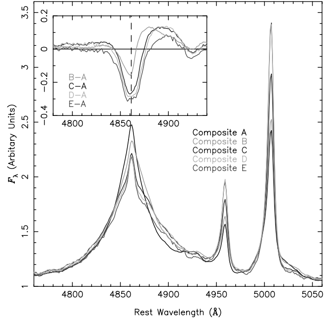
FIG. 13.—H \beta and [O III] region of the composite spectra. The inserted plot shows the difference spectra. The vertical dashed line is drawn at 4861 Å. Note the excess on the red wing of H \beta . [See the electronic edition of the Journal for a color version of this figure.]
