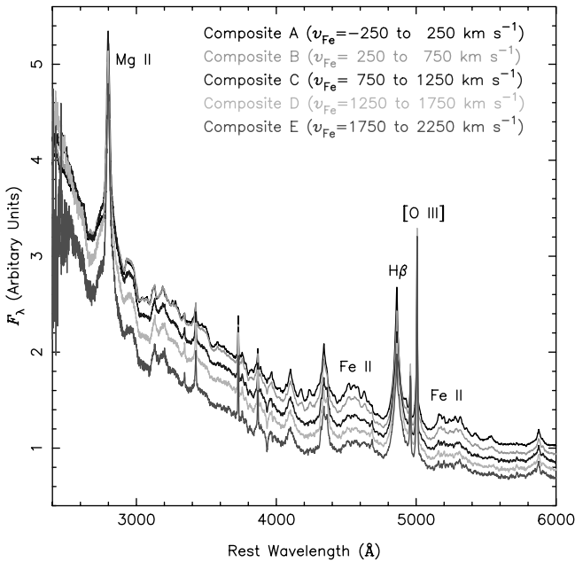
FIG. 12.—Composite spectra of quasars in bins of different v_{\text{Fe}} . See text for details on generating the composite spectra. We shifted the spectra vertically for clarity. Major emission lines are indicated; see Vanden Berk et al. (2001) for a complete identification of the emission lines. [See the electronic edition of the Journal for a color version of this figure.]
