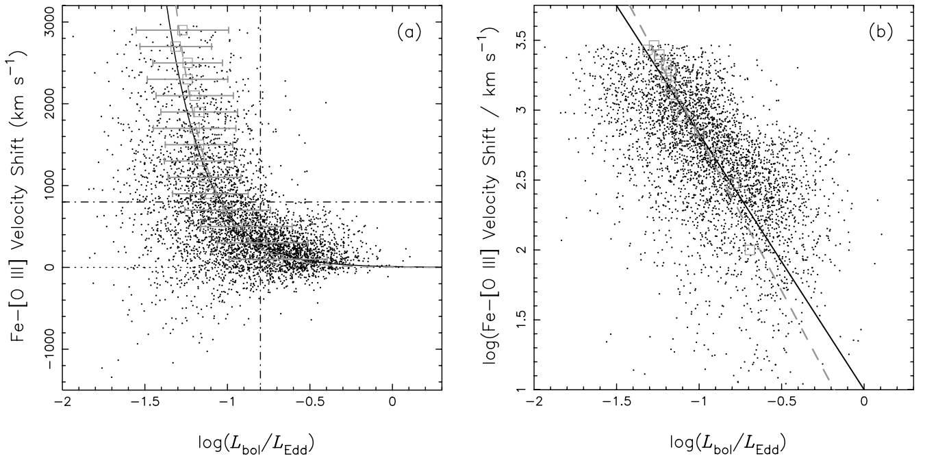
FIG. 10.—Correlation of Fe II velocity shift vs. Eddington ratio, with the Fe II velocity shift plotted (a) linearly and (b) logarithmically. See text explanation of the dot-dashed lines. The solid lines is the fit to data in eq. (12). The green squares represent the mean \log(L_{\text{bol}}/L_{\text{Edd}}) in bins of \Delta v_{\text{Fe}} = 200 \text{ km s}^{-1} , and the error bars represent the standard deviations. The green dashed line shows the fit to the binned data. [See the electronic edition of the Journal for a color version of this figure.]
