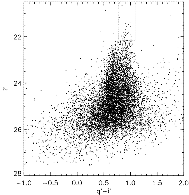
FIG. 1.—CMD for the globular clusters around NGC 3311. Note that the color index plotted here is the dereddened value (g' - i')_0 . The box indicates the location in color-magnitude space of the UCD candidates. [See the electronic edition of the Journal for a color version of this figure.]
