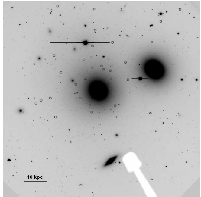
FIG. 2.—The i' -band GMOS field of NGC 3311 (center) and NGC 3309 (upper right). Locations of UCD candidates are marked by circles. The field size shown is 5.5' across. The shadow of the guide probe is seen at the bottom. North is up, and east is to the left. [See the electronic edition of the Journal for a color version of this figure.]
