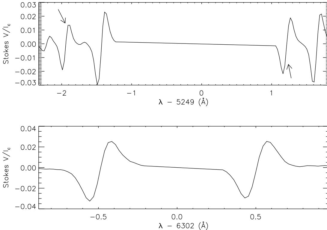
FIG. 9.—Average observed Stokes V profiles in a network patch (located approximately around coordinates [20, 7] in Fig. 1) continuum intensity. The 5250 line ratio (the relevant Fe I lines are marked with arrows) is 1.21.
