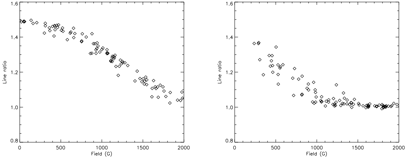
FIG. 3.—Line ratio calibration using synthetic Stokes profiles of Fe I 5250 Å emergent from the HSRA model atmosphere after adding random temperature perturbations and magnetic fields. Left : Macro-turbulence was kept fixed at 3 \text{ km s}^{-1} . Right : Random macro-turbulence varies between 0 and 1 \text{ km s}^{-1} .
