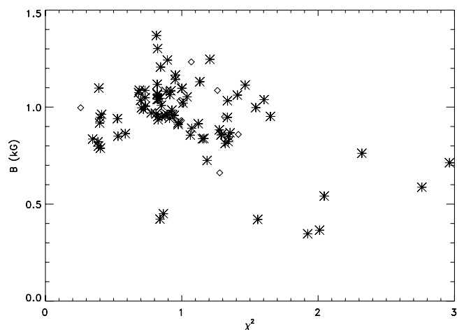
FIG. 18.—Inversions of the 5250 Å region. Average magnetic field in the lower photosphere of the MISMA component that harbors more flux, as a function of the quality of the fit \chi^2 . Asterisks: Solutions where the temperature decreases outwards in the upper photosphere. Diamonds: Solutions where the temperature increases outwards in the upper photosphere.
