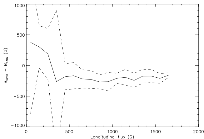
FIG. 7.—Differences in intrinsic field strengths measured at 6302 and 5250 Å as a function of the average longitudinal magnetic flux density. The solid line represents the median value over 100 G bins. The dashed lines represent the standard deviation of the points in each bin.
