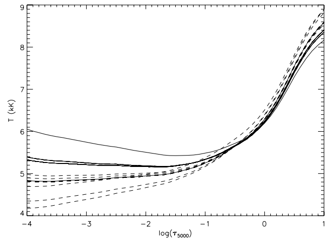
FIG. 16.—Temperature stratification of the models obtained from the 5250 Å inversions with LILIA. Solid line : Models that include kG fields. Dashed line : Models with sub-kG field.
