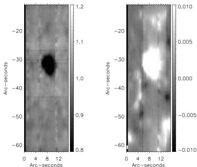
FIG. 2.—Continuum intensity map ( left ) and reconstructed magnetogram ( right ) of the pore scan near 5250 Å. The magnetogram shows the integrated Stokes V signal over a narrow bandwidth on the red lobe of the Fe I 5250.2 Å line. In both panels, values are referred to the average quiet-Sun intensity. The angular scale on the vertical axis measures the distance from the upper hairline.
