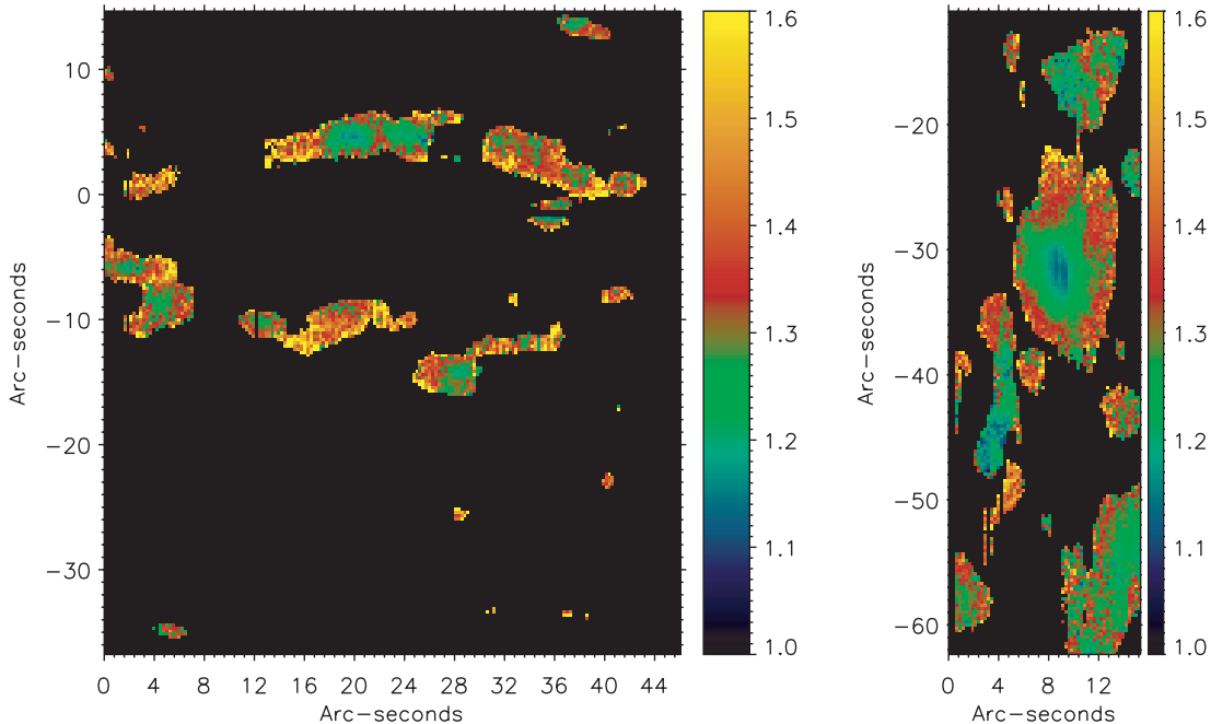
FIG. 4.—Amplitude ratio of Stokes V in Fe I 5250.2 Å to Fe I 5247.0 Å. Left : Network patches observed in the quiet-Sun scan. Right : A small pore (centered on coordinates [10, -30], approximately) and surrounding plage. Ratios close to 1 are indicative of a strong field of nearly 2 kG. Ratios close to 1.6 correspond to the weak-field (up to \sim 500 \text{ G} ) regime. Black areas exhibit a circular polarization amplitude smaller than 1% and have not been inverted.
