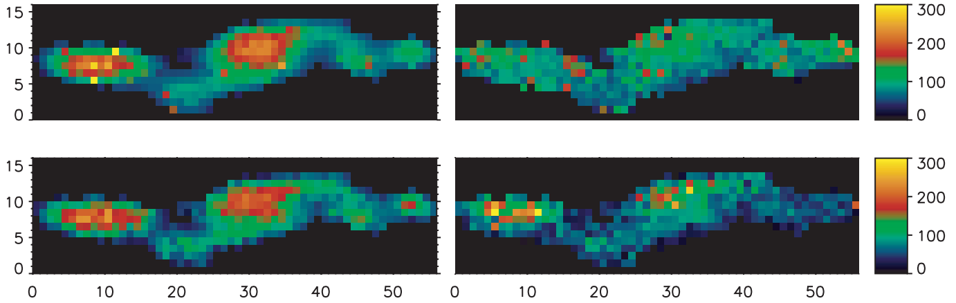
FIG. 8.—Longitudinal flux density from the inversions of a network patch at 6302 Å ( left ) and 5250 Å ( right ). Upper panels : Inversions with the Milne-Eddington code MELANIE. Lower panels : Inversions with the LTE code LILIA. Spatial scales are in pixels.
