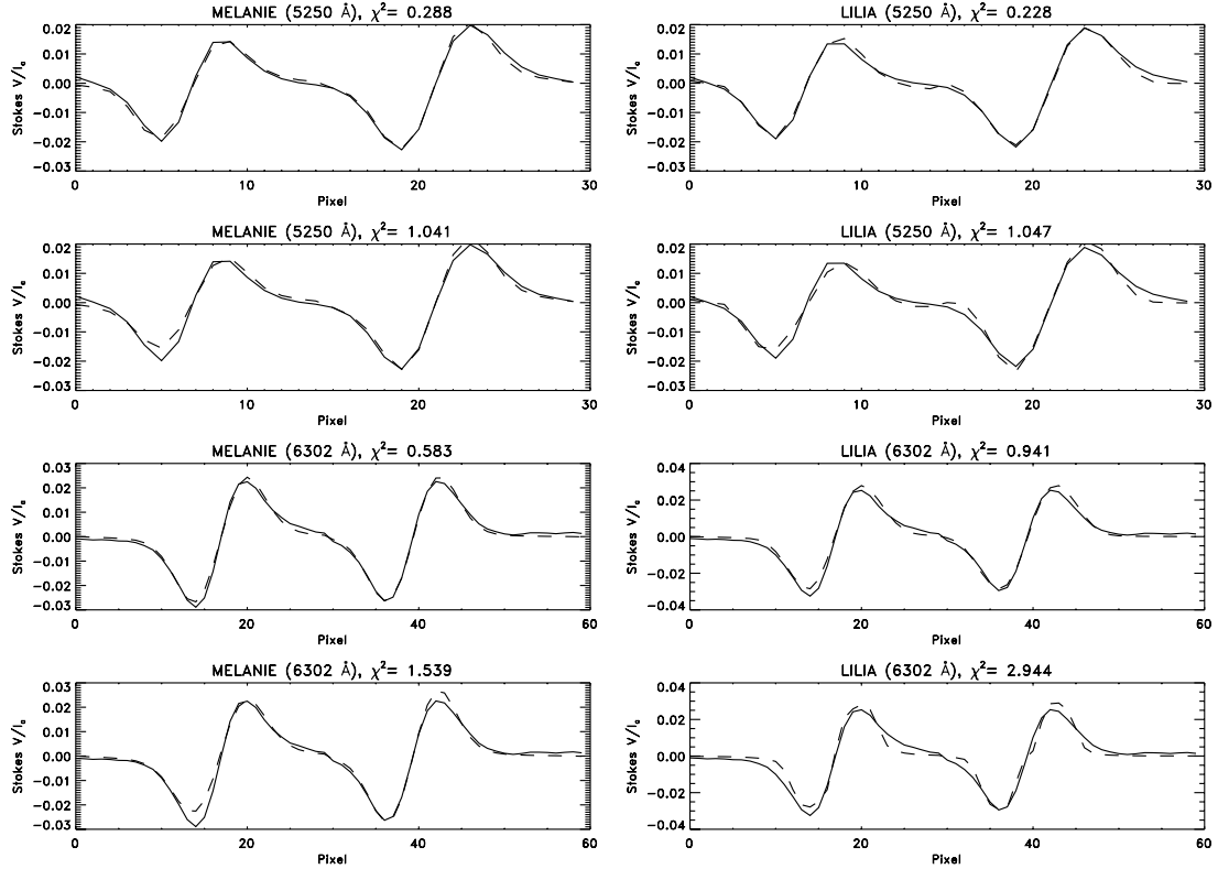
FIG. 14.—Fits obtained with MELANIE ( left ) and LILIA ( right ) to the average network profile observed at 5250 Å ( upper four panels ) and 6302 Å ( lower four panels ). For each case we show the best fit (smaller \chi^2 ) and a not so good one.
