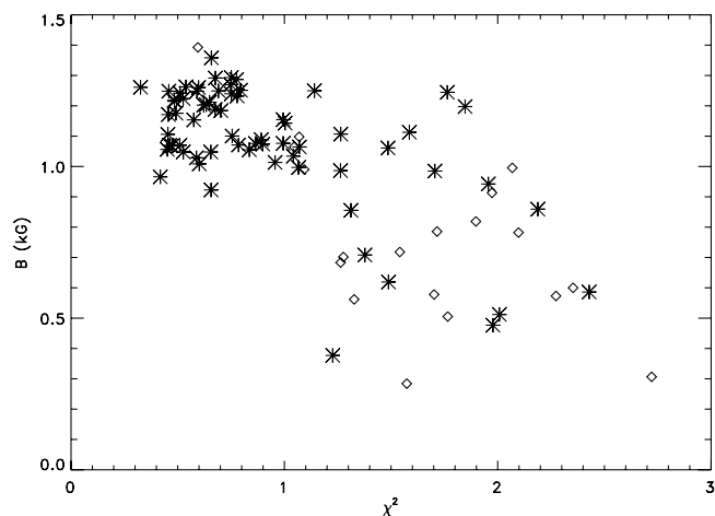
FIG. 17.—Inversions of the 6302 Å region. Average magnetic field in the lower photosphere of the MISMA component that harbors more flux, as a function of the quality of the fit \chi^2 . Asterisks: Solutions where the temperature decreases outwards in the upper photosphere. Diamonds: Solutions where the temperature increases outwards in the upper photosphere.
