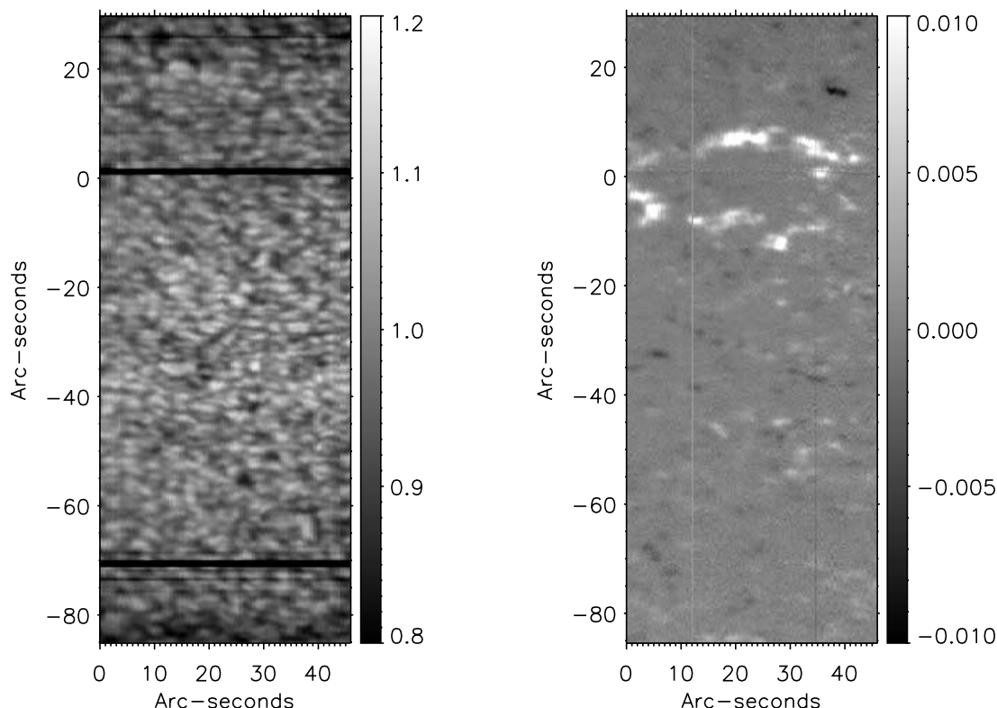
FIG. 1.—Continuum intensity map ( left ) and reconstructed magnetogram ( right ) of the quiet-Sun scan near 5250 Å. The magnetogram shows the integrated Stokes V signal over a narrow bandwidth on the red lobe of the Fe I 5250.2 Å line. In both panels, values are referred to the average quiet-Sun intensity. The angular scale on the vertical axis measures the distance from the upper hairline.
