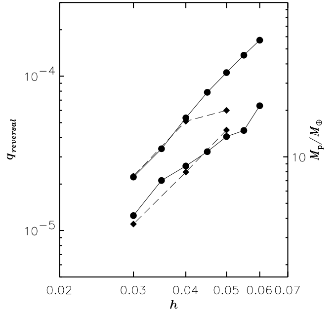
FIG. 17.—Domain of migration reversal, in the (h, q) -plane, in the unsaturated case ( solid curves ) and partially saturated case ( dashed curve ). For each line style ( solid or dashed ), the lower curve represents the minimal mass for migration reversal while the upper curve represents the maximal mass for migration reversal. At low h (hence low q ), the partially saturated and unsaturated results almost coincide, since the corotation torque is very weakly saturated (we work with a constant kinematic viscosity), while the reversal domain is more narrow at large h , owing to the increasing corotation torque saturation. The right axis labeling assumes a solar mass central object.
