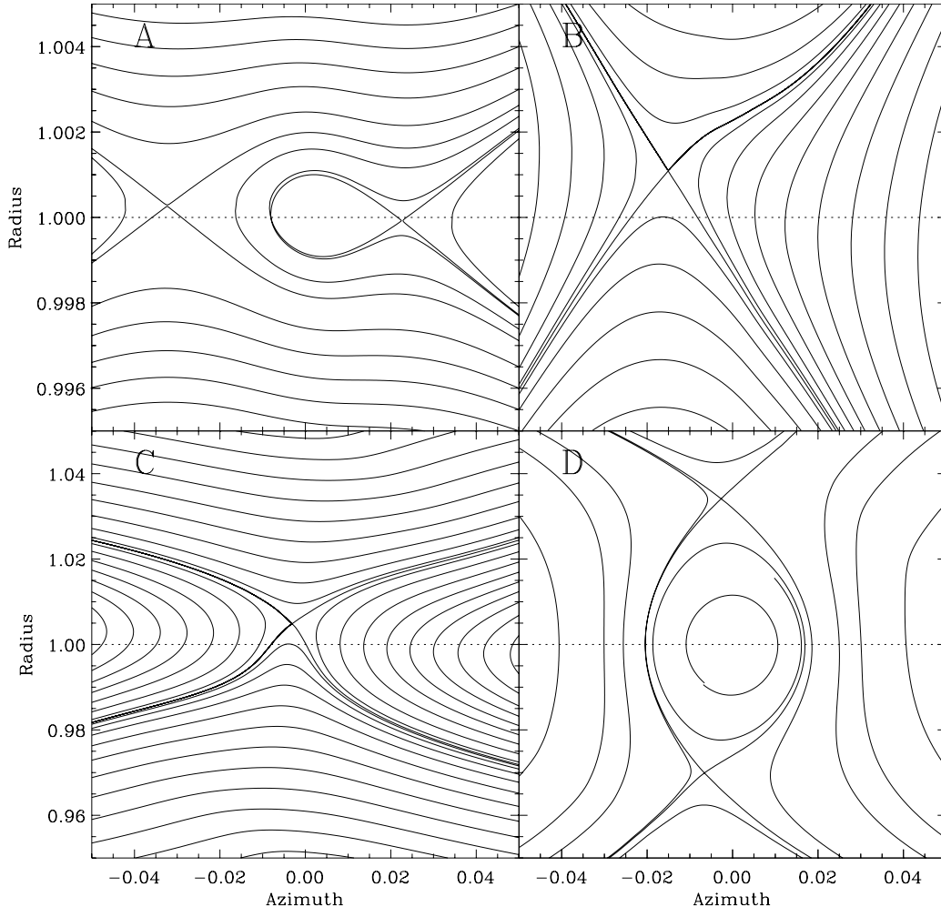
FIG. 11.—Streamline appearance for the four planet masses quoted in text, at t = 10 orbits. The radial range is the same for cases A and B and for cases C and D. It is 10 times larger for the latter than for the former. The aspect ratio is 1 : 1 for cases C and D.
