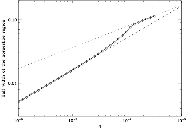
FIG. 9.—Horseshoe zone half-width as a function of the planet mass for the 35 planets of the reference calculations. The dashed line represents the horseshoe zone half-width expected from eq. (3). It scales with q^{1/2} . The dotted line shows the relationship x_s \propto q^{1/3} , which passes through the large-mass data points.
