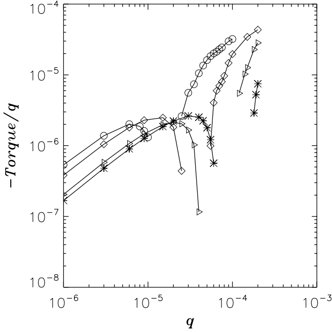
FIG. 7.—Negative of the specific torque acting on the planet as a function of the planet to primary mass ratio, for different values of h : 0.06 (asterisks), 0.05 (triangles), 0.04 (diamonds), and 0.03 (circles). Torques are measured at early times (between 7 and 10 orbits) so that corotation torques are unsaturated. Gaps in the curves identify the ranges of planetary masses for which the total torque is positive.
