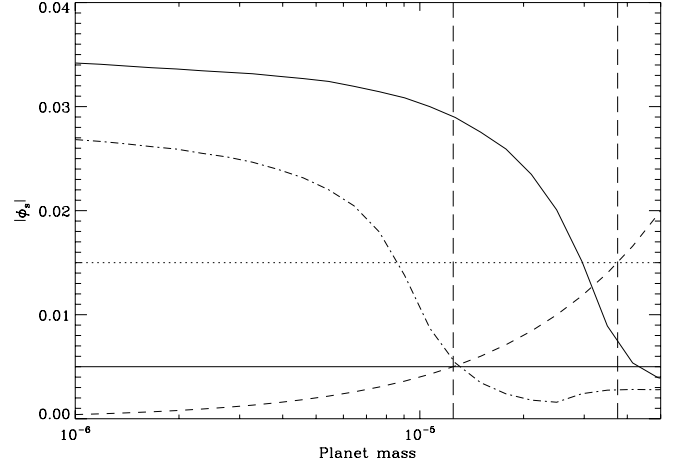
FIG. 15.—Negative of the azimuth of the left stagnation point as a function of the planet mass for the standard softening length case ( \epsilon = 0.3H ; solid line) and for a 3 times smaller softening length case ( \epsilon = 0.1H ; dash-dotted line). The dashed line shows the Bondi radius as a function of the planet mass. The horizontal dotted line shows the standard softening length ( \epsilon = 0.015 ), while the horizontal solid line shows the shorter softening length ( \epsilon = 0.005 ). The vertical lines show the mass for which the planet's Bondi radius is equal to the potential softening length in both cases. We see that the stagnation point enters the Bondi sphere when r_B \approx \epsilon .
