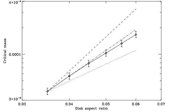
FIG. 6.—Critical mass q_c for maximal offset as a function of the disk thickness, for the two-dimensional runs. The dotted, dashed, and dot-dashed lines show, respectively, the relationships q_c \propto h^2 , q_c \propto h^4 , and q_c \propto h^3 , which pass through the leftmost data point. The error bars indicate the sampling of data points around the critical mass.
