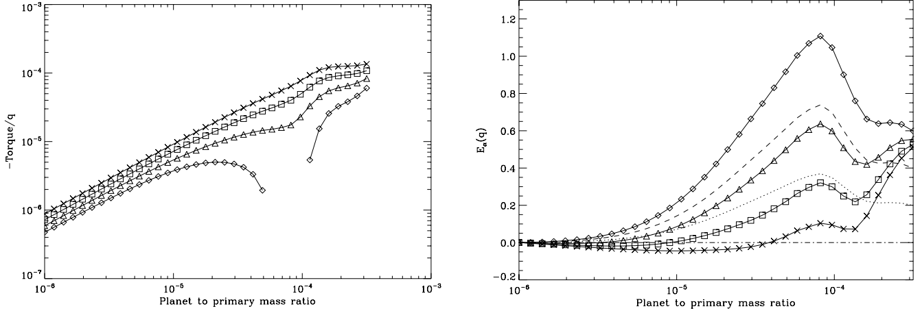
FIG. 2.—Two-dimensional results. Left : Negative of specific torque acting on the planet, as a function of its mass, for four values of the surface density slope: \alpha = 0 (diamonds), \alpha = 1/2 (reference calculation; triangles), \alpha = 1 (squares), and \alpha = 3/2 (crosses). The hole in the data for the flat surface density profile corresponds to a torque reversal. Right : Departure from linearity for the same surface density slopes (same symbols). The meaning of the additional lines is explained in the text.
