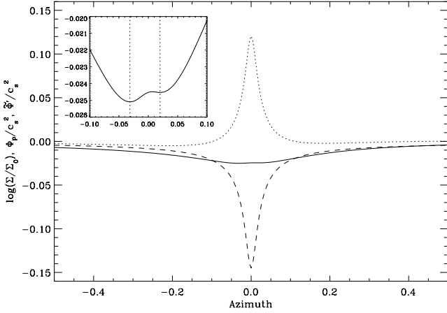
FIG. 14.—Graph shows \log(\Sigma/\Sigma_0) (dotted line), \Phi_p/c_s^2 (dashed line), and their sum ( \tilde{\Phi}/c_s^2 ; solid line) as a function of azimuth at r = 1 for the case A (planet mass q = 5.44 \times 10^{-6} ) with the very high radial resolution ( N_{\text{rad}} = 3860 ). We note in passing that the close up shows two relative extrema (vertical dotted lines), which correspond to the position of the stagnation points shown in Fig. 11. The Bondi radius to softening length ratio for this planet is r_B/\epsilon = 0.145 \ll 1 , which implies that the flow is linear even at the planet location. We see that indeed the maximum value of |\Sigma - \Sigma_0|/\Sigma_0 \approx \log(\Sigma/\Sigma_0) is of the order of the above ratio.
