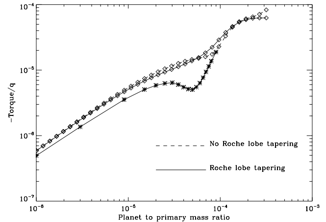
FIG. 1.—Negative of specific torque acting on the planet, as a function of its mass, in the reference disk for the two-dimensional case. The solid line with diamonds shows the torque computed with Roche lobe tapering, while the dashed line shows the torque computed without special treatment of the Roche lobe zones. The solid line with stars shows the results of the three-dimensional calculations, scaled by \Sigma_0^{2D}/\Sigma_0^{3D} = 60/29 . We note that the offset depth is larger in the three-dimensional case.
