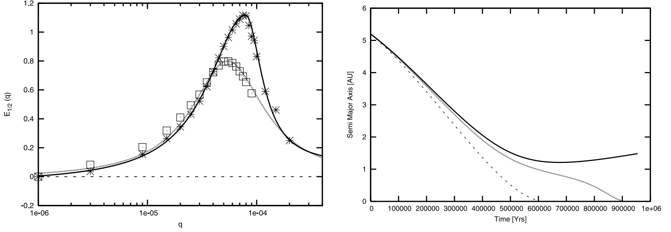
FIG. 16.— Left: The departure from linearity for three-dimensional models with \alpha = 1/2 for the unsaturated ( stars ) and saturated ( squares ) case. The solid and dotted lines are the corresponding analytical fit formulae used for evolving the planet. The dashed line ( E_{1/2} = 0 ) refers to the linear case. Right: The evolution of an embedded planet in the disk using these analytical formulae (unsaturated, solid line ; saturated, dotted line ; linear, dashed line ).
