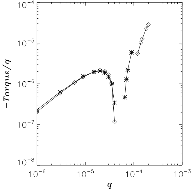
FIG. 5.—Negative of the specific torque acting on the planet, as a function of its mass, for models with \alpha = 0 . Asterisks indicate torques, from long-run simulations, for which corotation torques are saturated. Diamonds represent torques at early times (between 7 and 10 orbits); hence corotation torques are unsaturated.
