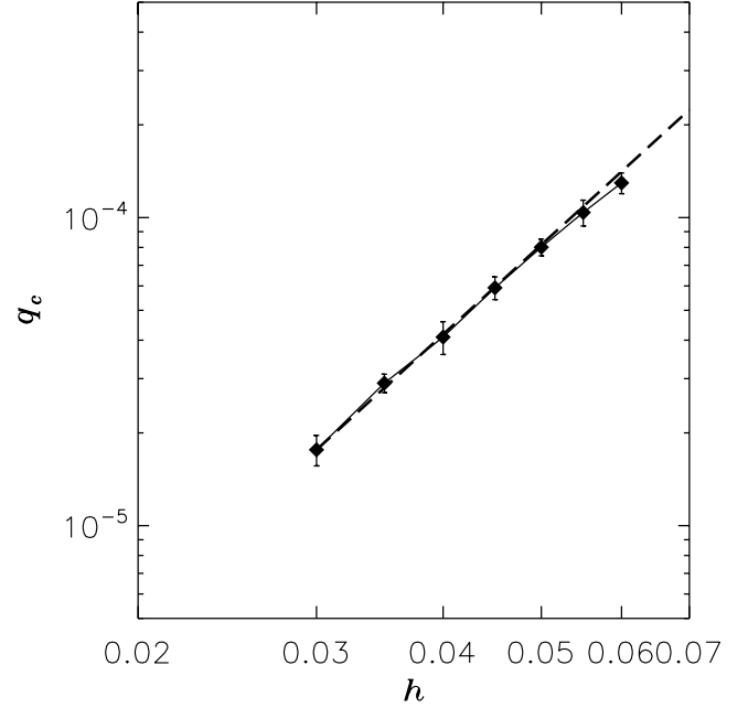
FIG. 8.—Critical mass vs. the relative disk thickness obtained from three-dimensional calculations. At q = q_c , the offset is the largest. The error bars indicate the sampling of the data points around the critical mass. The dashed line identifies the relationship q_c \propto h^3 passing through the data point with minimum h .
