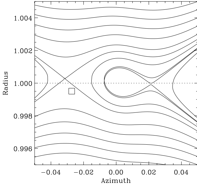
FIG. 12.—Streamline appearance for the planet mass A quoted in text, at t = 10 orbit, with a radial resolution 10 times higher than in Fig. 11. The streamlines appearance and the position of the stagnation points is almost indistinguishable from the lower resolution case. The square shows a zone from the high-resolution mesh.
