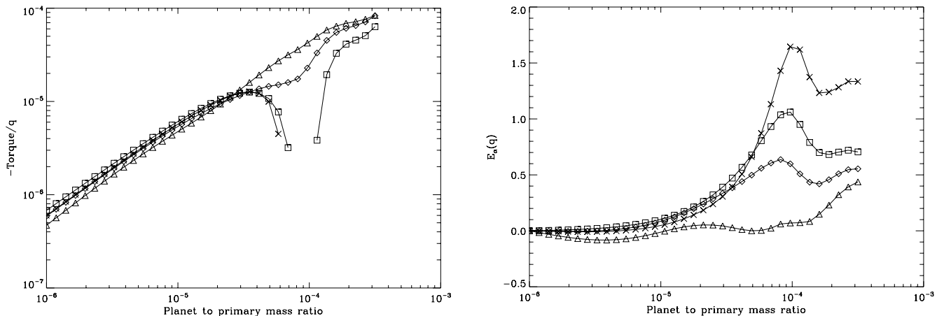
FIG. 4.— Left : Specific torque acting on the planet as a function of the planet mass for different disk viscosities: \nu = 5 \times 10^{-6} (triangles), \nu = 10^{-5} (reference calculations; diamonds), \nu = 2 \times 10^{-5} (squares). The curve with crosses shows the torque of the reference calculations averaged between t = 6 and t = 7 orbits, i.e., the early value of the torque, before it possibly saturates. Right : The value of E_\alpha (given by eq. [2]) for these calculations (same symbols).
