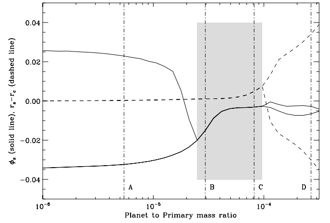
FIG. 13.—Azimuth \phi_s of the stagnation point(s) (solid line) and radial distance to corotation ( r_s - r_c ) of the fixed point(s) (dashed line) as a function of the planet mass. The gray shaded zone shows the mass interval over which there is a unique stagnation point. The four vertical dot-dashed lines show the masses for which the flow topology is sketched in Fig. 11.
