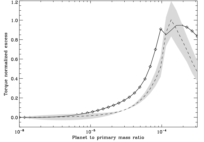
FIG. 10.—Horseshoe drag ( dashed line ) and total torque ( solid line ) normalized excesses as a function of planet mass. The shaded area shows the uncertainty on the horseshoe drag, arising from the uncertainty on the horseshoe zone width. If one calls x_s^- ( x_s^+ ) the distance of the inner (outer) separatrix to the corotation, then the upper (lower) limit of the shaded zone is given by using \max(x_s^-, x_s^+) [ \min(x_s^-, x_s^+) ] in eq. (4), while the dashed line uses (1/2)(x_s^- + x_s^+) .
