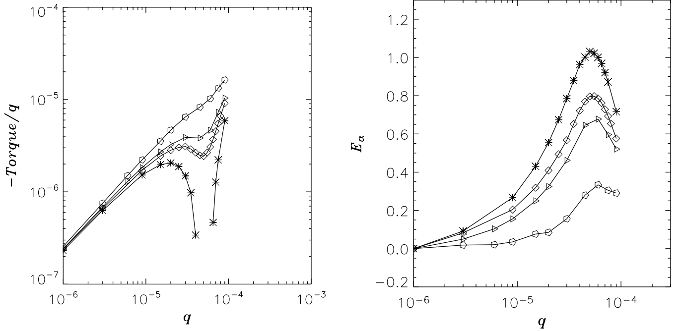
FIG. 3.—Three-dimensional results. Left : Negative of the specific torque exerted on the planet, as a function of its mass, for different values of the surface density slope: \alpha = 0 (asterisks), \alpha = 1/2 (diamonds), \alpha = 3/4 (triangles), and \alpha = 3/2 (pentagons). The gap in the data for the \alpha = 0 case corresponds to situations where the total torque is positive. Right : Departure from linearity (eq. [2]) for the same values of \alpha (same symbols).
