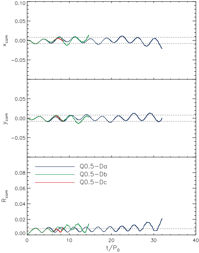
FIG. 11.—Drift of the center of mass during the Q0.5-D simulations: Q0.5-Da (blue), Q0.5-Db (green), and Q0.5-Dc (red). Top to bottom: The x - and y -components of the position of the center of mass in the corotating frame, and the cylindrical radial distance to the center of mass R_{\text{com}} , as functions of t/P_0 . The dotted lines at \pm\Delta R show the extent of the innermost radial grid zone. The center of mass stays very nearly within this one radial grid zone throughout these evolutions.
