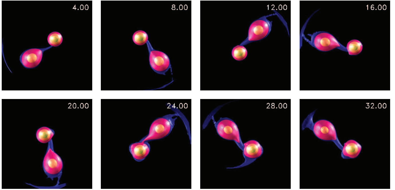
FIG. 7.—Same as Fig. 3, but for our Q0.5-Da evolution; images are separated in time by 4 initial orbital periods. Even after 32 orbits, the system continues to undergo mass transfer and there is no indication that the system will merge. [This figure is available as an mpeg file in the electronic edition of the Journal.]
