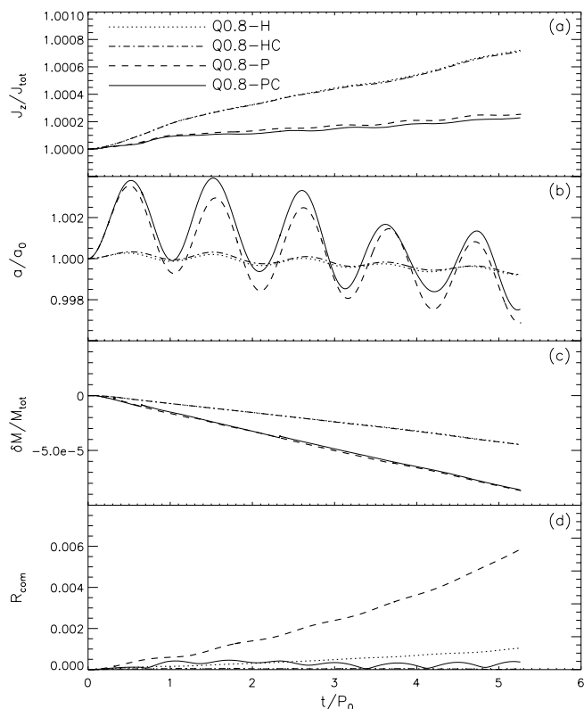
FIG. 2.—Results from the evolution of model Q0.8 using four slightly different versions of the hydrocode (evolution H: dotted line; HC: dot-dashed line; P: dashed line; PC: solid line). (a) The z -component of the system's angular momentum J_z , normalized to its initial value J_{\text{tot}} , plotted as a function of time t , normalized to the system's initial orbital period P_0 = 2\pi/\Omega_0 . (b) Binary separation a , normalized to its initial value a_0 , plotted as a function of t/P_0 . (c) Difference between the total mass of the binary system and its initial value, \delta M \equiv M(t) - M_{\text{tot}} , normalized to the initial mass, plotted as a function of t/P_0 . (d) Distance in code units R_{\text{com}} from the axis of the grid to the instantaneous center of mass as a function of t/P_0 . Note that the boundary of the innermost radial cell in these units is at R_{\text{com}} = 0.008 .
