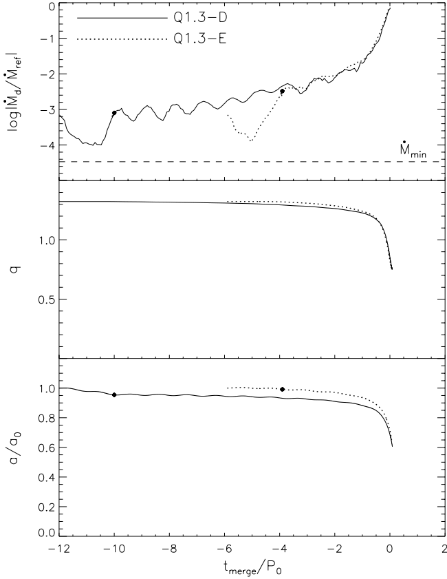
FIG. 5.—Evolution of the mass transfer rate ( top ), the mass ratio q , and the separation a for the same initial binary driven to contact by removing angular momentum (Q1.3-D, solid lines ) and by expansion of the donor (Q1.3-E, dotted lines ). The times shown are times to “merger” measured in initial binary periods. The dashed line in the top panel indicates the minimum level of mass transfer \dot{M}_{\text{min}} that is resolvable in our simulations (see text). The separation a is normalized to its initial value a_0 . The mass transfer rate is normalized to the reference value \dot{M}_{\text{ref}} \equiv \dot{M}_d(0)/P_0 (initial donor mass divided by initial orbital period). For most of the evolution q > 1 , so a decreases as a result of mass transfer even in the absence of driving. The filled circles mark the points at which driving was stopped.
