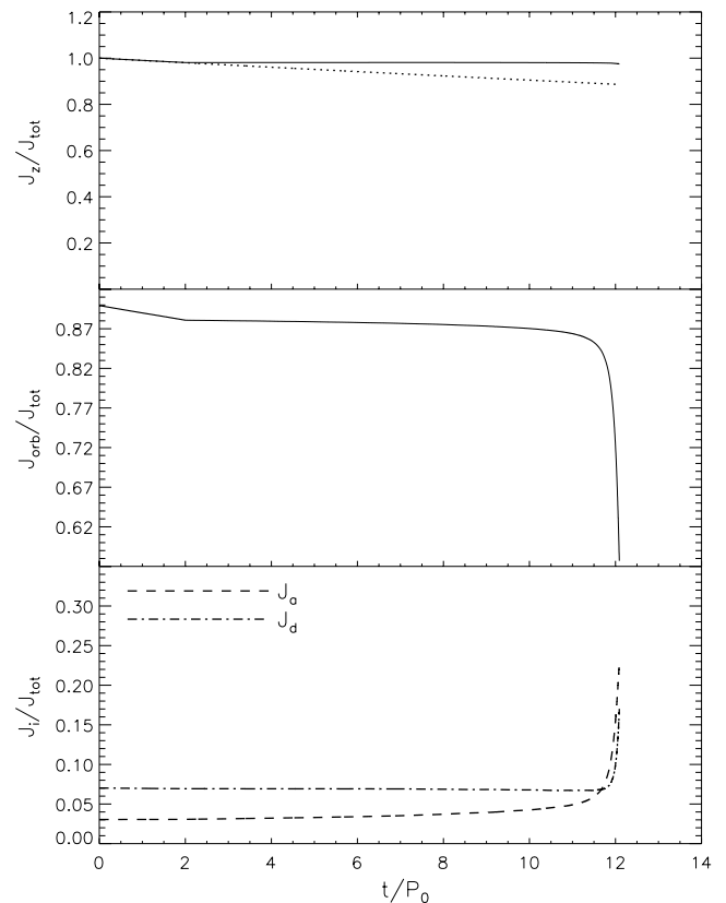
FIG. 4.—Top: The z -component of the total angular momentum with respect to an inertial frame centered at the center of mass, J_z , normalized to its initial value for Q1.3-D (solid line). The initial loss rate of angular momentum at 1% per orbit is denoted by the dotted line. The driving for Q1.3-D is stopped after 2 orbits, and this can be seen when the solid line becomes horizontal. Middle and bottom: Evolution of the orbital angular momentum and the spin angular momenta of the components all normalized to the total initial angular momentum for the Q1.3-D run.
