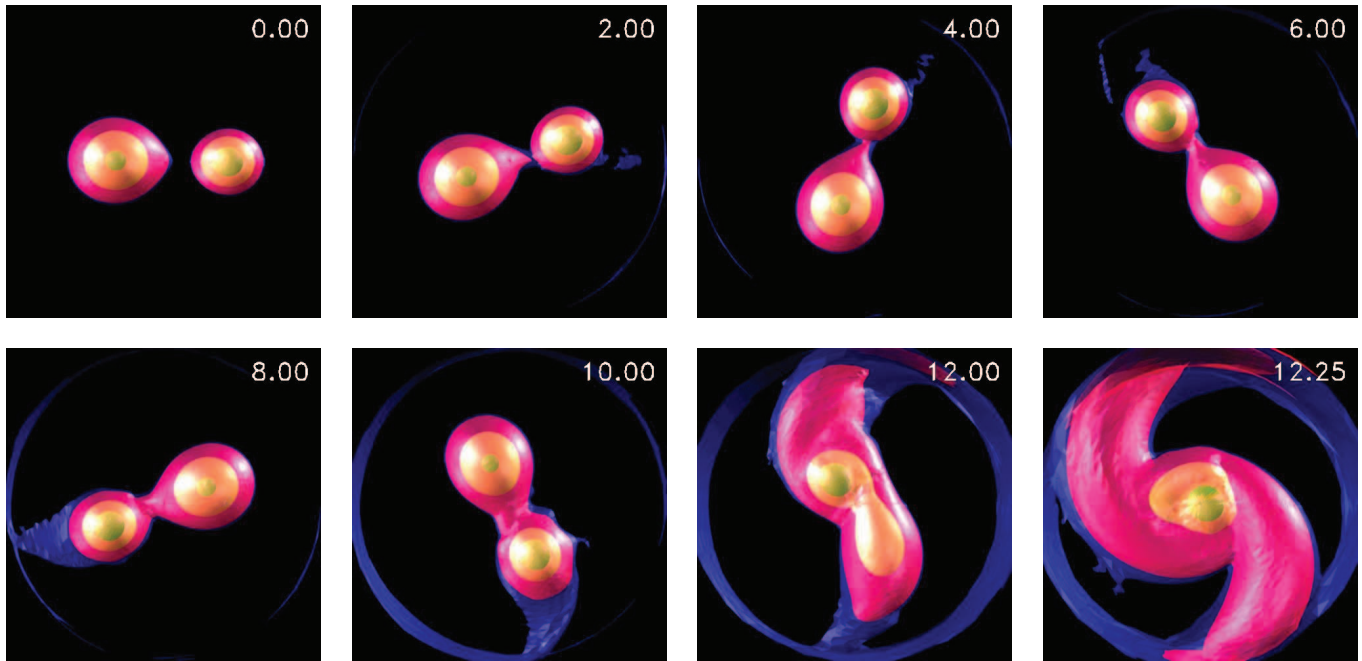
FIG. 3.—Three-dimensional rendering of the mass density at selected time slices during the Q1.3-D evolution that demonstrate direct impact accretion. Times are shown on the top right of each frame in units of the initial orbital period. Each image is a snapshot as viewed by an observer looking down on the equatorial plane while rotating with the angular velocity \Omega_0 . The four colored transparent shells are isodensity surfaces shown at levels \rho/\rho_a^{\max} = 0.5 (green), 0.1 (yellow), 10^{-3} (red), and 10^{-5} (blue), where \rho_a^{\max} is the maximum density of the accretor—the star on the right in the initial frame ( t = 0 ) of the figure. [This figure is available as an mpeg file in the electronic edition of the Journal.]
