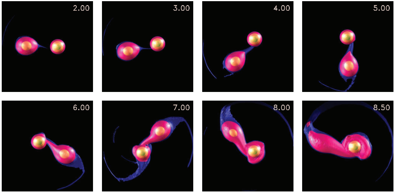
FIG. 10.—Same as Fig. 7, but for our Q0.5-Dc evolution; images are separated in time by 1 initial orbital period, except the last image. Since this binary is continuously driven, the separation and the orbital period decrease throughout, except perhaps at the very end.
