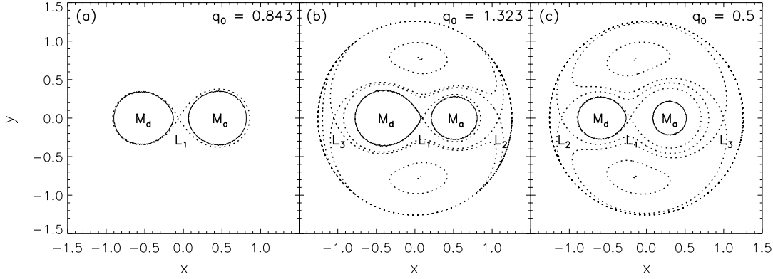
FIG. 1.—Slice through the equatorial plane shown for (a) model Q0.8, (b) model Q1.3, and (c) model Q0.5. In each panel, the solid isodensity contours denote the surfaces of the two stars; they are drawn at a level, \rho/\rho_d^{\max} = 10^{-5} . The “donor” star is located on the left in each panel. The dashed lines trace selected equipotential contours of the self-consistently calculated Roche potential for each model. The outermost circle drawn in panels (b) and (c) identifies the radial edge, R_{\text{grid}} , of the computational grid that was used to evolve these initial models hydrodynamically. The location of the inner ( L_1 ) Lagrange point is identified for each system; for models Q1.3 and Q0.5, two additional ( L_2 and L_3 ) Lagrange points are identified because they fall at positions R < R_{\text{grid}} .
