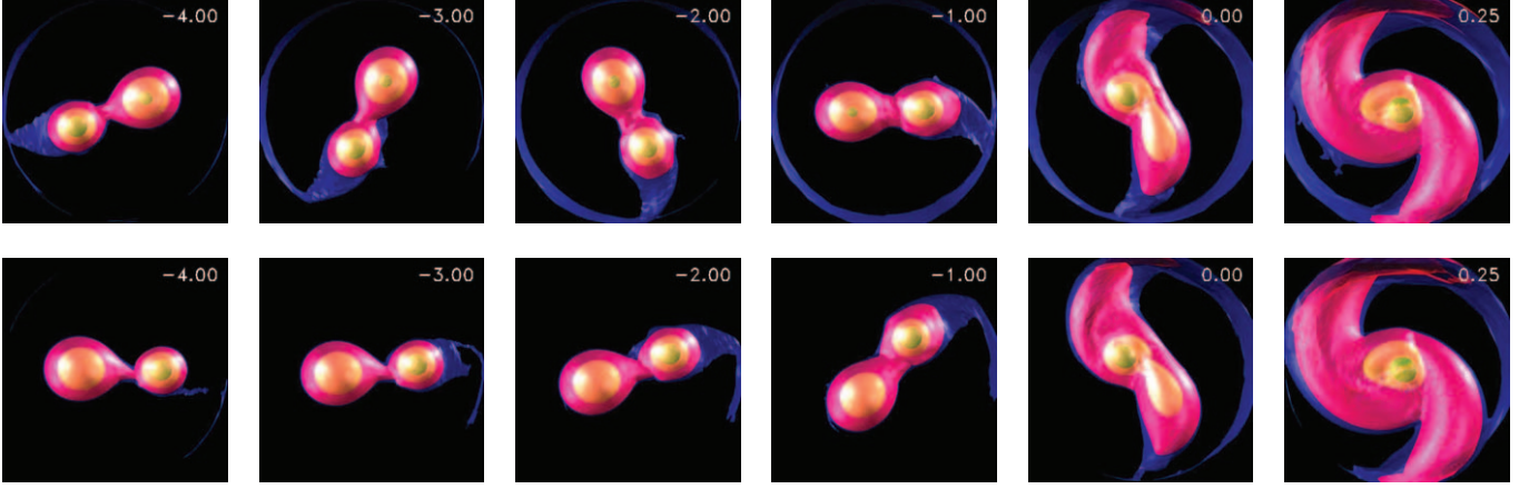
FIG. 6.—Two evolutions with q_0 = 1.3 , in which mass transfer is initiated by angular momentum losses (Q1.3-D; top row ) and by expansion of the donor (Q1.3-E; bottom row ), leading to an almost identical merger. The time shown in the movie is t_E . [This figure is available as an mpeg file in the electronic edition of the Journal.]
