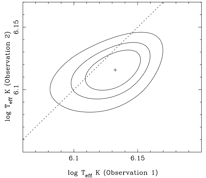
FIG. 4.—Comparison of the effective temperature (for an observer on the surface of the neutron star) between observations 1 and 2 when taking the distance to the source to be 8.5 kpc. The contours mark the 68.3%, 90%, and 99% confidence levels. The dashed line indicates where the temperature of observation 1 equals the temperature of observation 2. The contours were determined with the power law fixed to the best-fitting value. [See the electronic edition of the Journal for a color version of this figure.]
