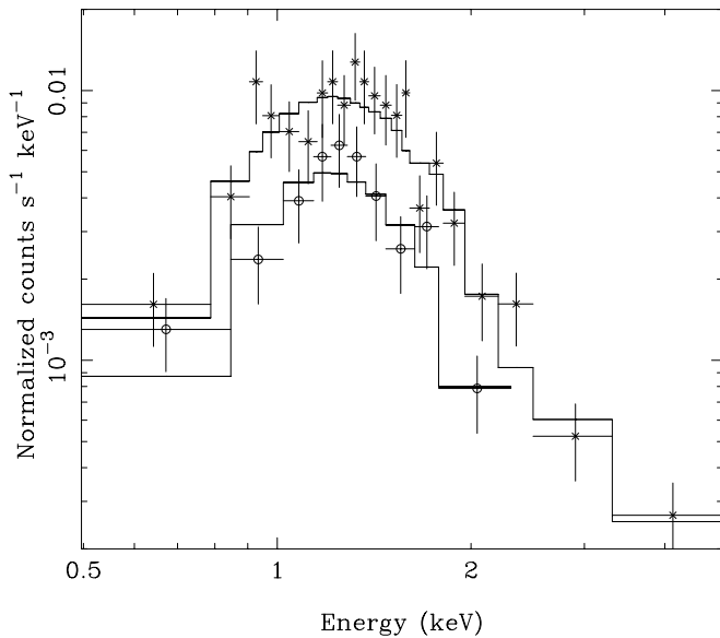
FIG. 3.—X-ray spectra of the X-ray transient neutron star in NGC 6440 during observation 1 ( crosses ) and observation 2 ( circles ). The solid lines through the data points are the best-fitting models to the data. [See the electronic edition of the Journal for a color version of this figure.]
