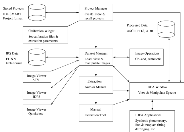
FIG. 1.—SMART flowchart.
