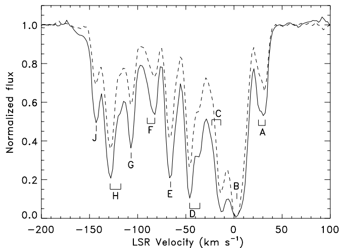
FIG. 1.—Line profiles of the Na D1 ( dashed ) and Na D2 ( solid ) lines. Spectra have been normalized, but no offset is applied between the lines. Labels denote distinct components, with vertical tick marks indicating the components fitted in Table 1. Some of these (e.g., D) appear to be further unresolved multiples.
