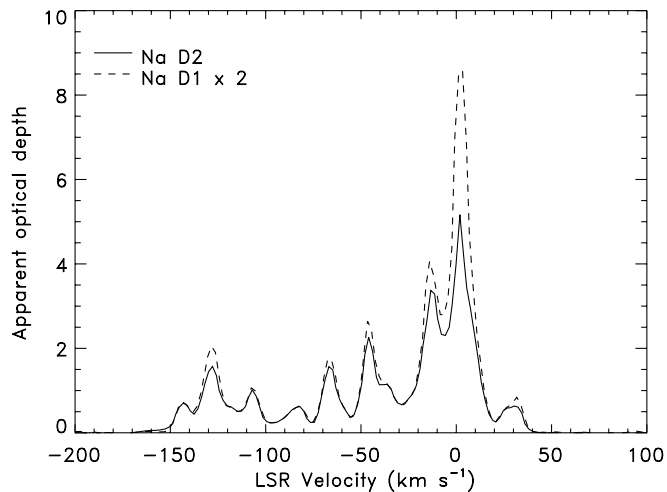
FIG. 2.—Apparent optical depths of the Na D lines. The D1 optical depths have been doubled so that they are identical to D2 in the optically thin limit. Where the lines disagree, saturation is important and the optical depth may be underestimated.
