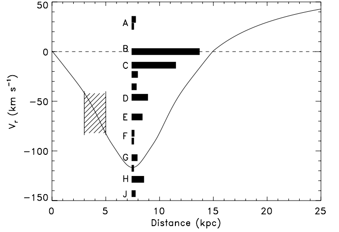
FIG. 4.—Expected relation between radial velocity and distance along the line of sight to GX 339–4. The curve uses the rotation curve adopted by Nakanishi & Sofue (2003). Each horizontal bar represents one of the fitted components of Na D absorption. The vertical position indicates the fitted velocity, and the length of the bar is proportional to the column density. The horizontal positions are arbitrary. The hatched region indicates the distance range favored by Zdziarski et al. (1998).
