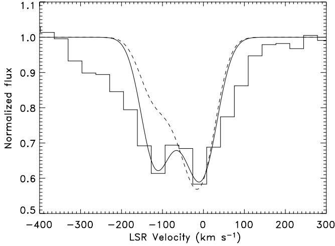
FIG. 3.—Line profile of the Ca II K line. Histograms show the data, which are at much lower resolution than that of the Na D lines. The dashed line shows a “blind” prediction of the line profile based on the Na D fits, assuming that no velocity correction is needed, that the intrinsic component widths are thermal, and that the ratio of Ca II to Na I is 0.6, appropriate for inner Galactic center lines of sight (Sembach & Danks 1994). The solid line is a better fit, including a small velocity offset and allowing the abundance of the G–J complex to differ from the rest of the components. See the text for more details.
