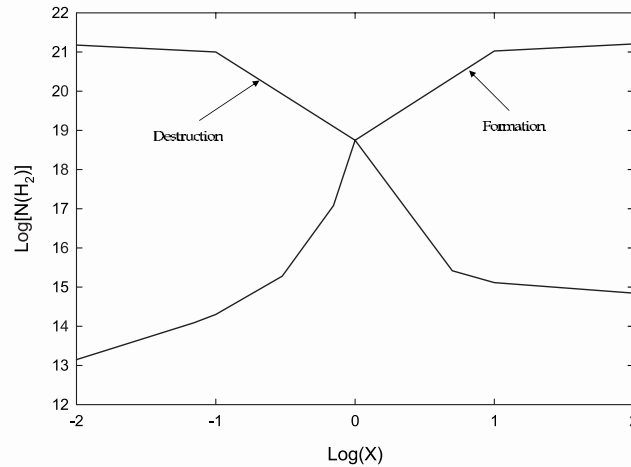
FIG. 11.—Predicted \text{H}_2 column density ( \text{cm}^{-2} ) as a function of the dissociation and formation rate scaling factor X . This plot clearly illustrates the sensitivity of the \text{H}_2 column density to the various rates. Changes in either rate of an order of magnitude can cause changes to the \text{H}_2 column density of up to 6 orders of magnitude. In order to have confidence in predicting the \text{H}_2 column density, one must model the \text{H}_2 formation and destruction processes as accurately as possible, without resorting to approximations.
