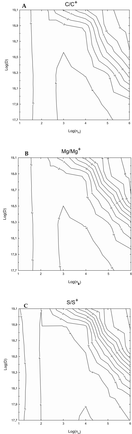
FIG. 3.—Log of the ratio of atomic to ionized (a) C, (b) Mg, and (c) S, which correspond to the column densities measured in more than one stage of ionization by SS97. The observed 1\sigma ratios of C ( >-4.35 ), Mg ( -3.4 \pm 0.5 ), and S ( -4.2 \pm 1.0 ) agree with most of our calculations. In this and all subsequent contour plots, the parameter n_{\text{H}} = n(\text{H}^+) + n(\text{H}^0) + 2n(\text{H}_2) ( \text{cm}^{-3} ), the total hydrogen density in all forms.
