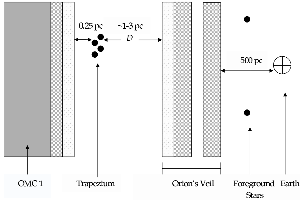
FIG. 2.—Geometry of the central regions of the Orion Nebula and the veil. For this figure, solid regions correspond to H_2 , checked regions to H^0 , and dotted regions to H^+ . Starting with the side of the veil facing the Trapezium, we have a small H^+ zone followed by a PDR. Because of the strong UV flux coming from the Trapezium cluster, H_2 never readily forms, but instead we have a thick region of atomic hydrogen. The segmented regions in the veil represent the multiple components seen in the 21 cm optical depth profile in Fig. 1. The distance D represents the distance from the side of the veil facing the Trapezium to the Trapezium itself and is the same distance used in all subsequent contour plots. [See the electronic edition of the Journal for a color version of this figure.]
