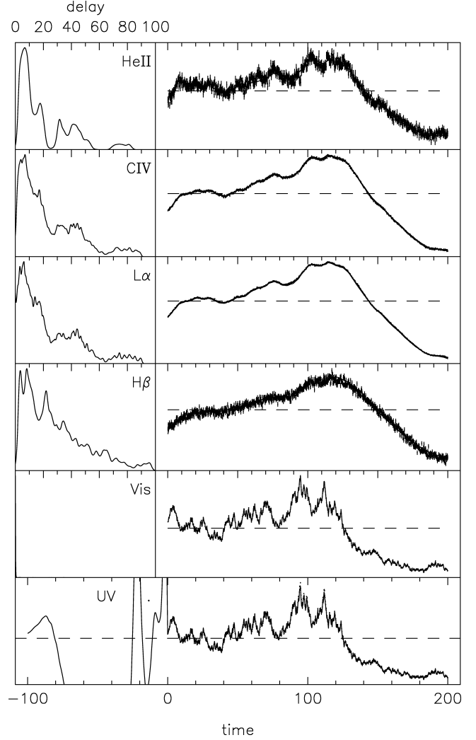
FIG. 6.—Continuum and velocity-integrated emission line fluxes measured from simulated Kronos spectra, representing 1 hr integrations every 0.2 days for 200 days. The driving continuum light curve F_c(t) is in the bottom panel, the responding line light curves F_i(t) above, and the recovered delay maps \Psi_i(\tau) are shown in the left-hand column.
