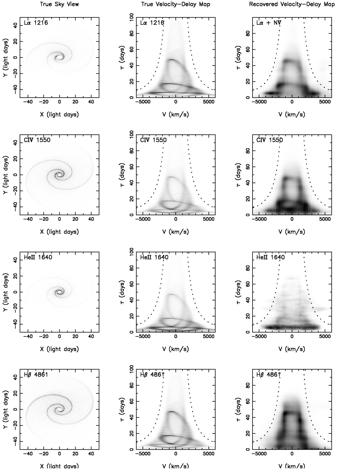
FIG. 7.—Recovery of velocity-delay maps from simulated Kronos data sets. The left column shows “sky views” of the adopted BLR model, in this case a Keplerian accretion disk with two spiral arms, in the light of four different emission lines. The middle column shows the corresponding theoretical velocity-delay maps, in which the spiral arms are also clearly visible. The right column gives the “observed” velocity-delay maps recovered from simulated Kronos data representing 1 hr exposures every 0.2 days for 200 days.
