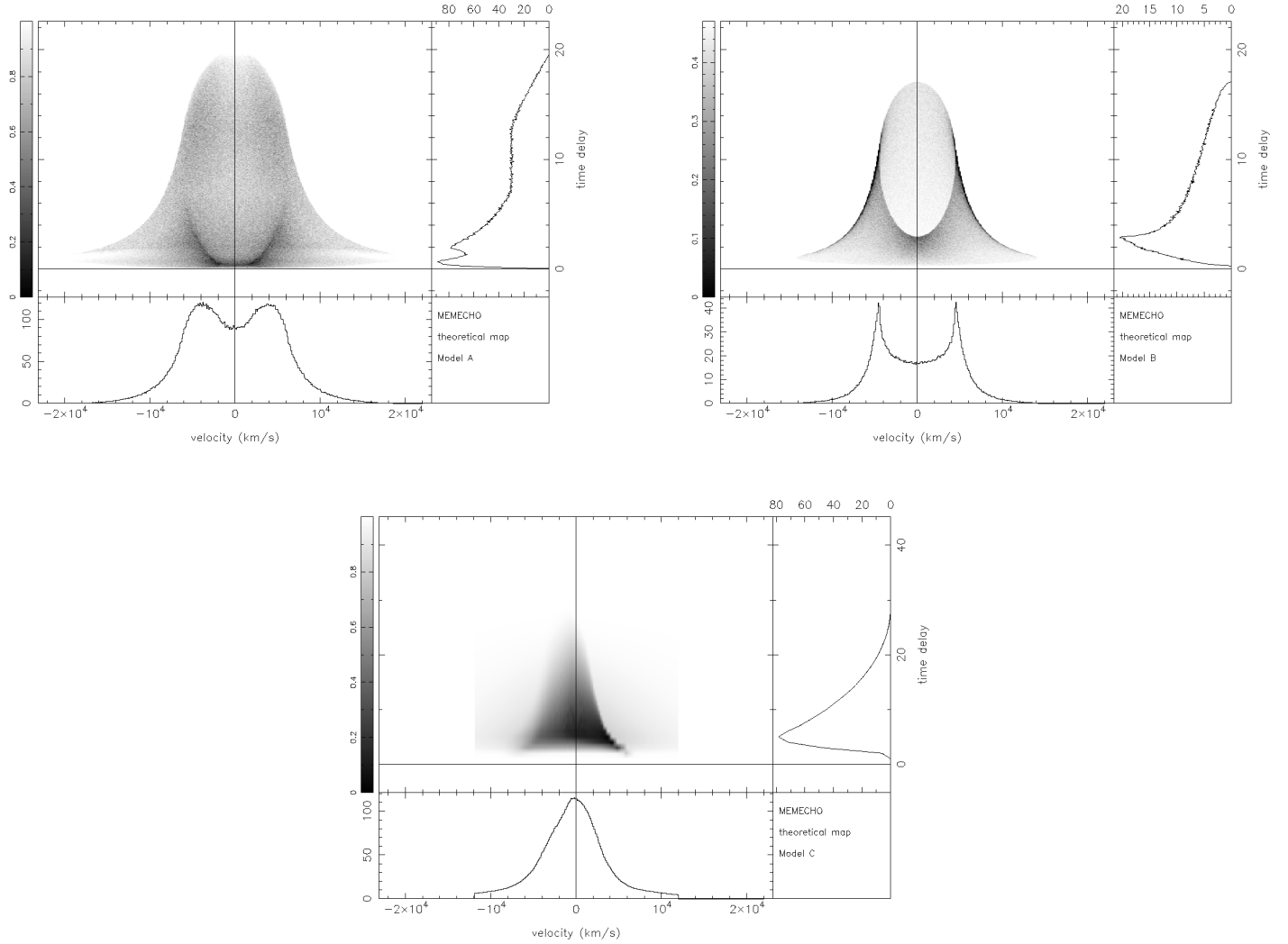
FIG. 1.—Theoretical velocity-delay maps \Psi_i(v, \tau) for (a) a spherical distribution of line-emitting clouds in circular Keplerian orbits of random inclination, illuminated by an anisotropic continuum source (Wanders et al. 1995; Goad & Wanders 1996); (b) a flat Keplerian disk of clouds; and (c) a hydromagnetically driven wind (Bottorff et al. 1997). Projections \Psi_i(v) and \Psi_i(\tau) are shown below and to the right, respectively, of each gray-scale \Psi_i(v, \tau) map.
