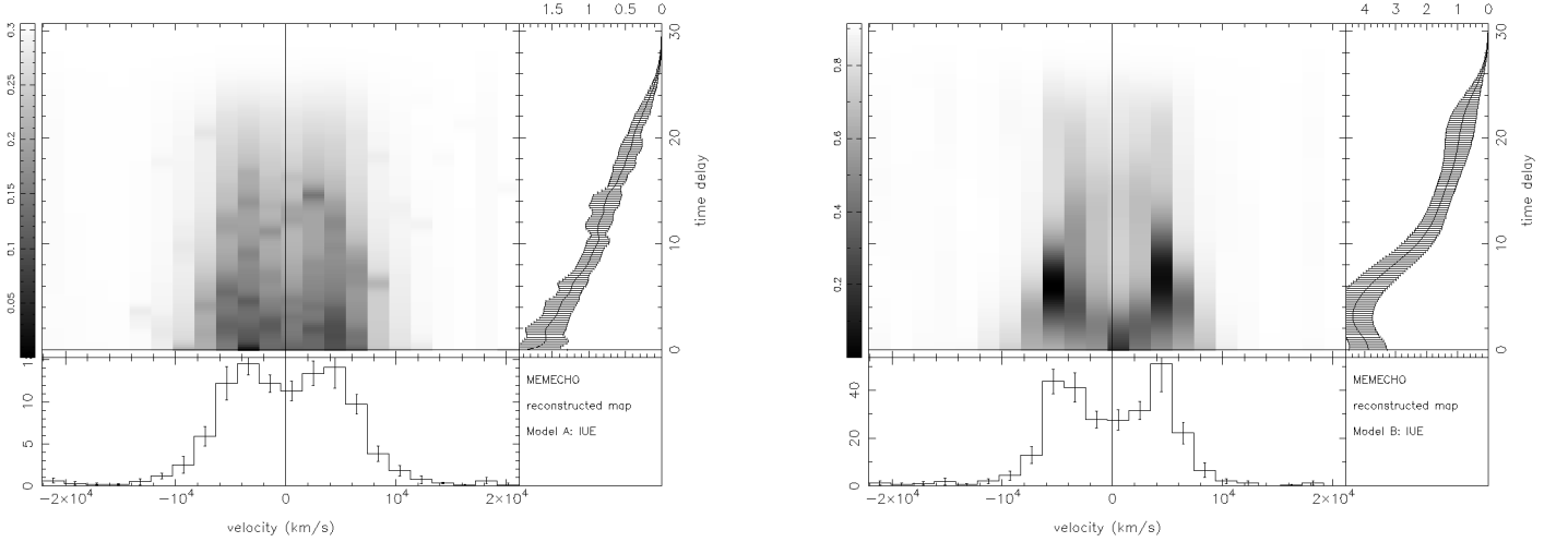
FIG. 3.—Observed velocity-delay maps \Psi(v, \tau) recovered from simulated data with characteristics similar to continuous IUE monitoring; specifically, T_{\text{dur}} = 49 days, \Delta t = 0.2 days, continuum and emission-line flux uncertainties of 3% and 7%, respectively, spectral resolution of \sim 8 \text{ \AA} , and continuum variations normalized to an amplitude of 12% on timescales of 10 days. The two cases shown, as in Fig. 1, are (a) a spherical distribution of line-emitting clouds in circular Keplerian orbits of random inclination, illuminated by an anisotropic continuum source (Wanders et al. 1995; Goad & Wanders 1996), and (b) a flat Keplerian disk of clouds. Projections \Psi(v) and \Psi(\tau) , with Monte Carlo error bars, are shown below and to the right, respectively, of each gray-scale \Psi(v, \tau) map.
