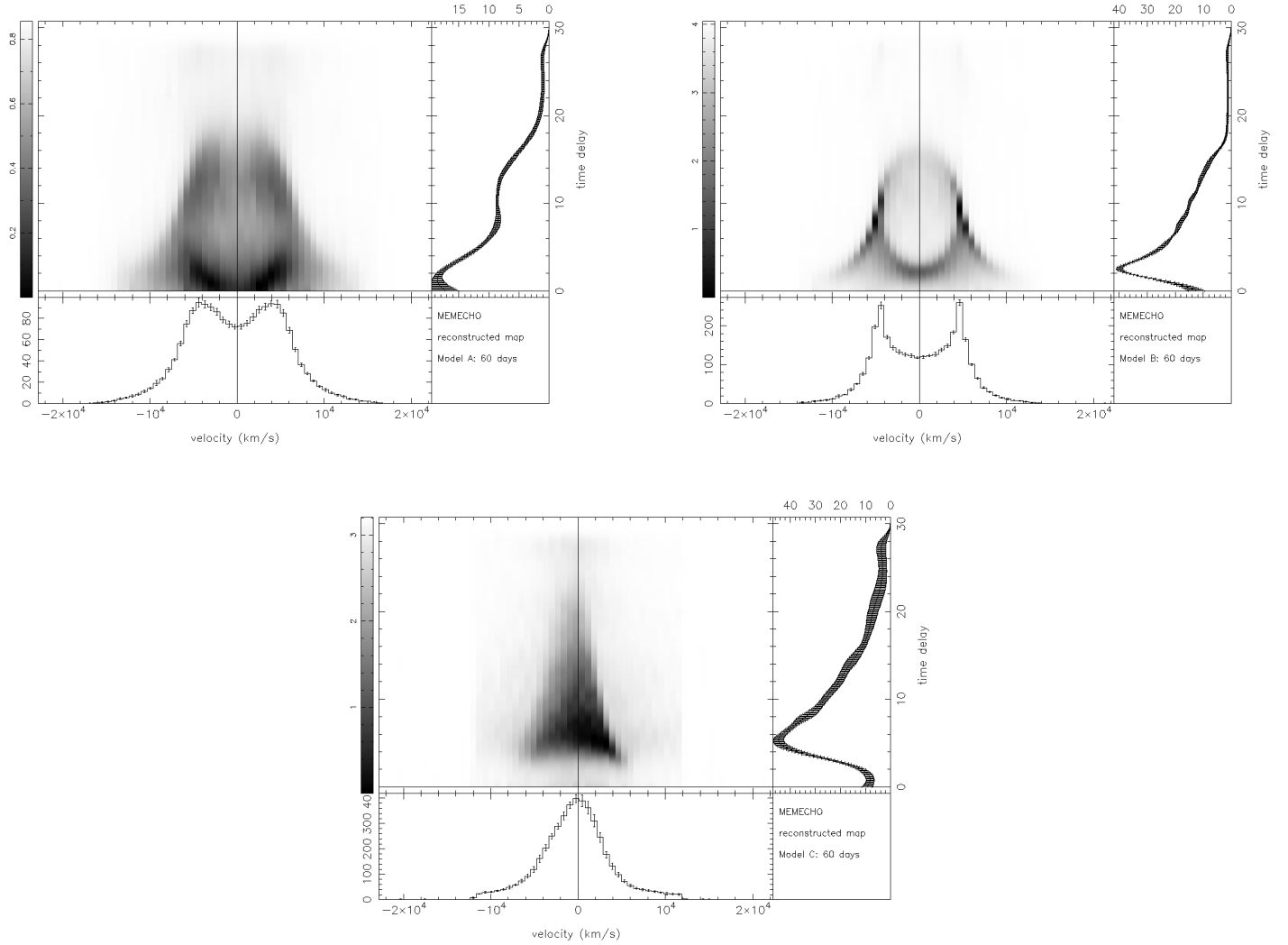
FIG. 2.—Observed velocity-delay maps \Psi(v, \tau) recovered from a simulation with duration T_{\text{dur}} = 60 days and time resolution \Delta t = 0.1 day (i.e., at total of \sim 600 observations). As in Fig. 1, the three cases shown are for (a) a spherical distribution of line-emitting clouds in circular Keplerian orbits of random inclination, illuminated by an anisotropic continuum source (Wanders et al. 1995; Goad & Wanders 1996); (b) a flat Keplerian disk of clouds; and (c) a hydromagnetically driven wind (Bottorff et al. 1997). Projections \Psi(v) and \Psi(\tau) , with Monte Carlo error bars, are shown below and to the right, respectively, of each gray-scale \Psi(v, \tau) map.
