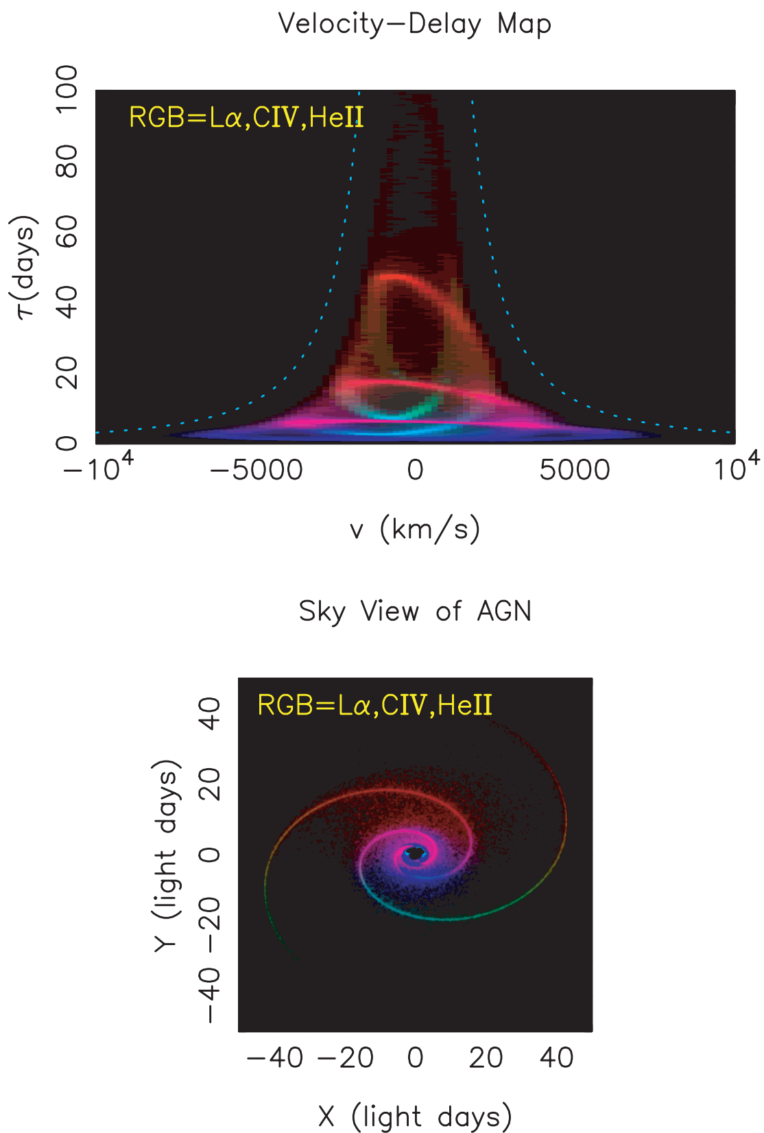
FIG. 4.—Velocity-delay map ( top ) and corresponding sky view ( bottom ) for a Keplerian accretion disk with two spiral arms. Red, green, and blue correspond to the \text{Ly}\alpha , \text{C IV} , and \text{He II} emission lines, respectively.
