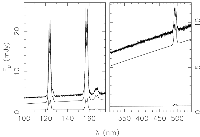
FIG. 5.—Synthetic Kronos spectra for NGC 5548. Top spectrum is a single 1 hr integration near peak brightness, below which are the mean and rms of 1001 such spectra representing 1 hr integrations every 0.2 days for 200 days. This simulation of reverberation in the environment of a 10^7 M_\odot black hole includes a Keplerian disk with spiral density waves, continuum variations, and responses in five key emission lines: \text{Ly}\alpha , N v \lambda 1240 , C IV \lambda 1549 , He II \lambda 1640 , and \text{H}\beta .
