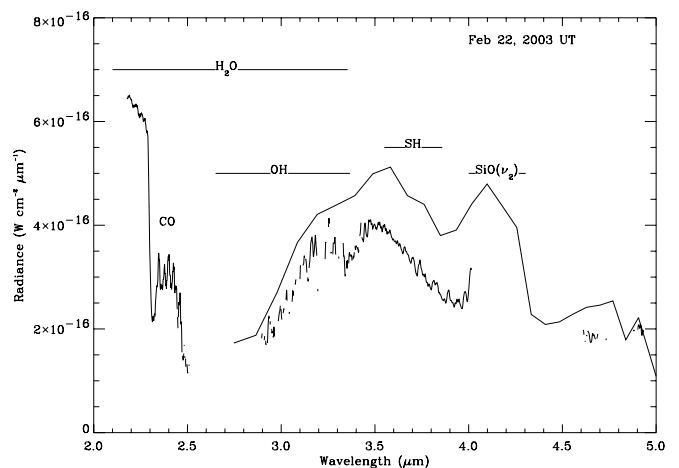
FIG. 8.—2003 February SpeX spectrum (lower curve). The upper curve shows the BASS spectrum taken about a month earlier. At short wavelengths, CO and H 2 O are responsible for the decrease longward of 2.3 \mu m. The very sharp turn up at 4 \mu m is the beginning of the SiO first-overtone band.
