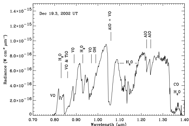
FIG. 6.—Late NIRIS spectrum from 0.81 to 1.33 \mu\text{m} . The spectrum is dominated by \text{H}_2\text{O} , CO, TiO, OH, VO, and AIO. The red-trending A-X(4, 0) doublet of AIO at 1.225 and 1.244 \mu\text{m} is particularly diagnostic. A number of weaker bands—presumably molecular—are present but are either not readily identifiable or sufficiently broad that they lack discrete features, e.g., OH, HS, and \text{H}_2\text{S} .
