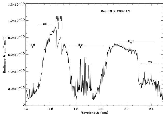
FIG. 7.—Late NIRIS spectrum from 1.4 to 2.5 \mu\text{m} . The spectrum is dominated by \text{H}_2\text{O} and CO. The red-trending A-X(2, 0) doublet of AIO at 1.650 and 1.687 \mu\text{m} is particularly diagnostic. A number of weaker bands—presumably molecular—are present but are either not readily identifiable or sufficiently broad that they lack discrete features, e.g., OH and HS.
