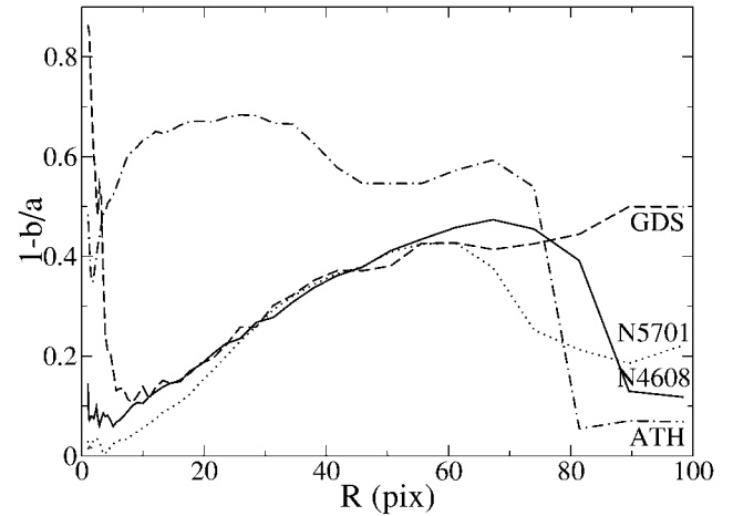
FIG. 3.—Ellipticity radial profiles for NGC 4608 and NGC 5701, as well as for both the GDS and the ATH models.
