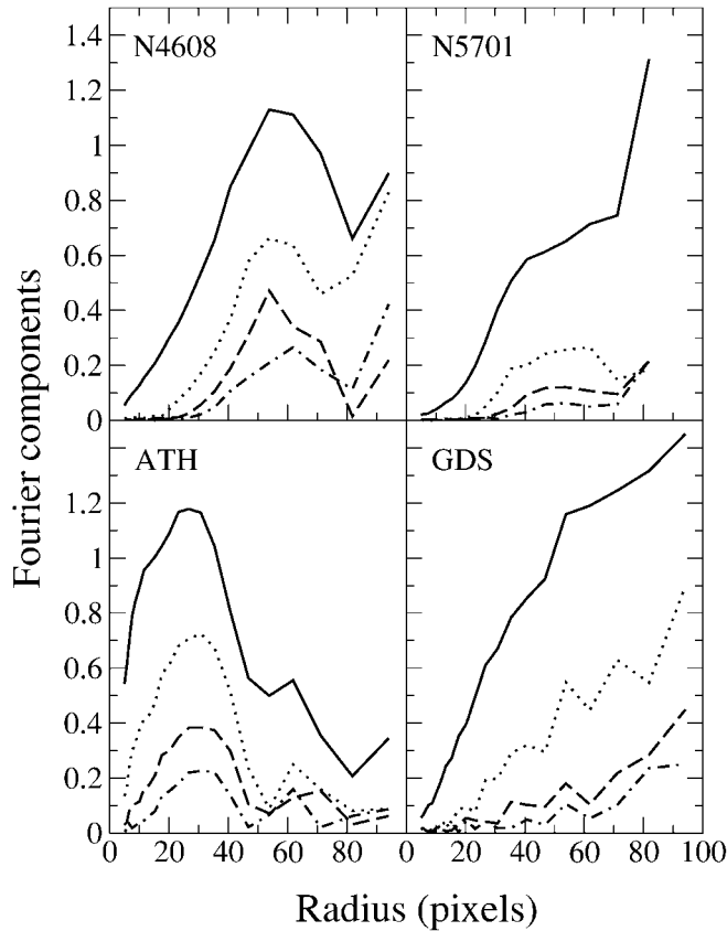
FIG. 5.—Radial profiles of the Fourier components of the observed galaxies and the models. The solid line refers to m = 2 , while the dotted line refers to m = 4 , the dashed line to m = 6 , and the dash-dotted line to m = 8 .
