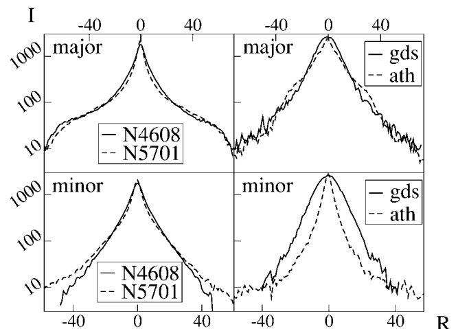
FIG. 4.—Intensity profiles along the major and minor axes of the observed galaxies and the models.
