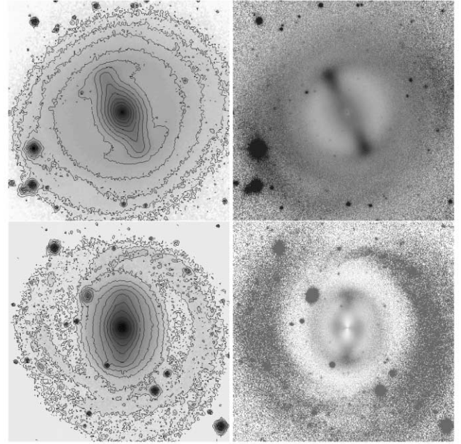
FIG. 1.—Results from the structural analysis. Top panels refer to NGC 4608, while bottom panels refer to NGC 5701. At left we present direct R images with an isophotal map. At right we show residual images after the subtraction of a bulge model only. Note the absence of a disk.
