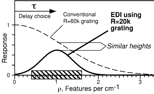
FIG. 11.—The interferometer shifts the grating response to higher \rho by \Delta\rho = \tau . The EDI response using R = 20,000 is comparable to that of the R = 60,000 grating (dashed curve) in the important \rho \sim 1 cm region. The photon S/N is proportional to the altitude of the curves.
