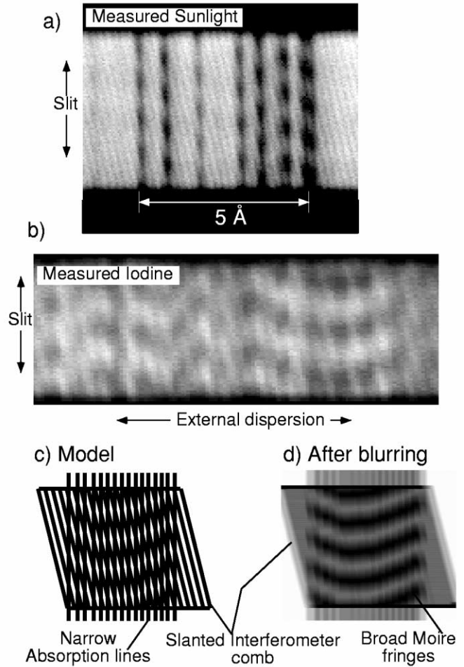
FIG. 5.—(a, b) Snippets of measured solar and iodine fringing spectra taken by the EDI prototype. The full bandwidth was 130 Å. The external spectrograph resolution was sufficiently high ( R \sim 20,000 ) to partially resolve the underlying phase-slanted interferometer comb. (c, d) Graphical models explaining formation of “smilelike” moiré pattern seen in iodine data. The high detail spectral features are heterodyned to lower details where they can survive the blurring of the external spectrograph.
