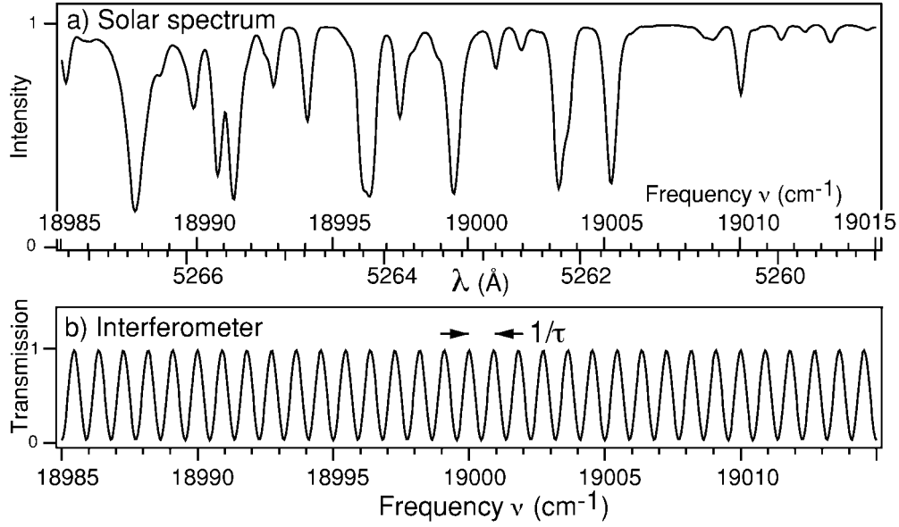
FIG. 4.—(a) Section of the solar spectrum vs. frequency ( \nu = 1/\lambda , in units of cm -1 ) or wavelength ( \lambda ). (b) Sinusoidal transmission function of Michelson interferometer having delay \tau = 1.1 cm, for one output arm. This is periodic when plotted vs. \nu , making \nu the natural dispersion variable. This value of \tau yields an interferometer comb peak spacing similar to the typical absorption line width.
