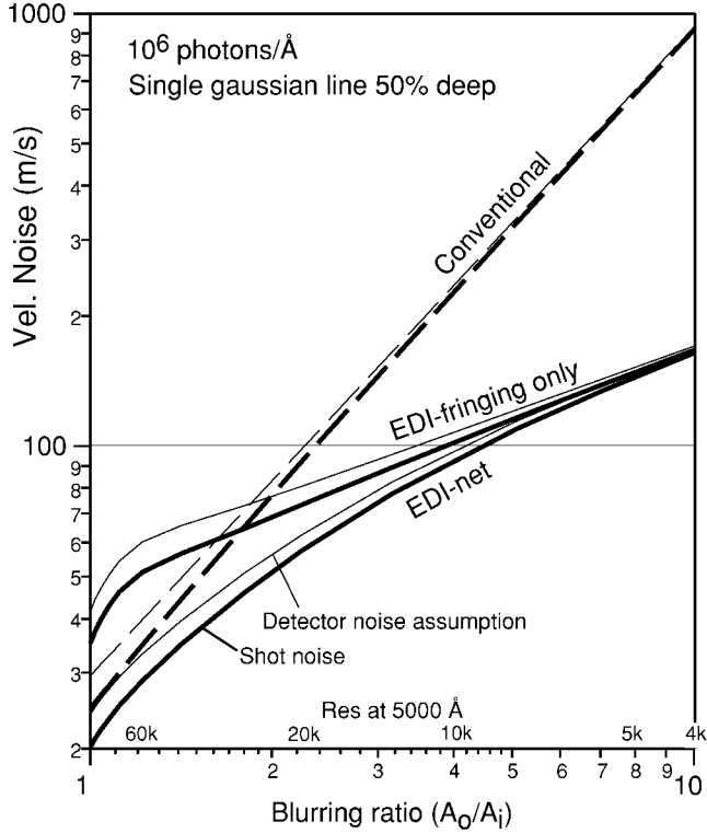
FIG. 8.—Calculated velocity noise for a single Gaussian line receiving 10^6 photons \text{\AA}^{-1} at 5000 \text{ \AA} in the continuum, for conventional and EDI spectroscopies. The thin curves assume constant noise set by continuum flux. The thick curves assume noise varying as the square root of local intensity. The EDI-net curve includes both fringing and nonfringing components. Both interferometer outputs are used.
