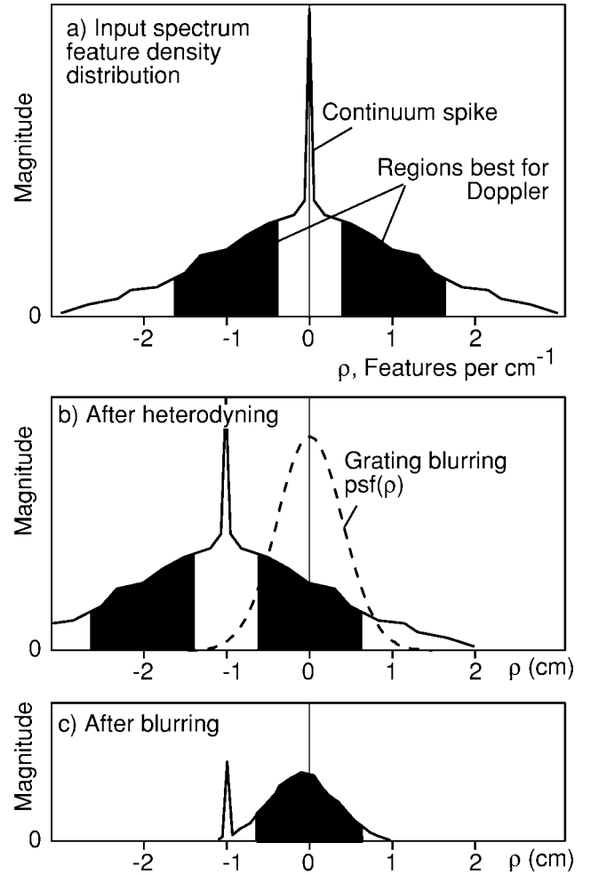
FIG. 10.—Stages in heterodyning process, in Fourier space. (a) Input s_o(\rho) . The regions near \rho \sim \pm 1 cm hold the most Doppler information and are blackened for labeling. (b) After passage through the interferometer, s_o(\rho) shifts by \Delta\rho = \tau . This places a blackened regions near the origin where it better survives the grating blurring psf ( \rho ) (dashed curve). (c) The data near the origin expresses the moiré fringe. The continuum spike remnant, now shifted to \rho \sim -1 cm, corresponds to the sinusoidal comb faintly seen in the CCD data (Figs. 5a and 5b).
